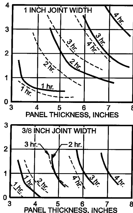
FIGURE 721.2.1.3.1 CERAMIC FIBER JOINT PROTECTION
