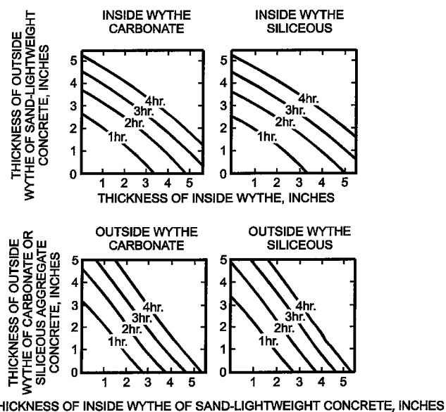
FIGURE 721.2.1.2 FIRE-RESISTANCE RATINGS OF TWO-WYTHE CONCRETE WALLS
