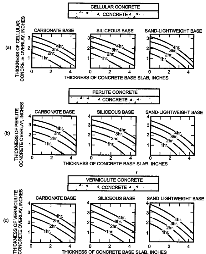
FIGURE 721.2.2.3(1) FIRE-RESISTANCE RATINGS FOR CONCRETE ROOF ASSEMBLIES
