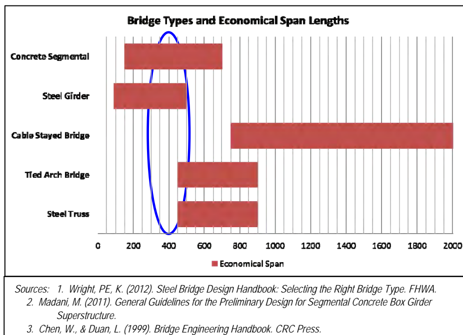
Figure 4-11 Bridge Types and Economical Span Lengths
