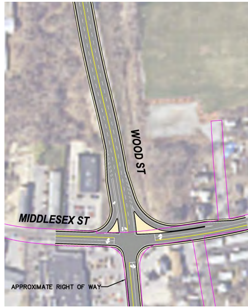
Figure 5-22 Rourke Bridge/Wood Street at Middlesex Street Concept 2
