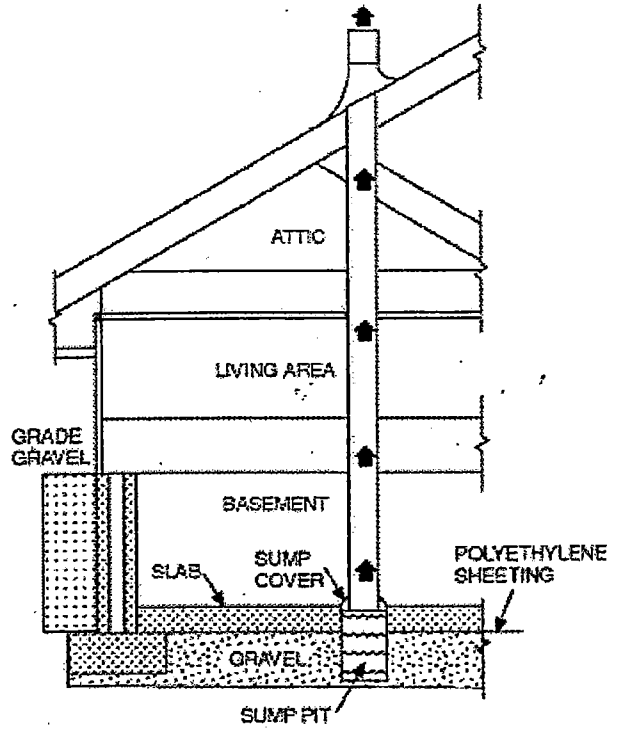
PASSIVE RADON SYSTEM VENTED THROUGH SUMP
