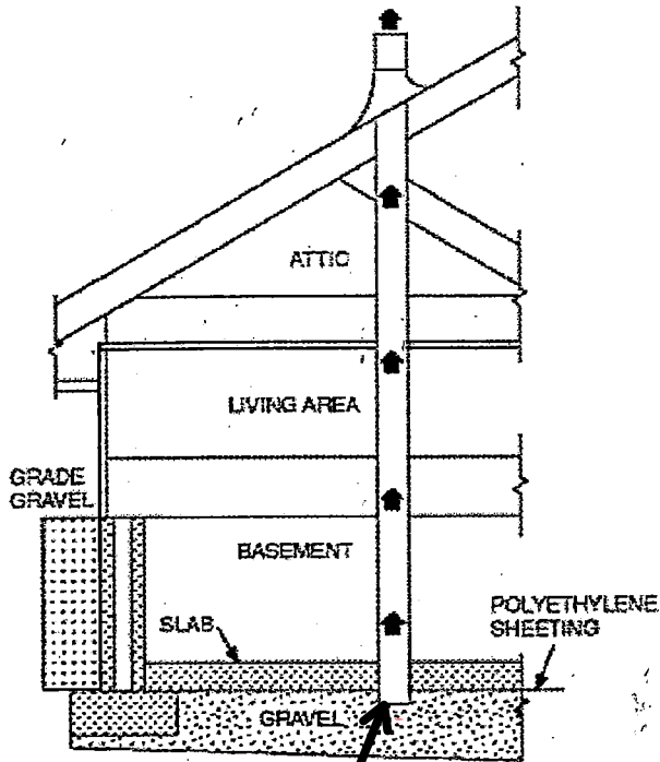
TYPICAL SUB-SLAB DEPRESSURIZATION PASSIVE RADON SYSTEM
