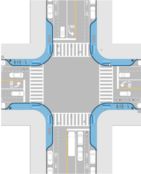
Figure 9. Curb extensions
