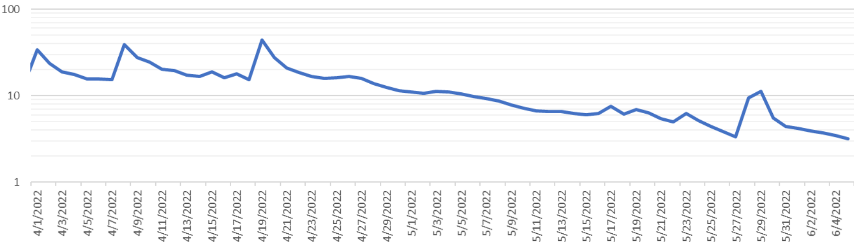
Browns Brook: daily mean streamflow, Apr - Jun 2022
