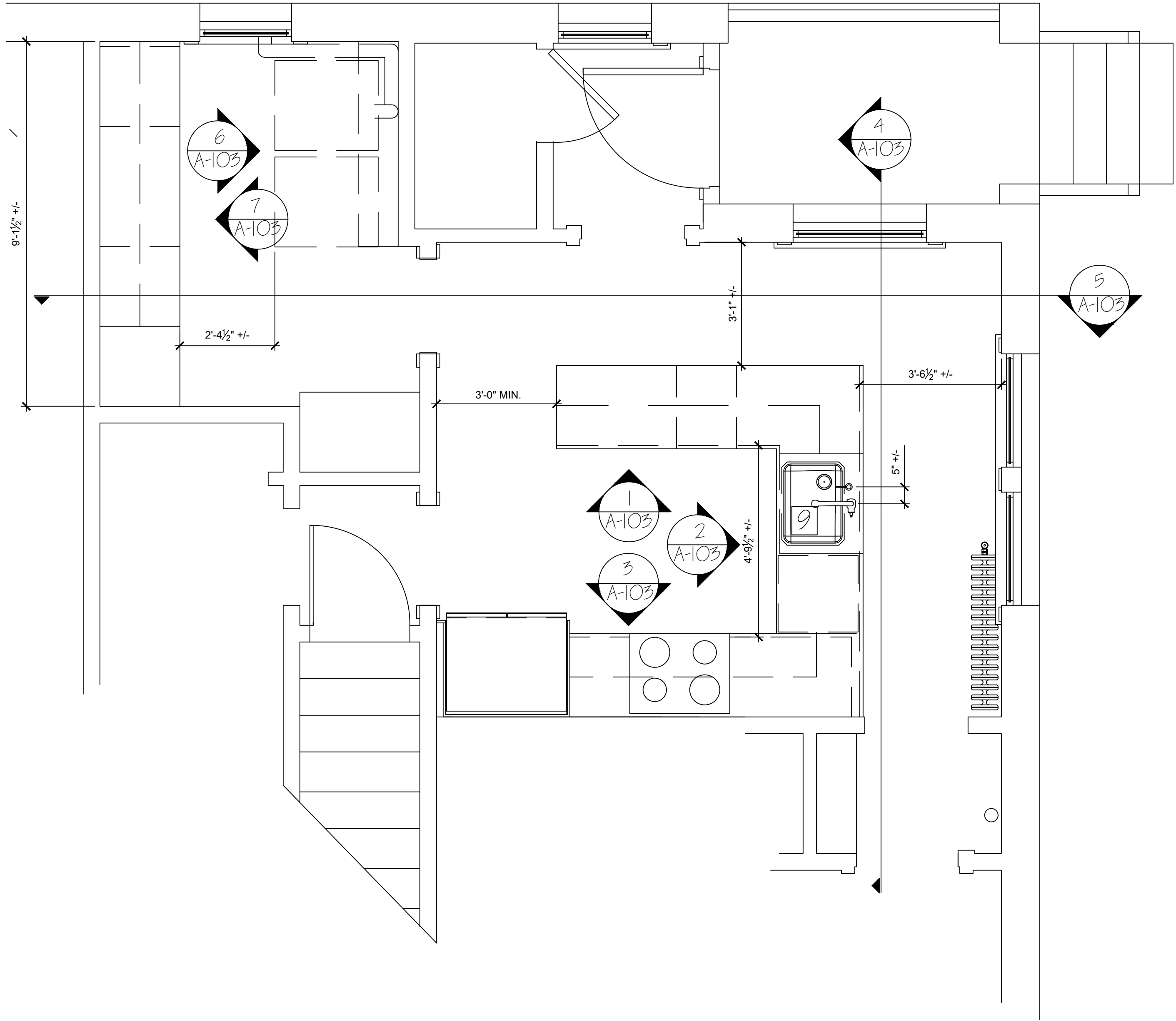
COTTAGE ONE KITCHEN FLOOR PLAN
