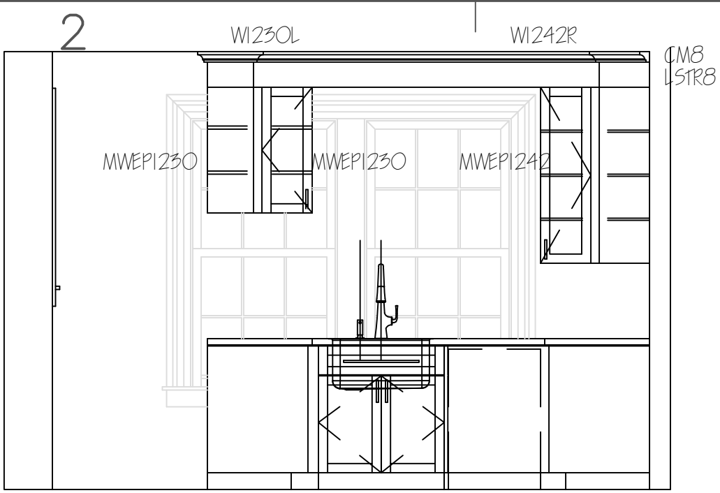
ELEVATION 2/ A-100
