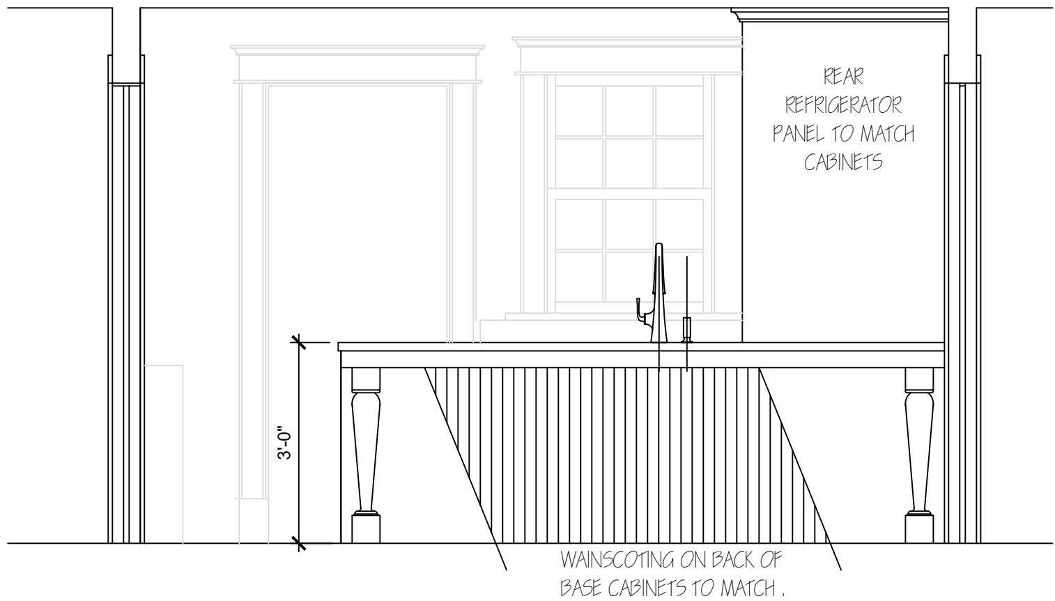
ELEVATION 4/ A-102
