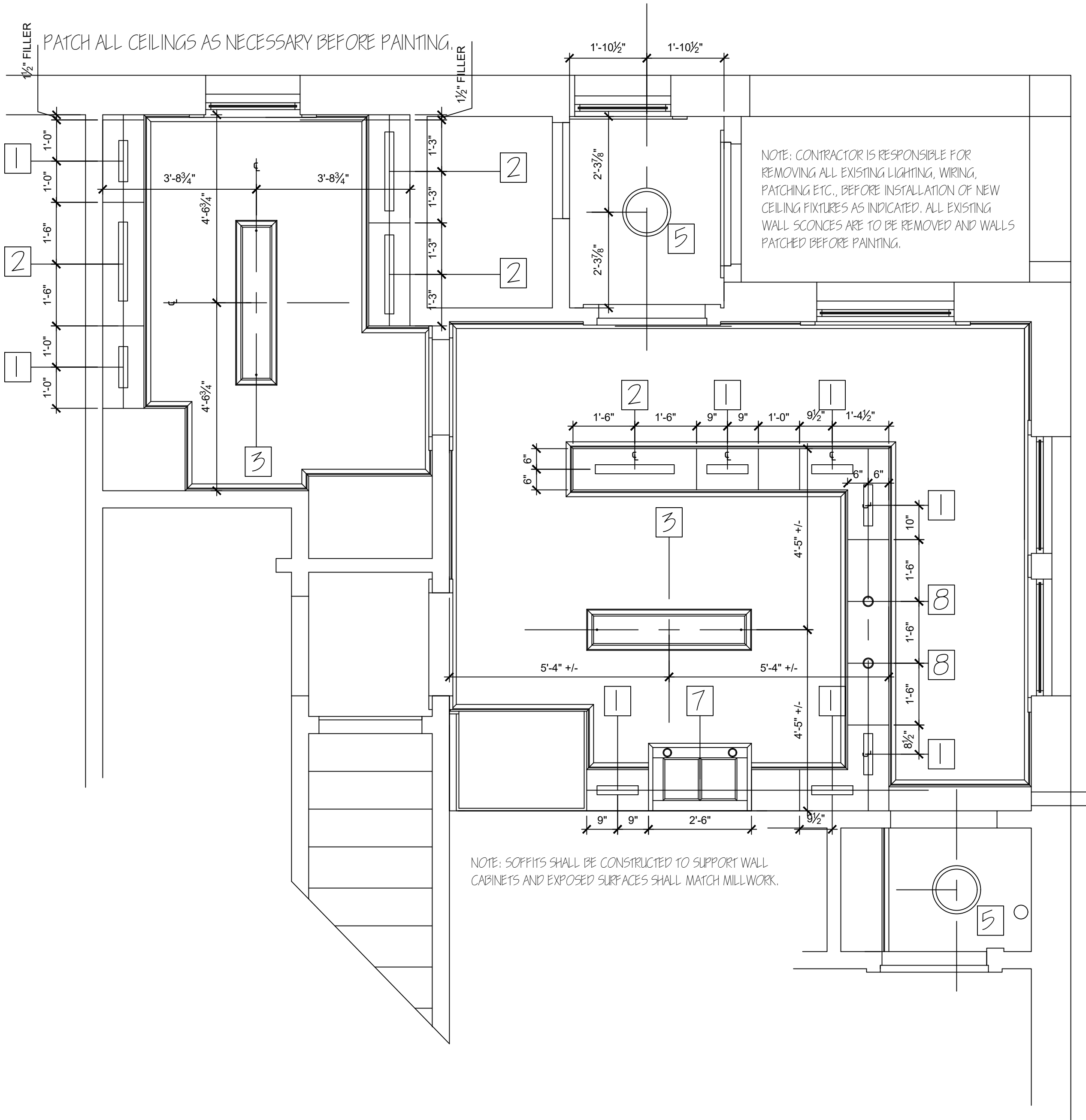
COTTAGE ONE KITCHEN REFLECTED CEILING PLAN
