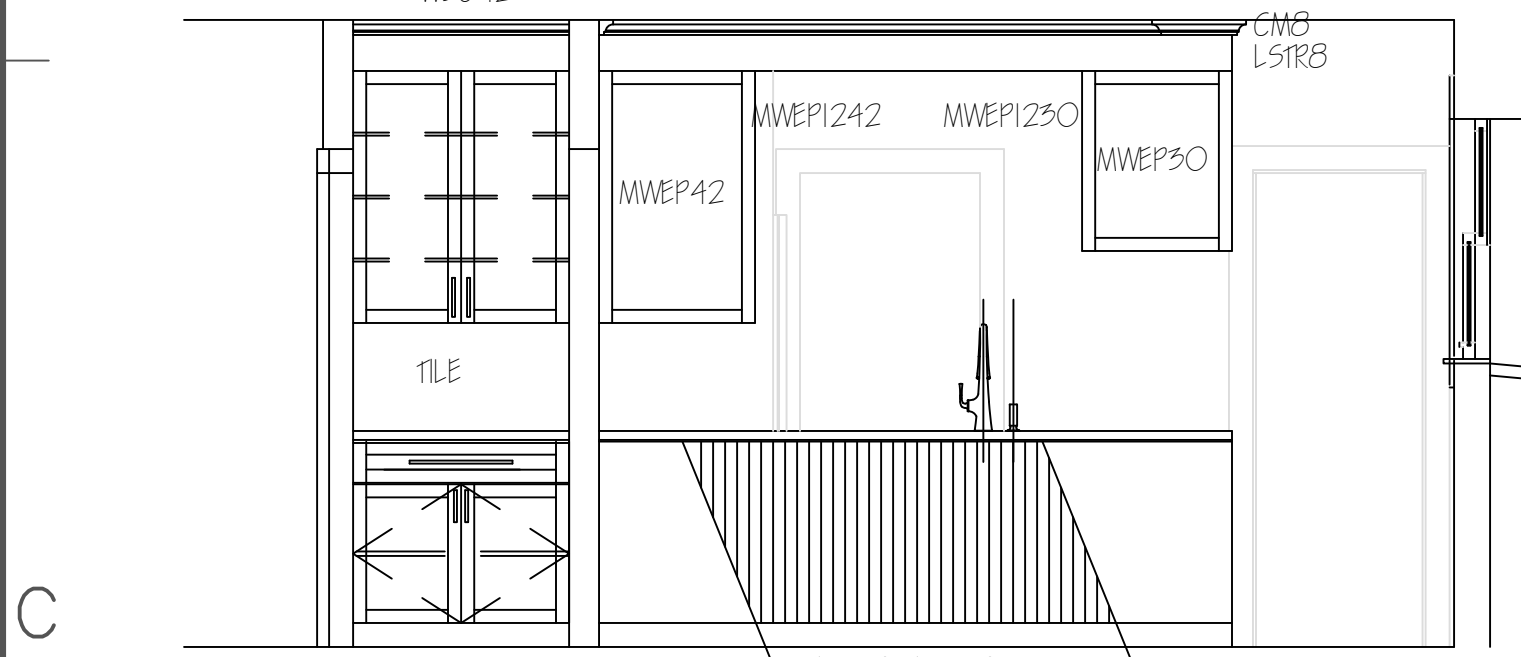
ELEVATION 4/ A-100
