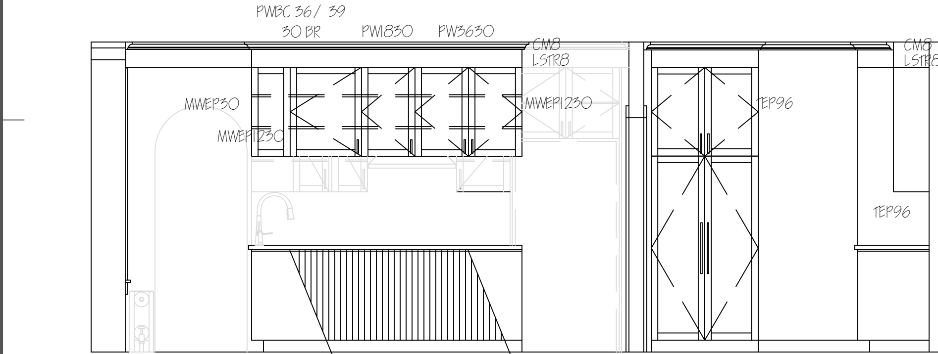
ELEVATION 5/ A-100
