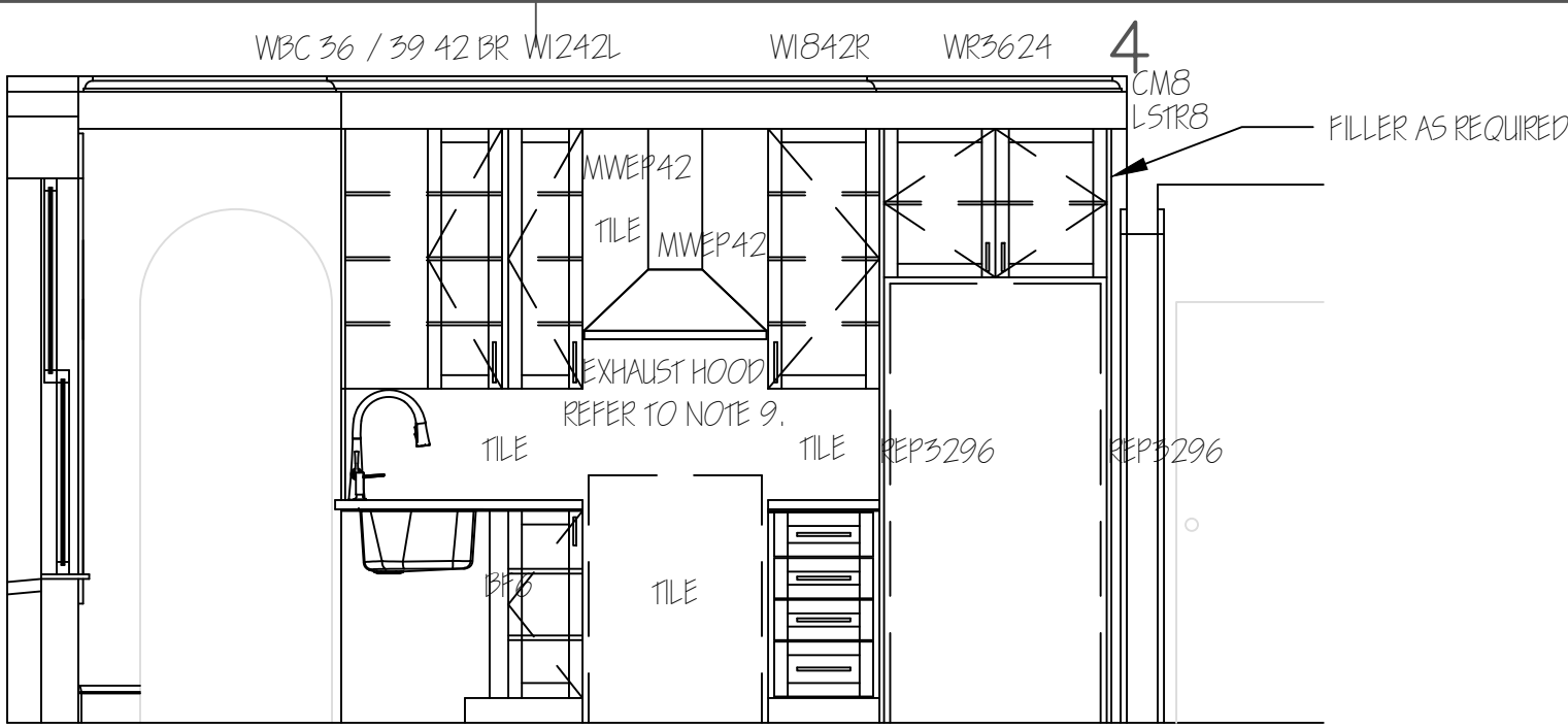
ELEVATION 3/ A-100
