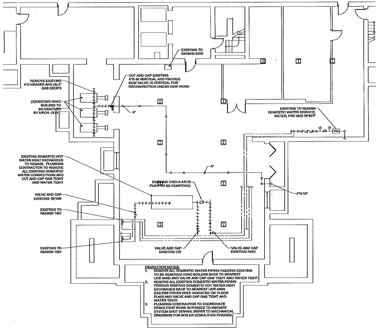
MECHANICAL ROOM DEMOLITION WORK PART PLAN
