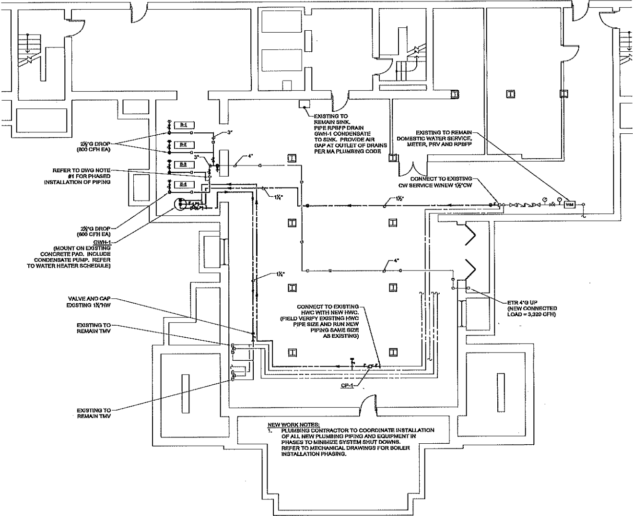
MECHANICAL ROOM NEW WORK PART PLAN
