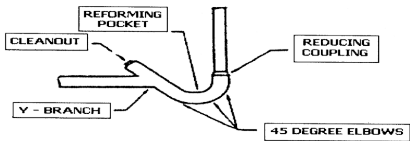
FIGURE F-5 HORIZONTAL TO VERTICAL LIFT CONNECTION
