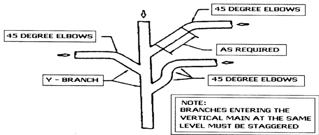
FIGURE F-6 HORIZONTAL TO VERTICAL DROP CONNECTION
