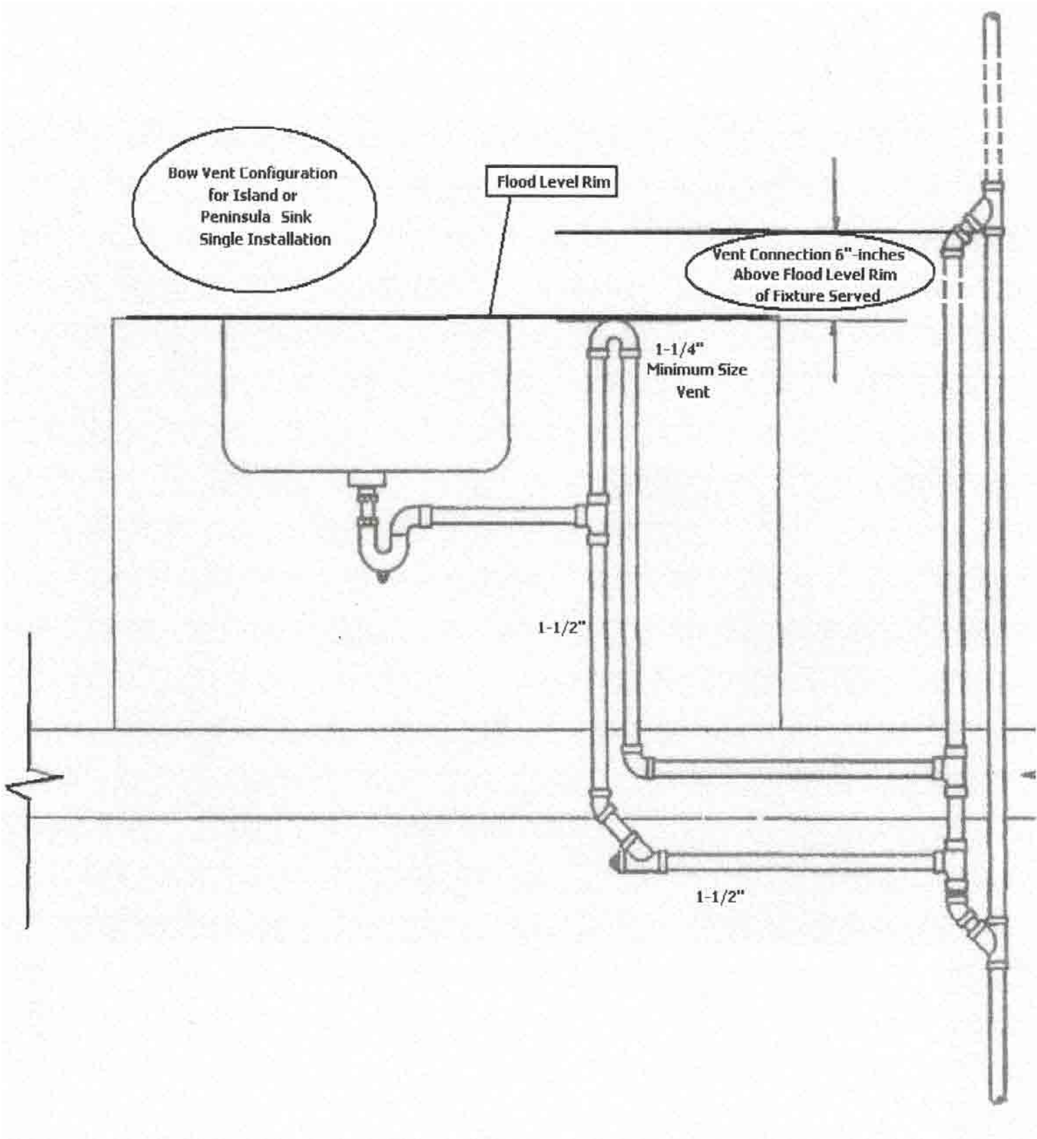
FIGURE 13A: Illustration of Bow Vent Single Installations.
