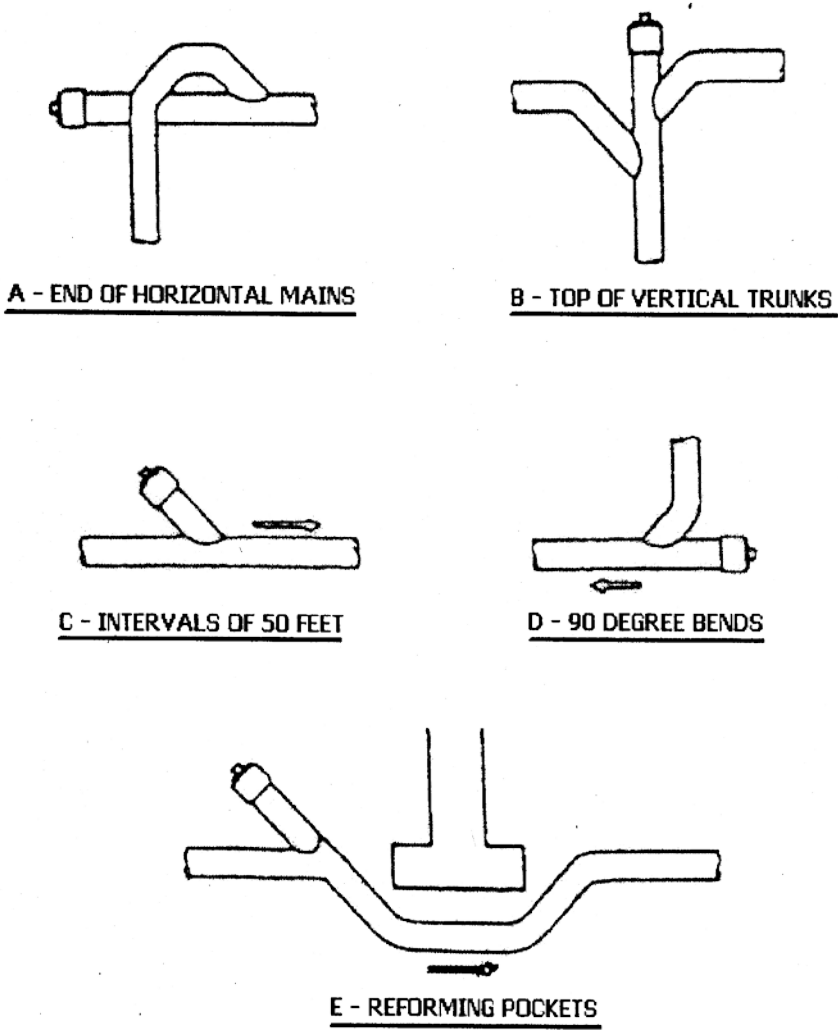
FIGURE F-10 TYPICAL CLEANOUT LOCATIONS
