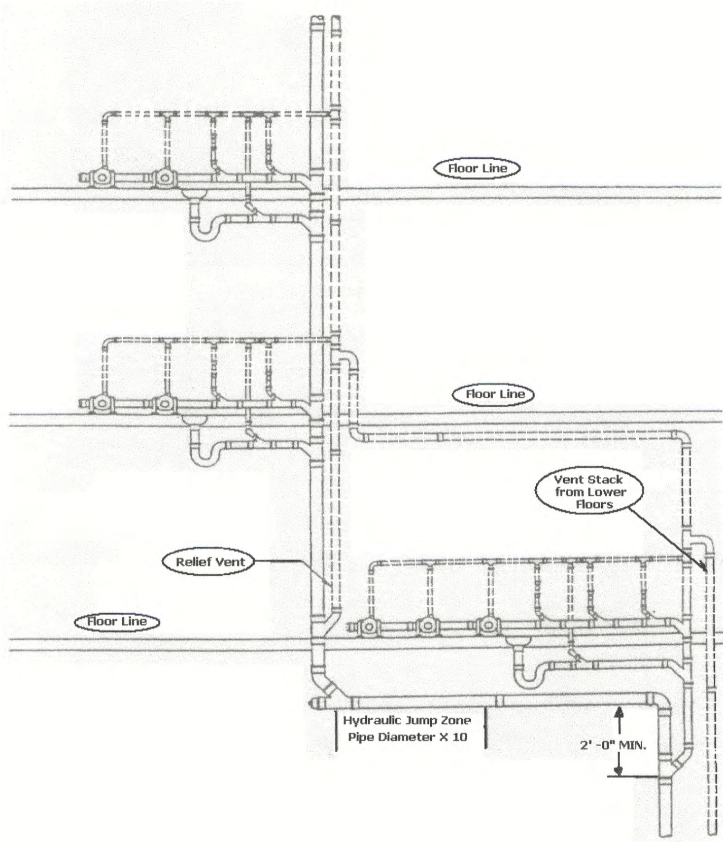
FIGURE 20: Illustration of Offsets of More than 45° in Buildings of Five Stories or More in Compliance with 248 CMR 10.15(8)(b) and 10.16(4)(c).
