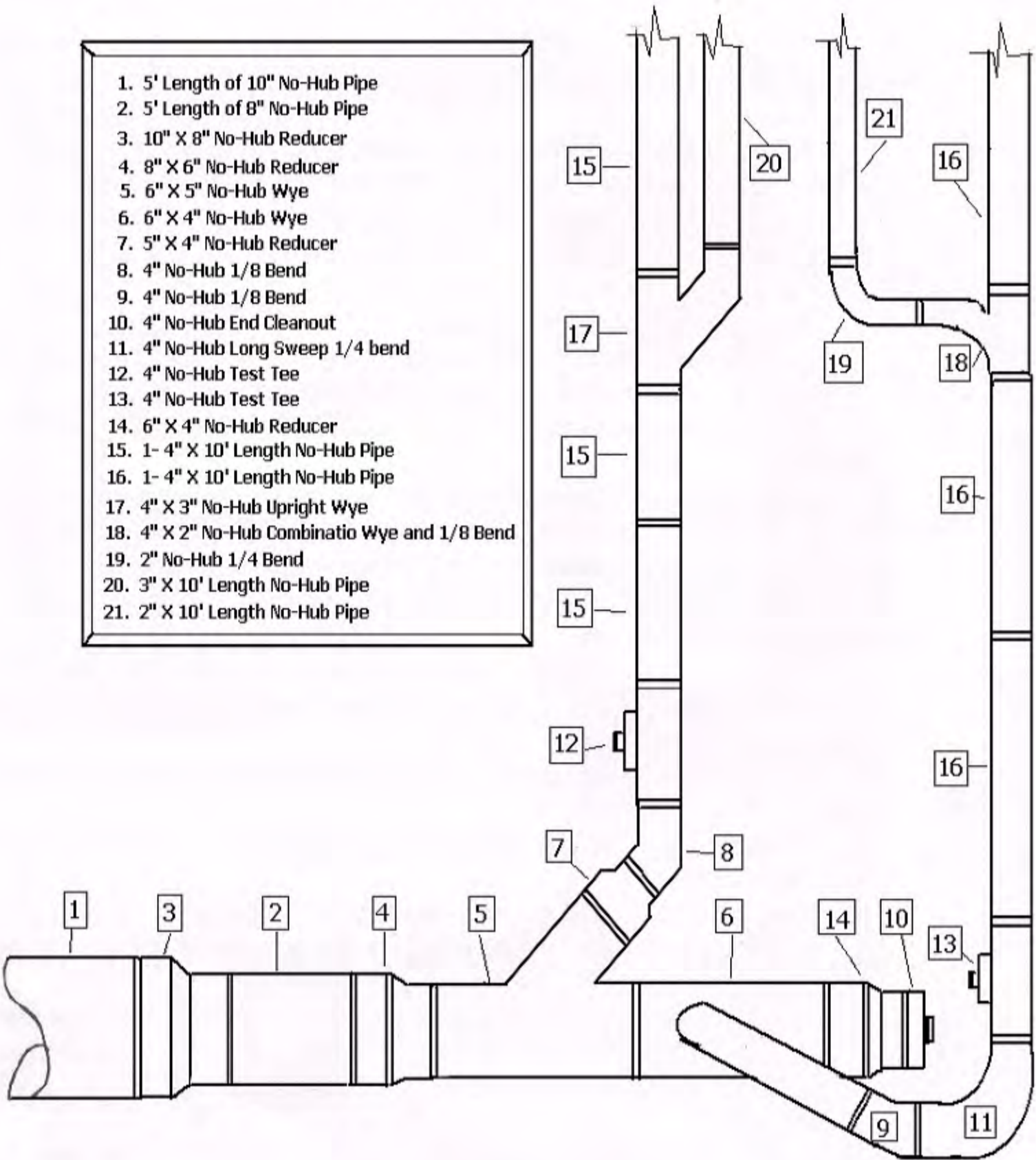
Figure 1 No-Hub Coupling Test Configuration Design
