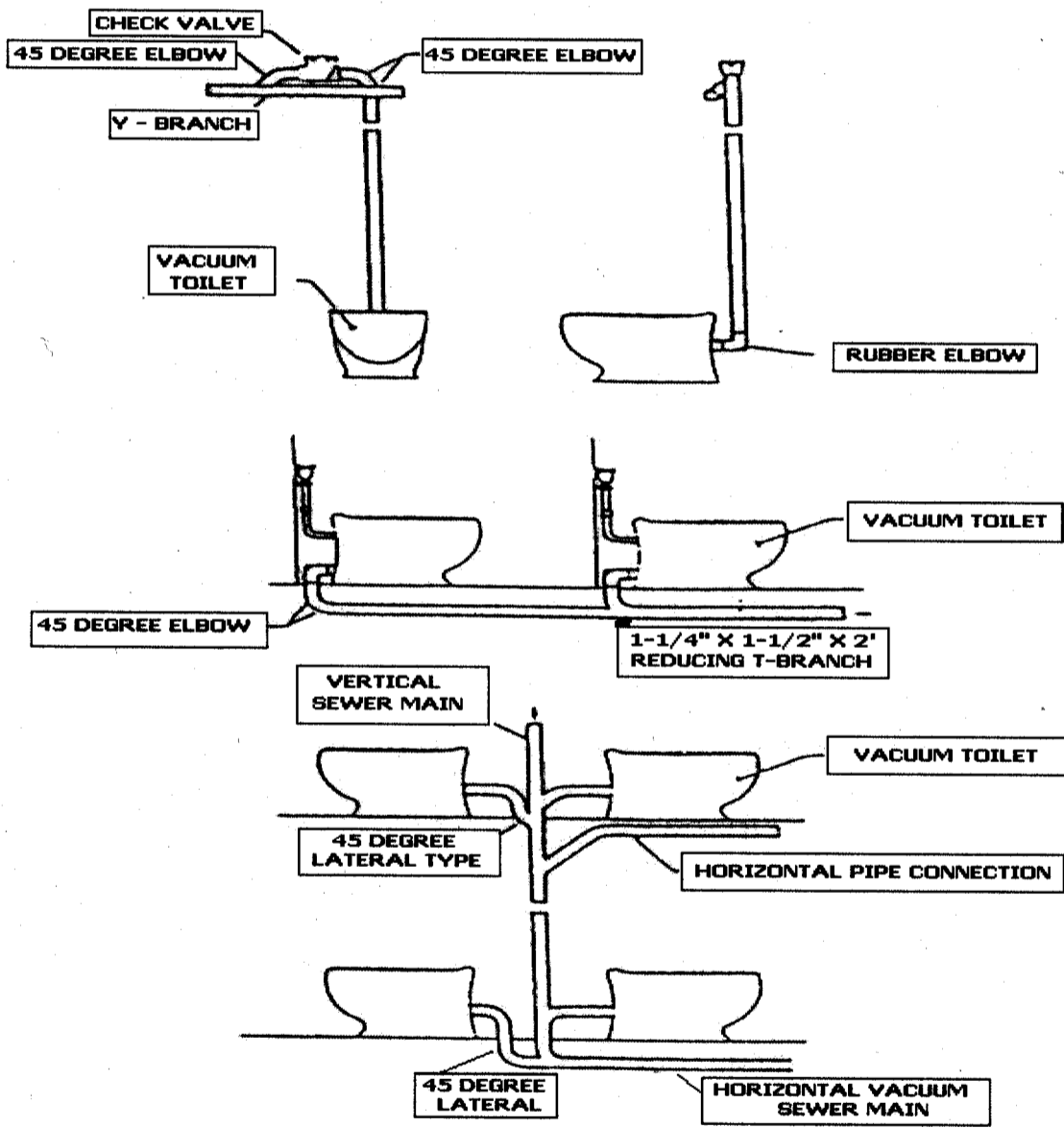
FIGURE F-9 TYPICAL VACUUM FIXTURE INSTALLATION
