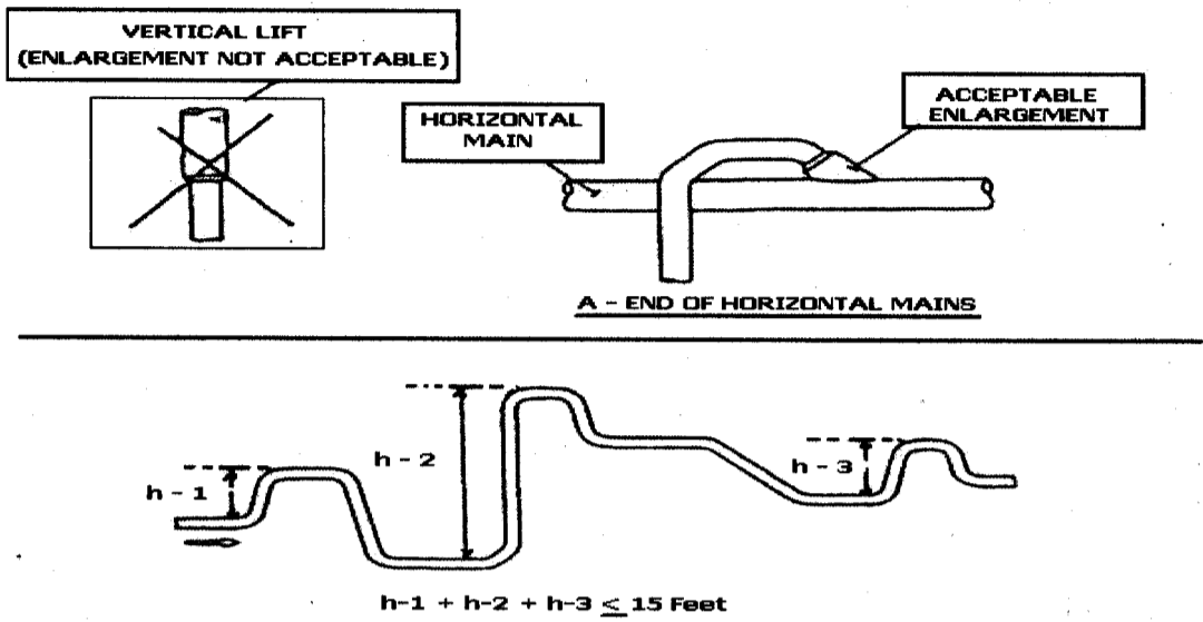
FIGURE F-11 VERTICAL LIFT RESTRICTIONS
