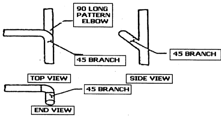
FIGURE-3 HORIZONTAL TO HORIZONTAL CONNECTION
