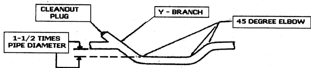
FIGURE F-1 REFORMING POCKETS
