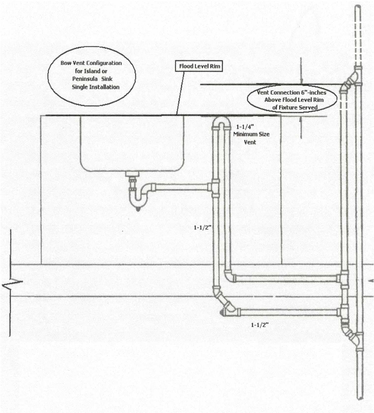
FIGURE 13A: Illustration of Bow Vent Single Installations.
