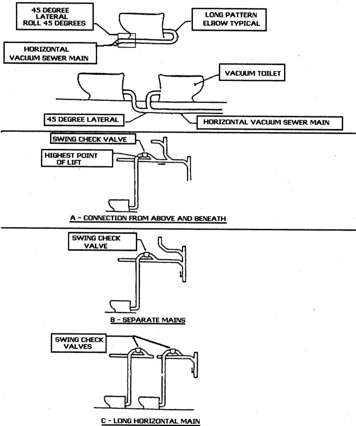
FIGURE F-9 TYPICAL VACUUM FIXTURE INSTALLATION (CONTINUED)
