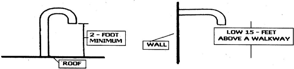
FIGURE F-8 VACUUM PUMP DISCHARGE PIPE TERMINATION
