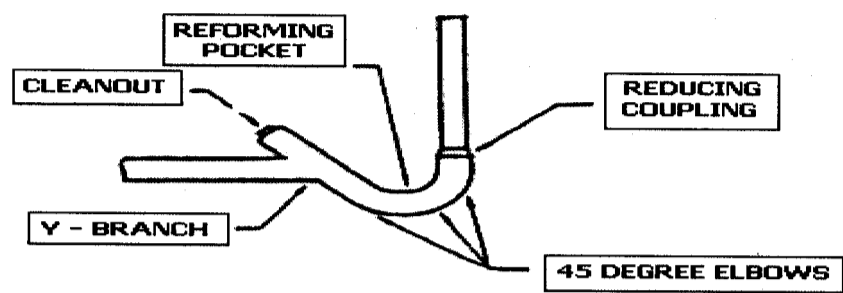
FIGURE F-5 HORIZONTAL TO VERTICAL LIFT CONNECTION
