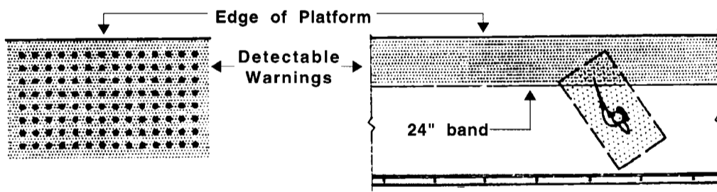
Detectable Warnings Figure 18a
