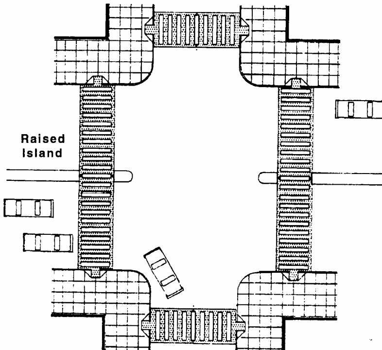
Curb Cuts at Intersection Figure 21a
