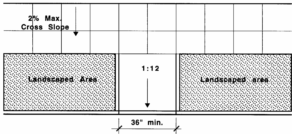
Curb Cut With Returned Sides Figure 21d
