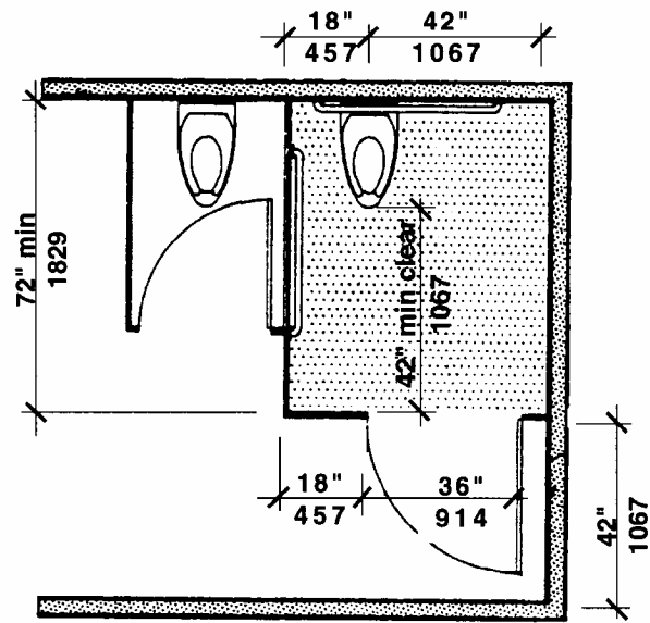
Accessible Toilet Stall (Left Approach) Figure 30a
