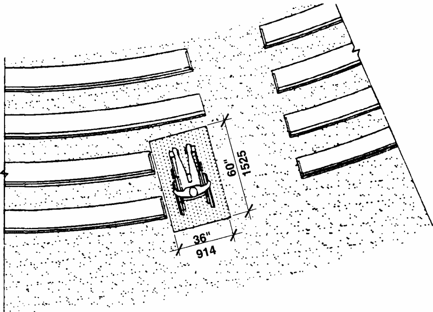
Wheelchair Seating Spaces Figure 16a
