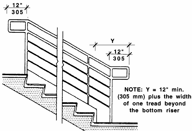
Handrail Extensions Figure 27d
