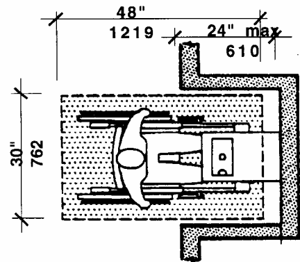
Front Approach (Cantilevered in a Recess) Figure 36e
