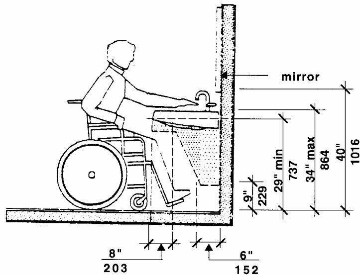
Sink Elevations Figure 30h
