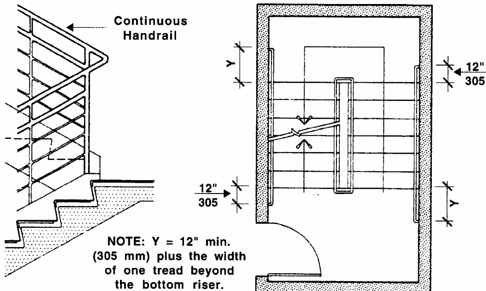
Handrails Figure 27c
