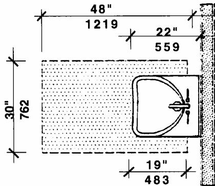
Clear Floor Space Figure 30g
