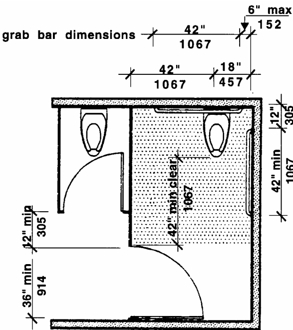
Accessible Toilet Stall (Right Approach) Figure 30b
