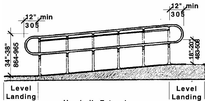
Handrail Extensions Figure 24d
