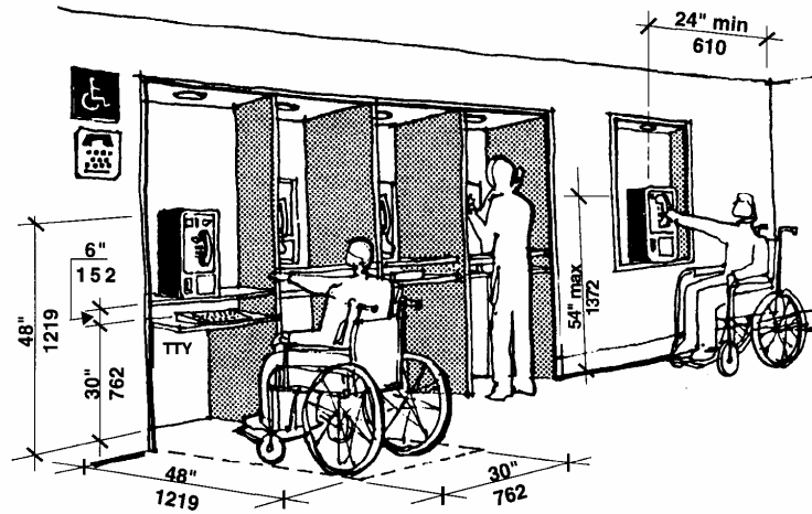
Accessible Telephones Figure 37a
