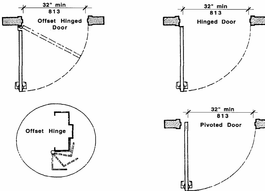
Clear Opening Figure 26b
