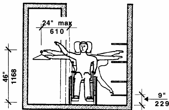
Reach Ranges Figure 34b
