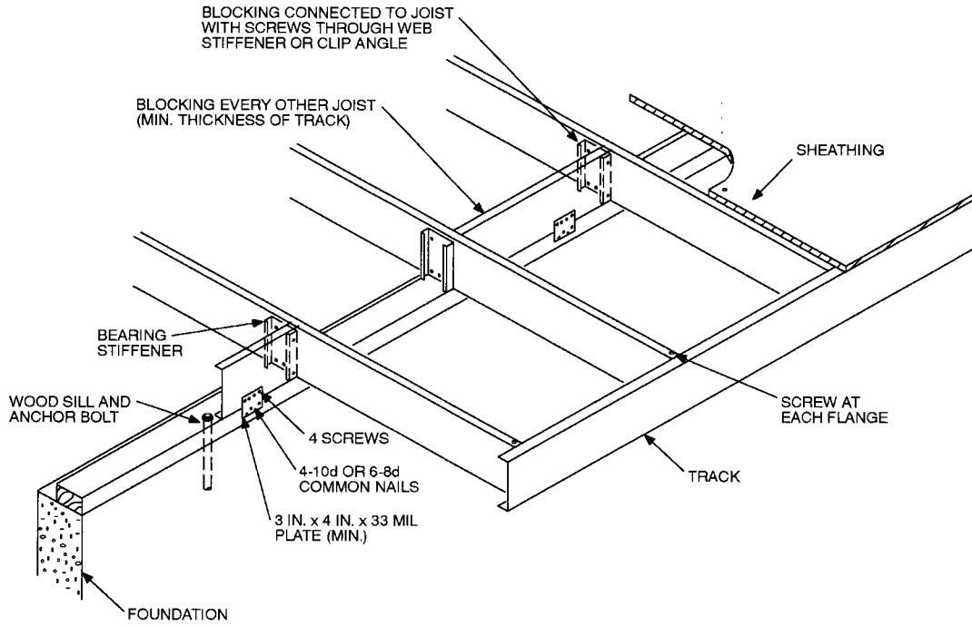
FIGURE 5505.3.1(5) FLOOR CANTILEVER TO WOOD SILL CONNECTION
