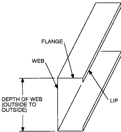
FIGURE 5505.2(1) C-SECTION
