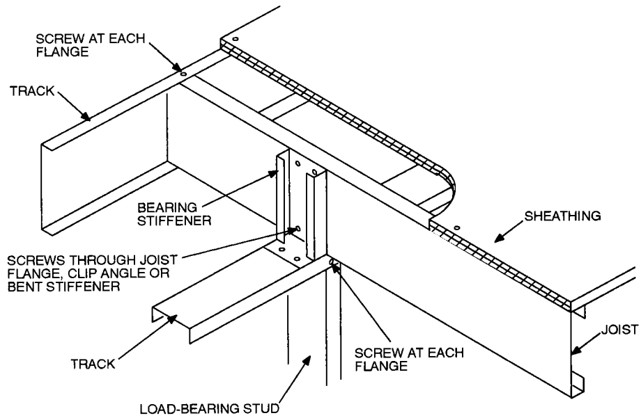
FIGURE 5505.3.1(4) FLOOR CANTILEVER TO LOAD-BEARING WALL CONNECTION
