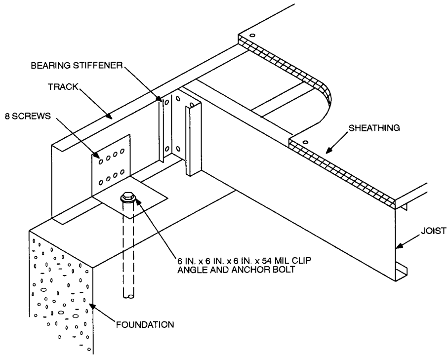
FIGURE 5505.3.1(3) FLOOR TO FOUNDATION CONNECTION
