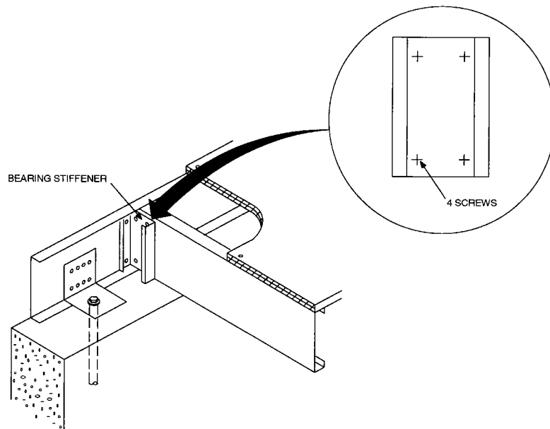
FIGURE 5505.3.4 BEARING STIFFENER
