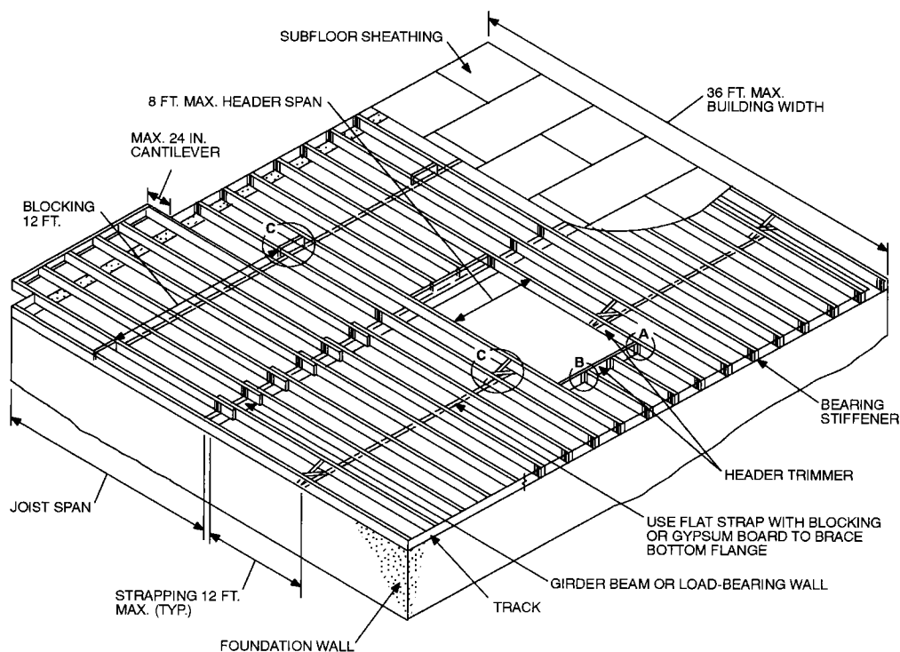
FIGURE 5505.3 STEEL FLOOR CONSTRUCTION
