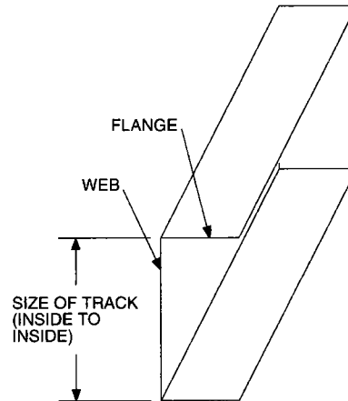
FIGURE 5505.2(2) TRACK SECTION
