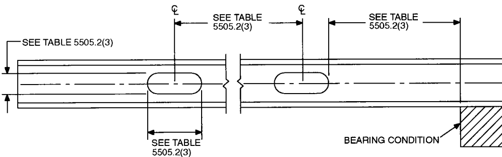
FIGURE 5505.2(1) C-SECTION
