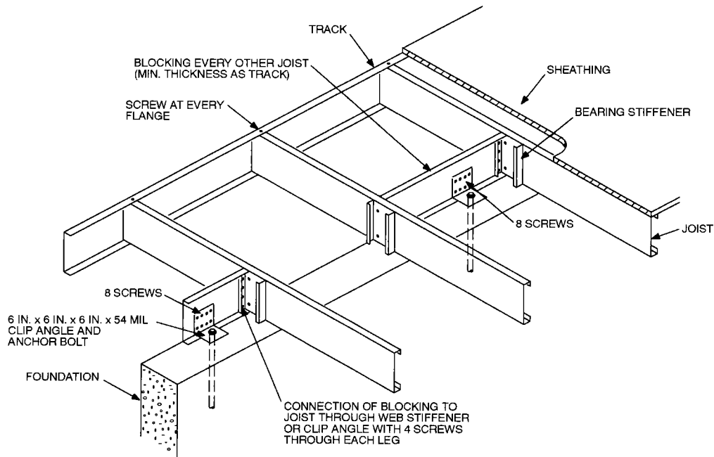
FIGURE 5505.3.1(6) FLOOR CANTILEVER TO FOUNDATION CONNECTION
