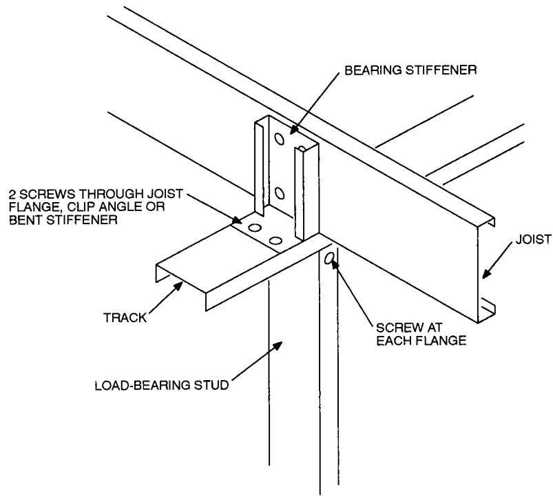
FIGURE 5505.3.1(7) CONTINUOUS JOIST SPAN SUPPORTED ON STUD
