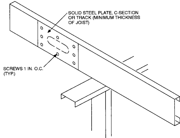
FIGURE 5505.3.6 HOLE PATCH
