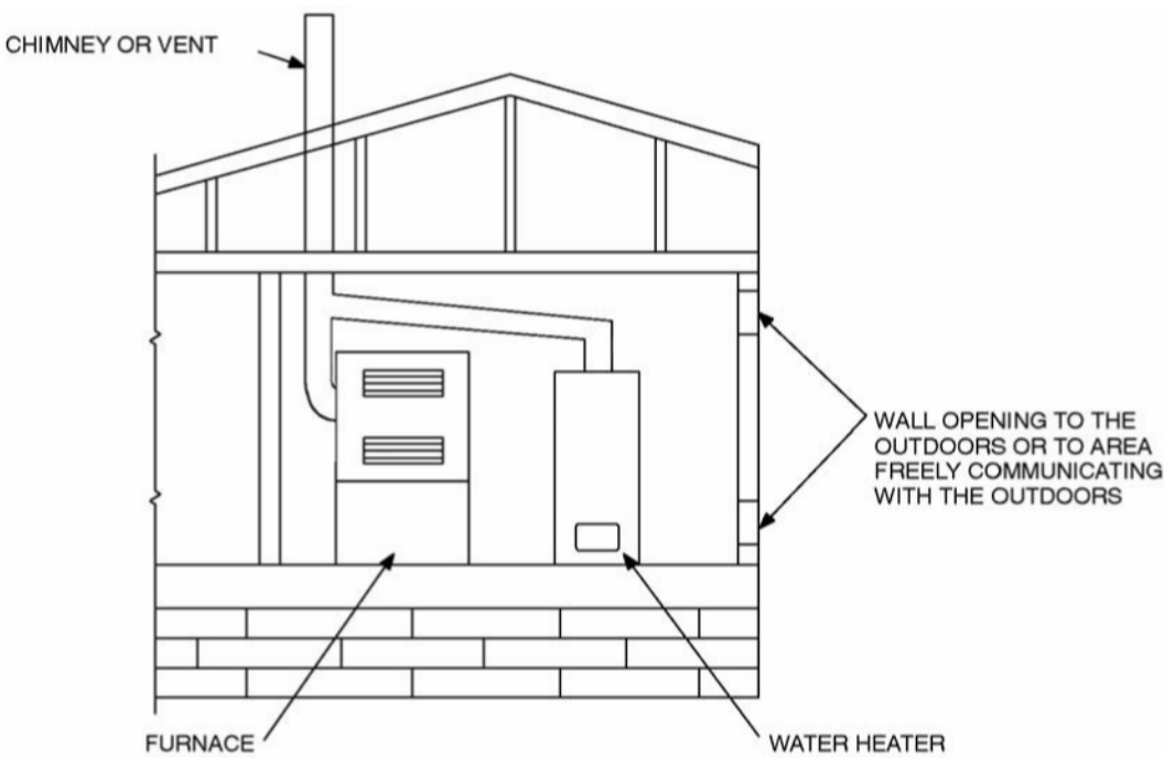
780 CMR FIGURE 6703.2(1) APPLIANCES LOCATED IN CONFINED SPACES—ALL AIR TAKEN FROM OUTDOORS THROUGH TWO OPENINGS
