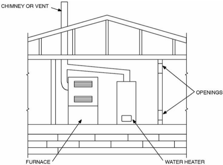
780CMR FIGURE 6702.2 APPLIANCES LOCATED IN CONFINED SPACES—ALL AIR TAKEN FROM ADJACENT SPACES WITHIN THE BUILDING
