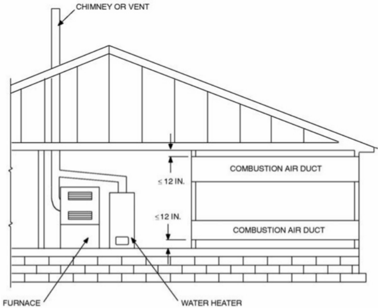
780 CMR FIGURE 6703.2(2) APPLIANCES LOCATED IN CONFINED SPACES—ALL AIR TAKE FROM OUTDOORS THROUGH HORIZONTAL DUCTS
