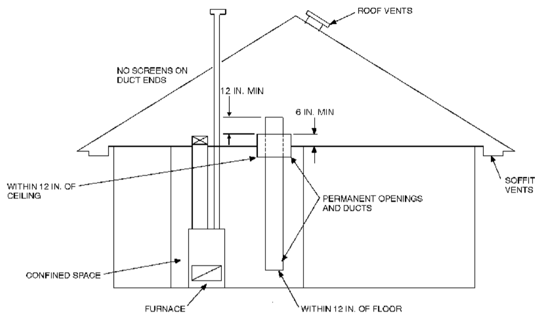
780 CMR FIGURE 6703.3 APPLIANCES LOCATED IN CONFINED SPACES—ALL AIR TAKEN FROM OUTDOORS THROUGH VENTILATED ATTIC, INLET DUCT WITHIN OUTLET DUCT
