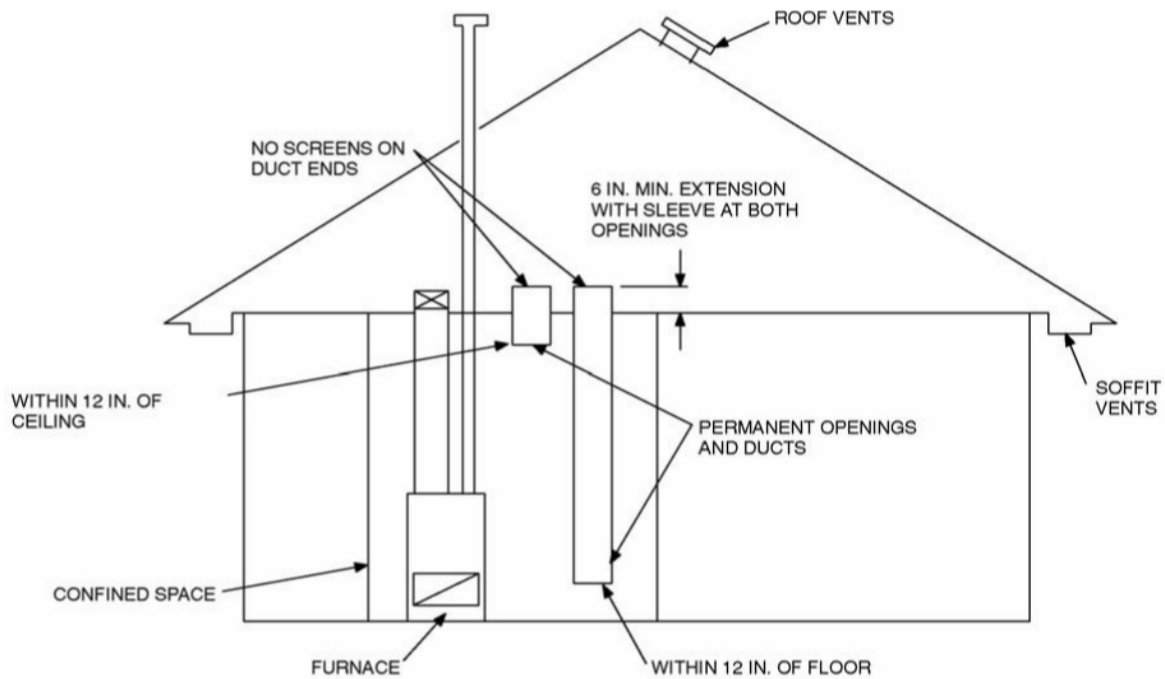
780 CMR FIGURE 6703.2(3) APPLIANCES LOCATED IN CONFINED SPACES—ALL AIR TAKEN FROM OUTDOORS THROUGH VENTILATED ATTIC
