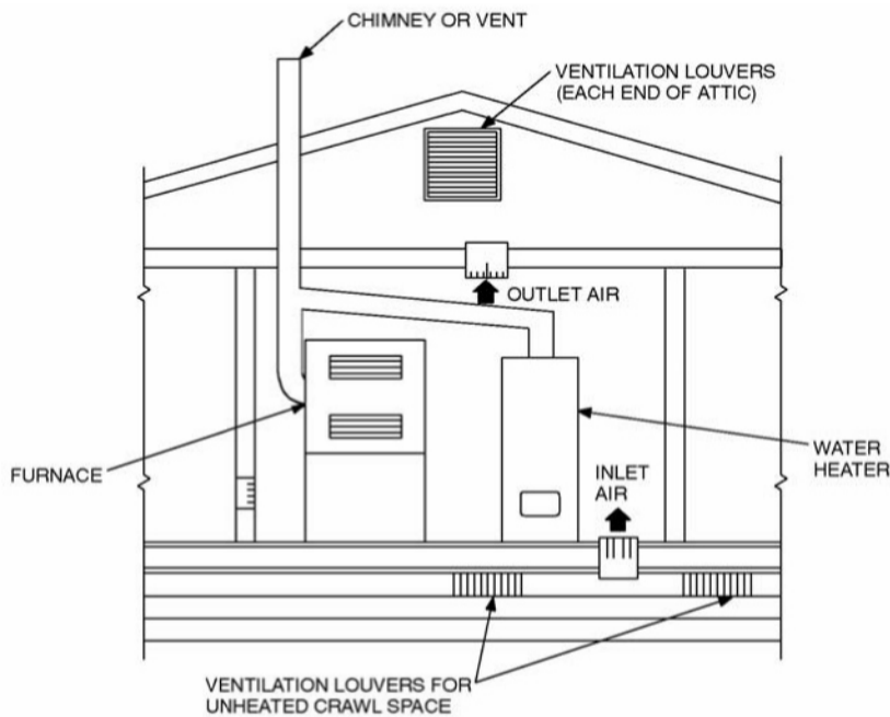
780 CMR FIGURE 6703.2(4) APPLIANCES LOCATED IN CONFINED SPACES—INLET AIR TAKEN FROM VENTILATED CRAWL SPACE AND OUTLET AIR TO VENTILATED ATTIC
