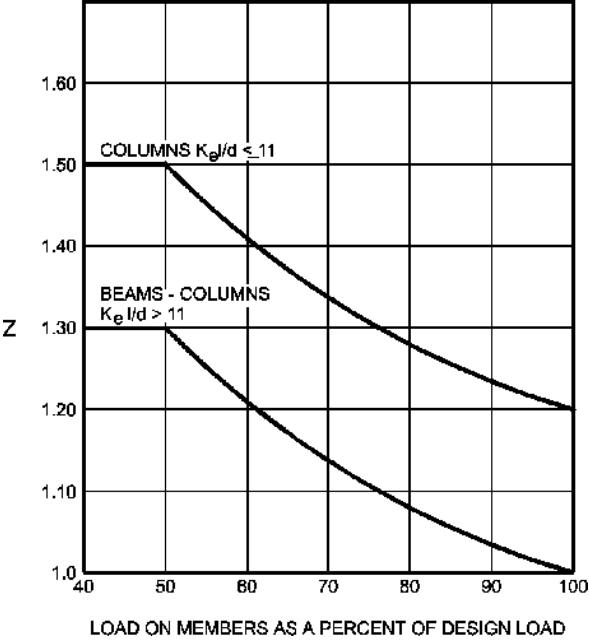
Figure 721.6.3(1) LOAD FIGURE
