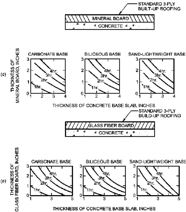
Figure 721.2.2.3(2) FIRE-RESISTANCE RATINGS FOR CONCRETE ROOF ASSEMBLIES
