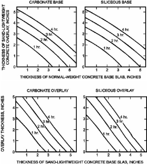
Figure 721.2.2.2 FIRE-RESISTANCE RATINGS FOR TWO- COURSE CONCRETE FLOORS
