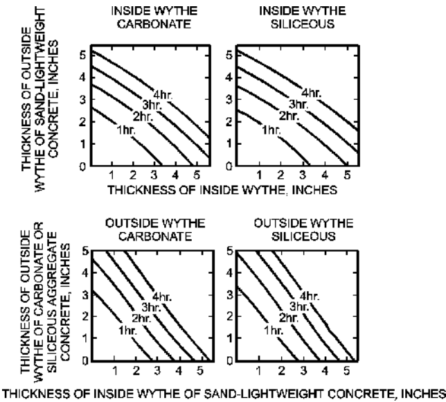
Figure 721.2.1.2 FIRE-RESISTANCE RATINGS OF TWO- WYTHE CONCRETE WALLS
