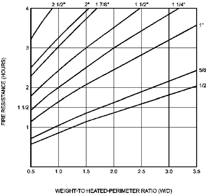
Figure 721.5.1(4) FIRE RESISTANCE OF STRUCTURAL STEEL COLUMNS PROTECTED WITH VARIOUS THICKNESSES OF TYPE X GYPSON WALLBOARD
