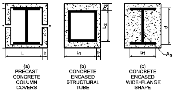
Figure 721.5.1(6) CONCRETE PROTECTED STRUCTURAL STEEL COLUMNS
