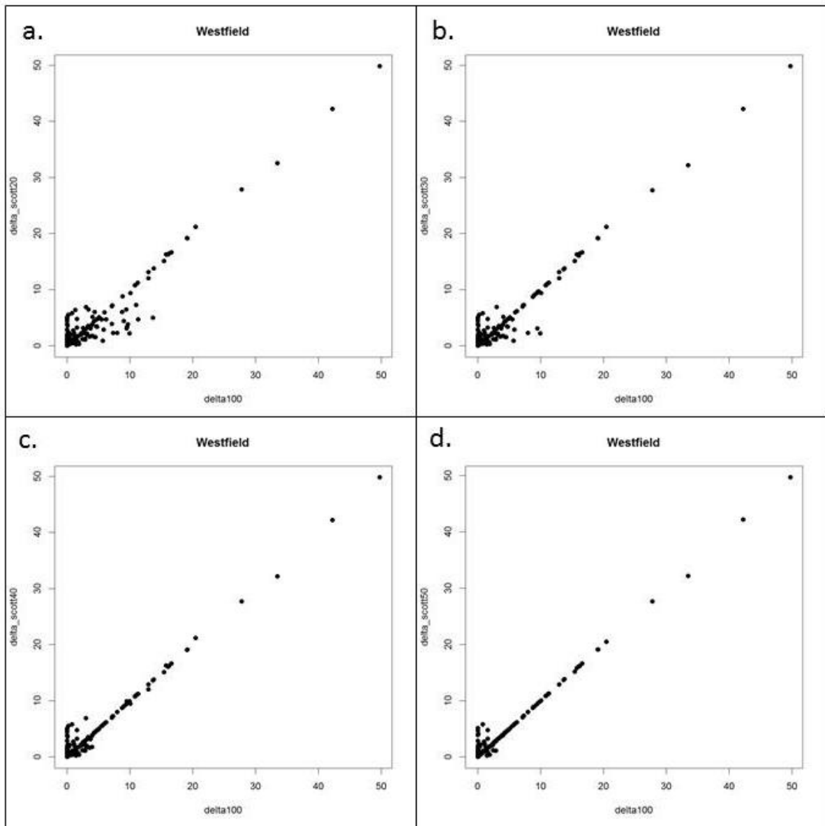
Figure AE-10. Correlation plots for crossings strategically selected for field assessment compared to (near) comprehensive crossing assessment in a portion of the Westfield River watershed: a. 20%, b. 30%, c. 40% and d. 50%.
