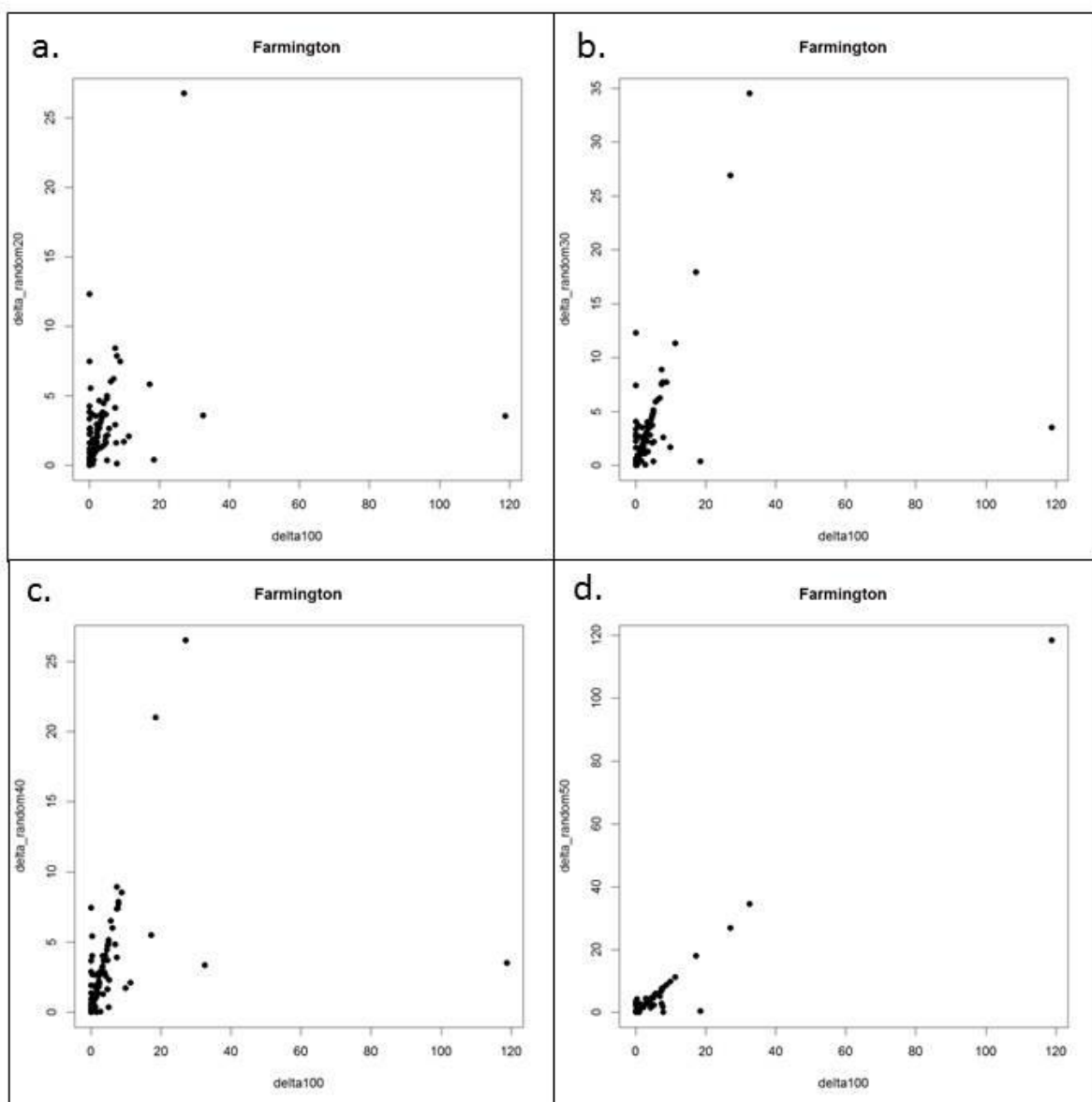
Figure AE-3. Correlation plots for crossings randomly selected for field assessment compared to (near) comprehensive crossing assessment in a portion of the Farmington River watershed: a. 20%, b. 30%, c. 40% and d. 50%.
