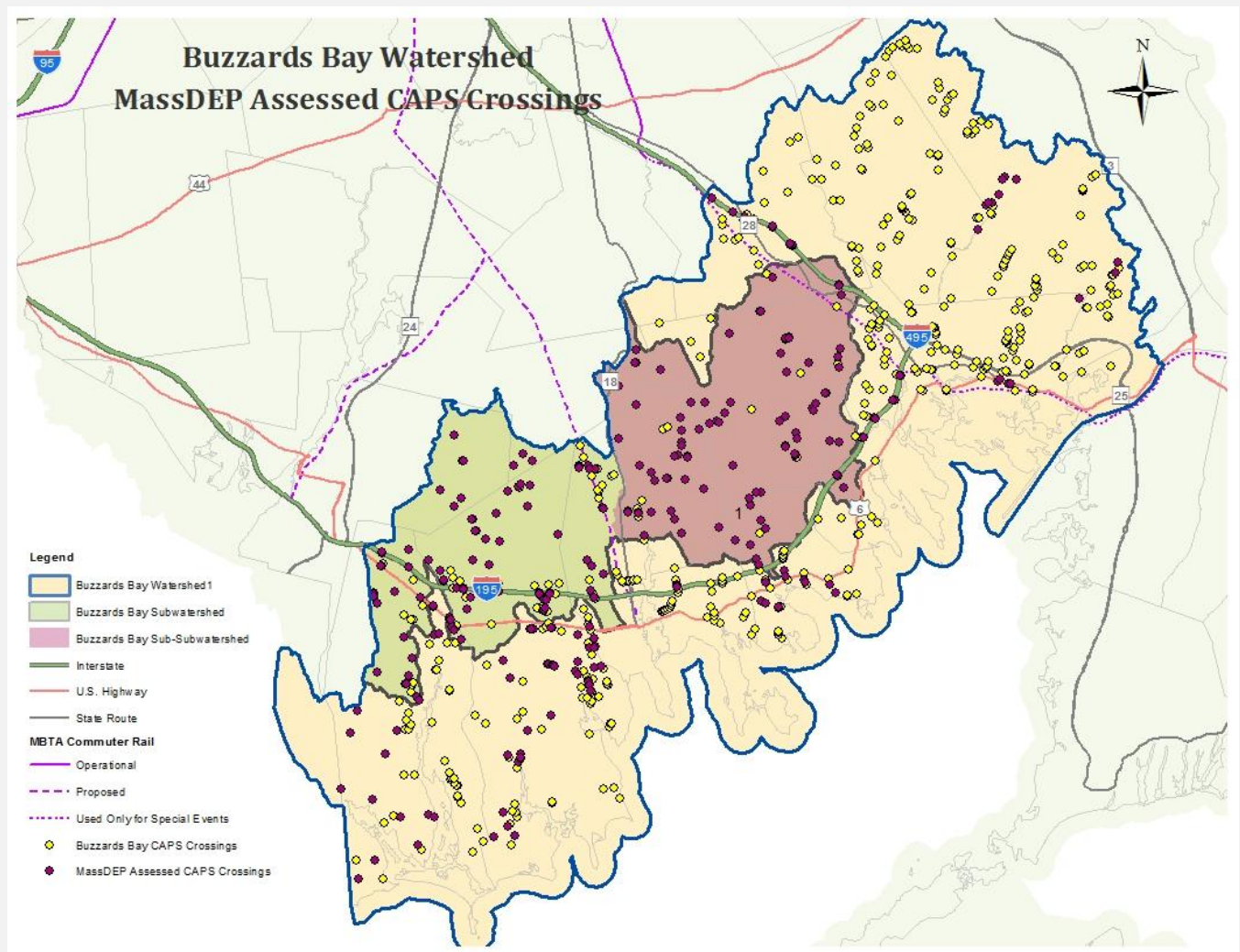
Figure AC-2. Plot of MassDEP stream crossing assessments completed in the Buzzards Bay Watershed with CAPS Crossings added as a reference.
