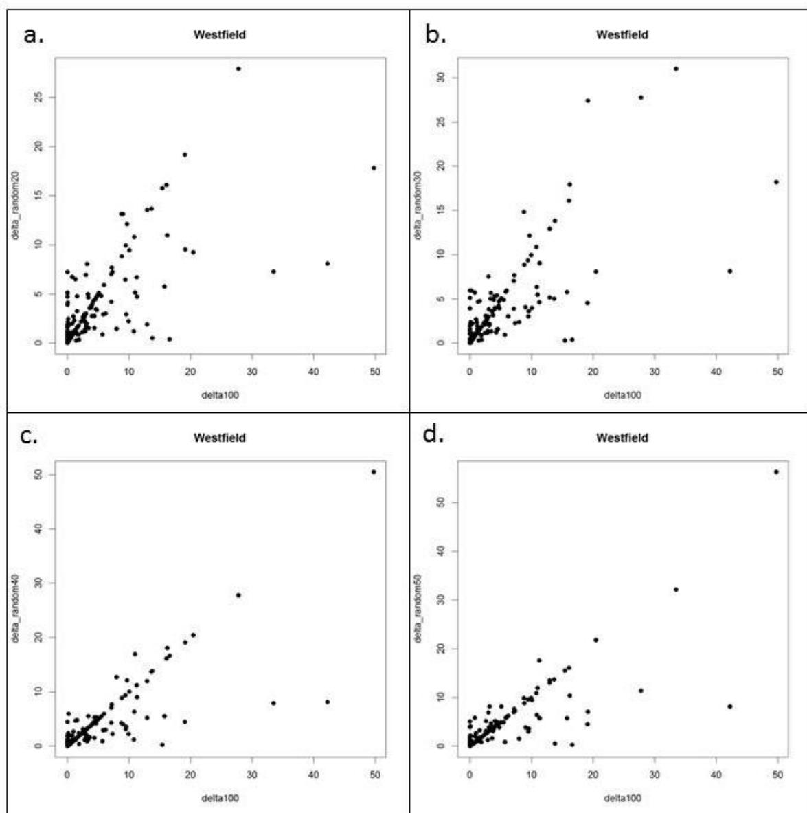
Figure AE-9. Correlation plots for crossings randomly selected for field assessment compared to (near) comprehensive crossing assessment in a portion of the Westfield River watershed: a. 20%, b. 30%, c. 40% and d. 50%.
