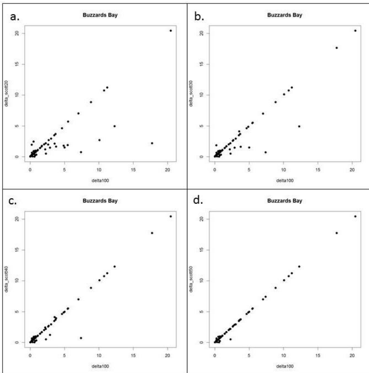
Figure AE-2. Correlation plots for crossings strategically selected for field assessment compared to (near) comprehensive crossing assessment in a portion of the Buzzards Bay watershed: a. 20%, b. 30%, c. 40% and d. 50%.
