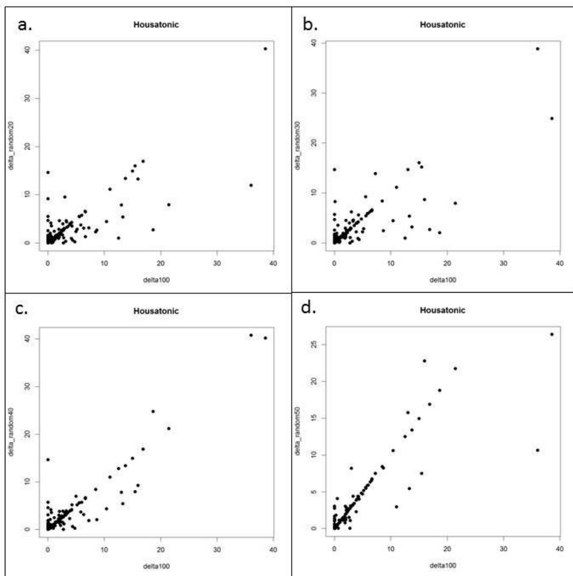
Figure AE-5. Correlation plots for crossings randomly selected for field assessment compared to (near) comprehensive crossing assessment in a portion of the Housatonic River watershed: a. 20%, b. 30%, c. 40% and d. 50%.
