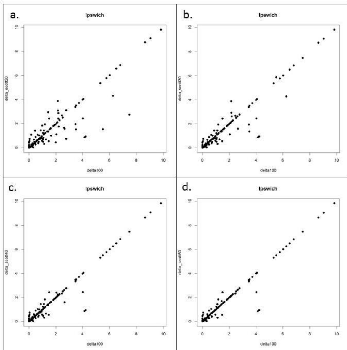
Figure AE-8. Correlation plots for crossings strategically selected for field assessment compared to (near) comprehensive crossing assessment in a portion of the Ipswich River watershed: a. 20%, b. 30%, c. 40% and d. 50%.
