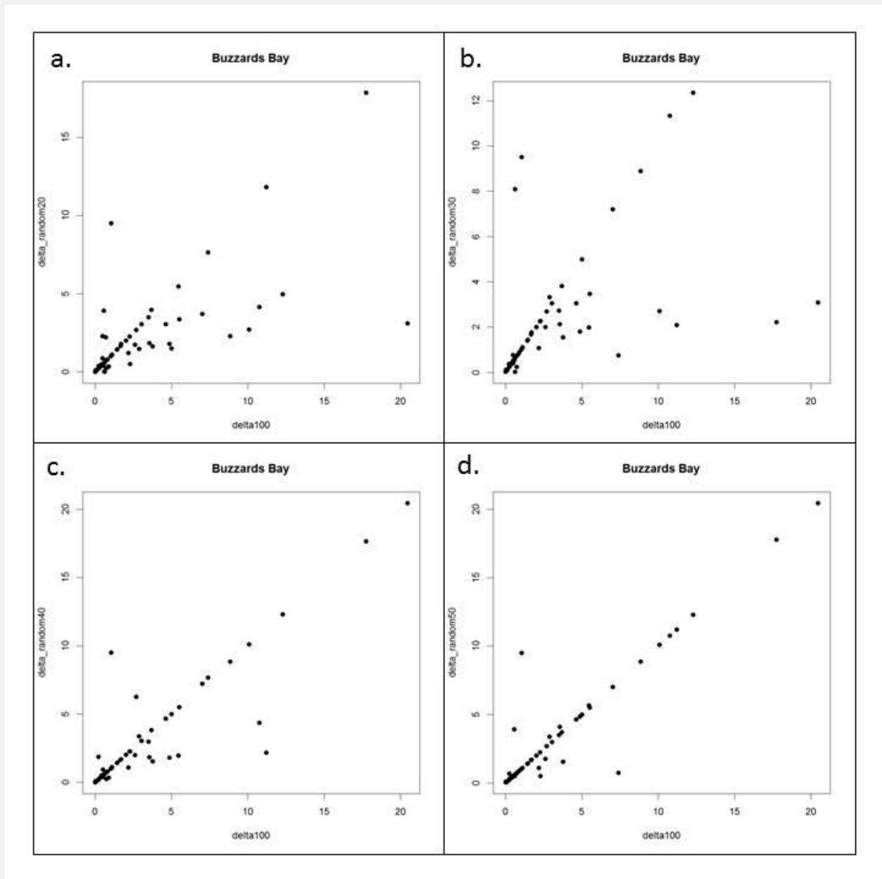
Figure AE-1. Correlation plots for crossings randomly selected for field assessment compared to (near) comprehensive crossing assessment in a portion of the Buzzards Bay watershed: a. 20%, b. 30%, c. 40% and d. 50%.
