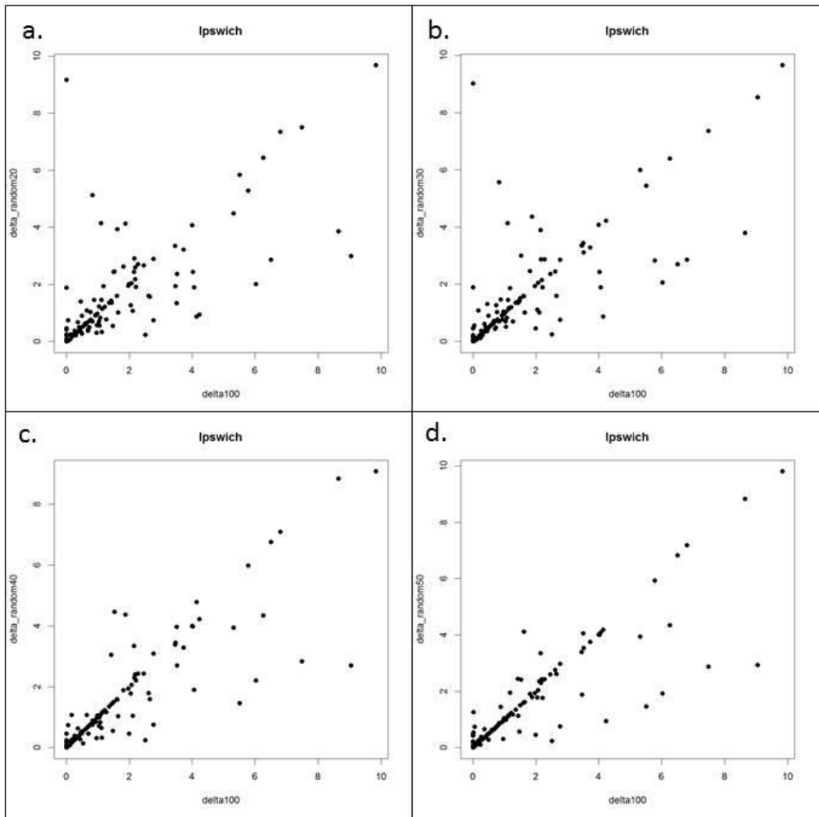
Figure AE-7. Correlation plots for crossings randomly selected for field assessment compared to (near) comprehensive crossing assessment in a portion of the Ipswich River watershed: a. 20%, b. 30%, c. 40% and d. 50%.
