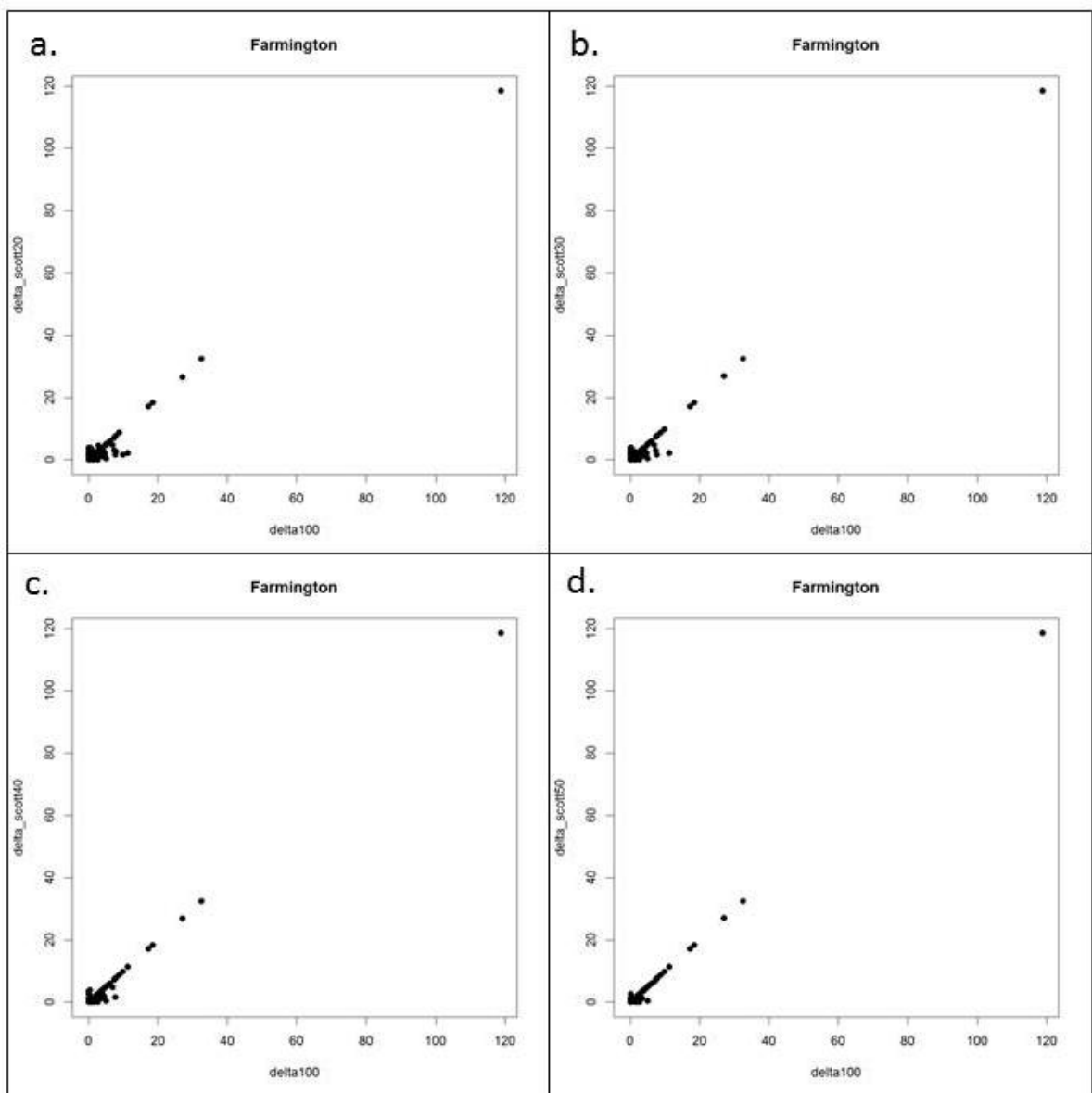
Figure AE-4. Correlation plots for crossings strategically selected for field assessment compared to (near) comprehensive crossing assessment in a portion of the Farmington River watershed: a. 20%, b. 30%, c. 40% and d. 50%.
