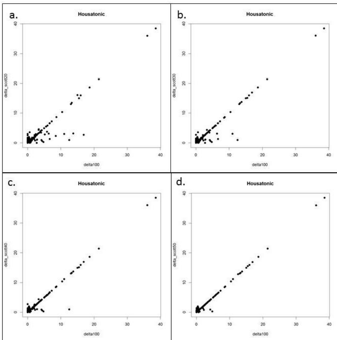
Figure AE-6. Correlation plots for crossings strategically selected for field assessment compared to (near) comprehensive crossing assessment in a portion of the Housatonic River watershed: a. 20%, b. 30%, c. 40% and d. 50%.
