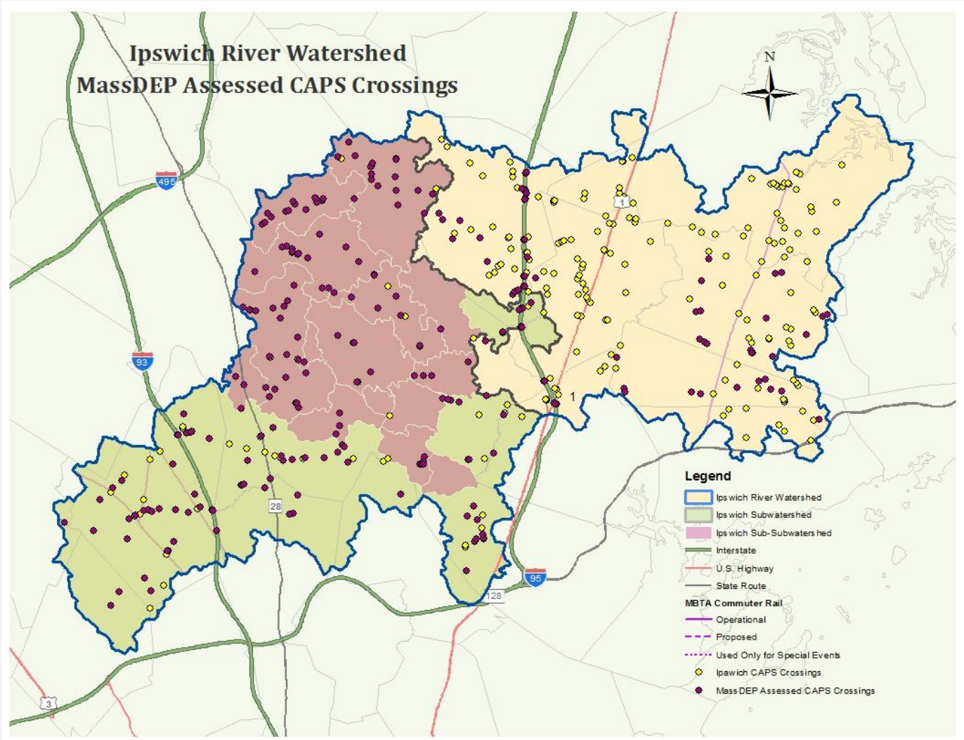
Figure AC-1. Plot of MassDEP stream crossing assessments completed in the Ipswich River Watershed with CAPS Crossings added as a reference.
