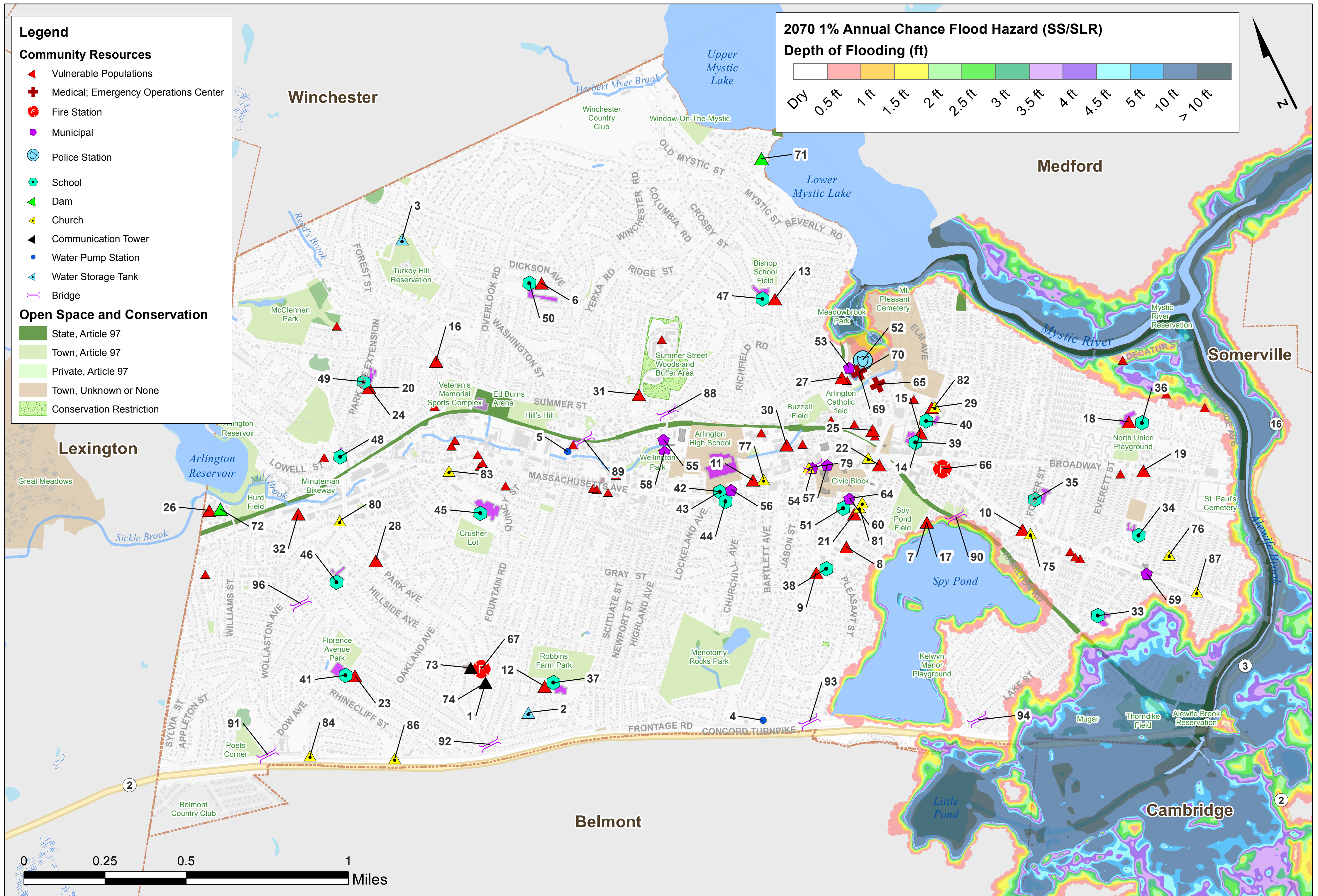
Sea Level Rise and Storm Surge Flooding
