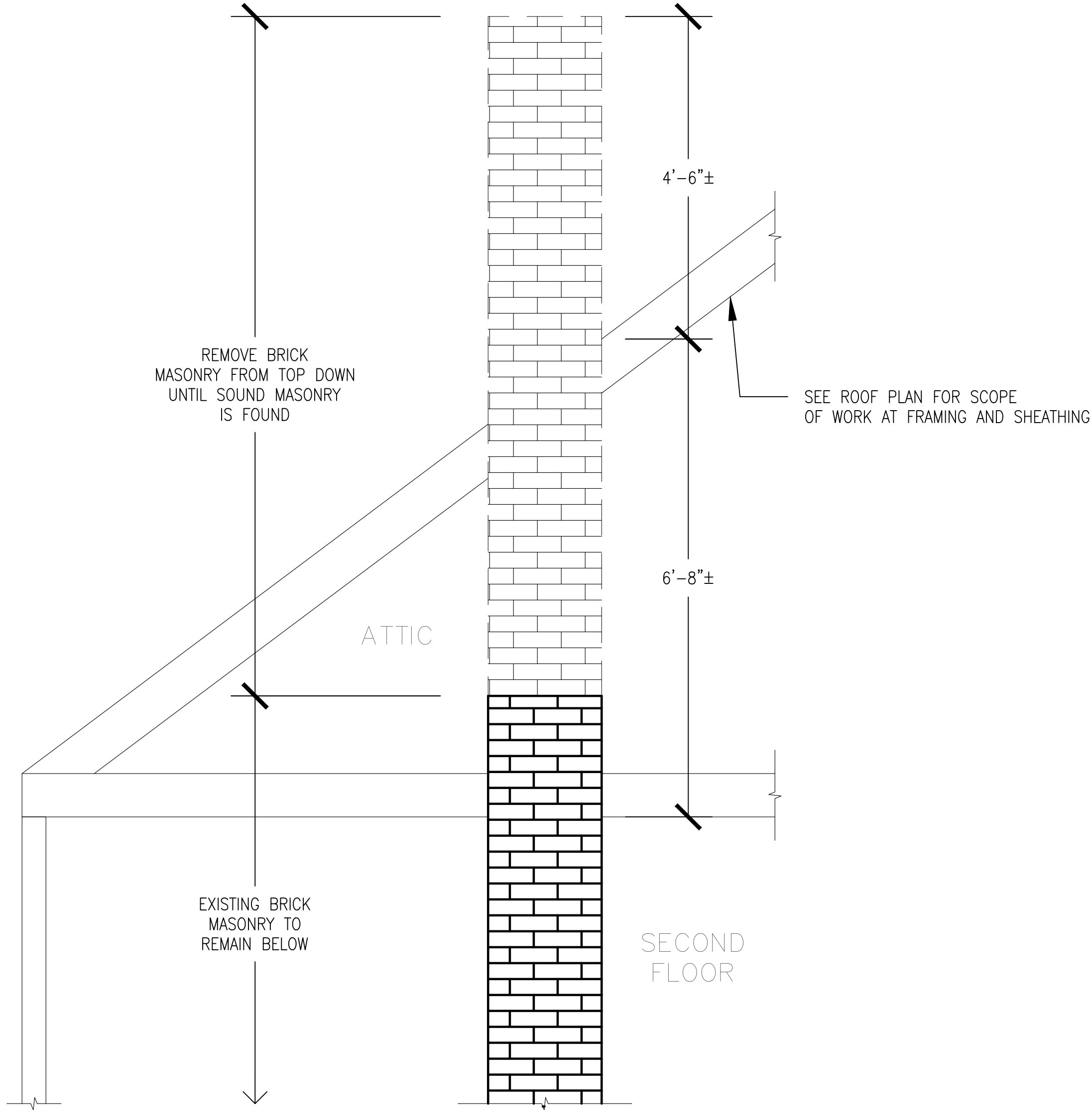
2 REAR CHIMNEY ATTIC SECTION
