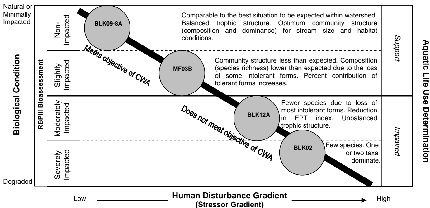
Figure 3. A schematic of results of the RBPIII analysis of the 2003 Blackstone River watershed biomonitoring stations as they relate to Tiered Aquatic Life Use.
