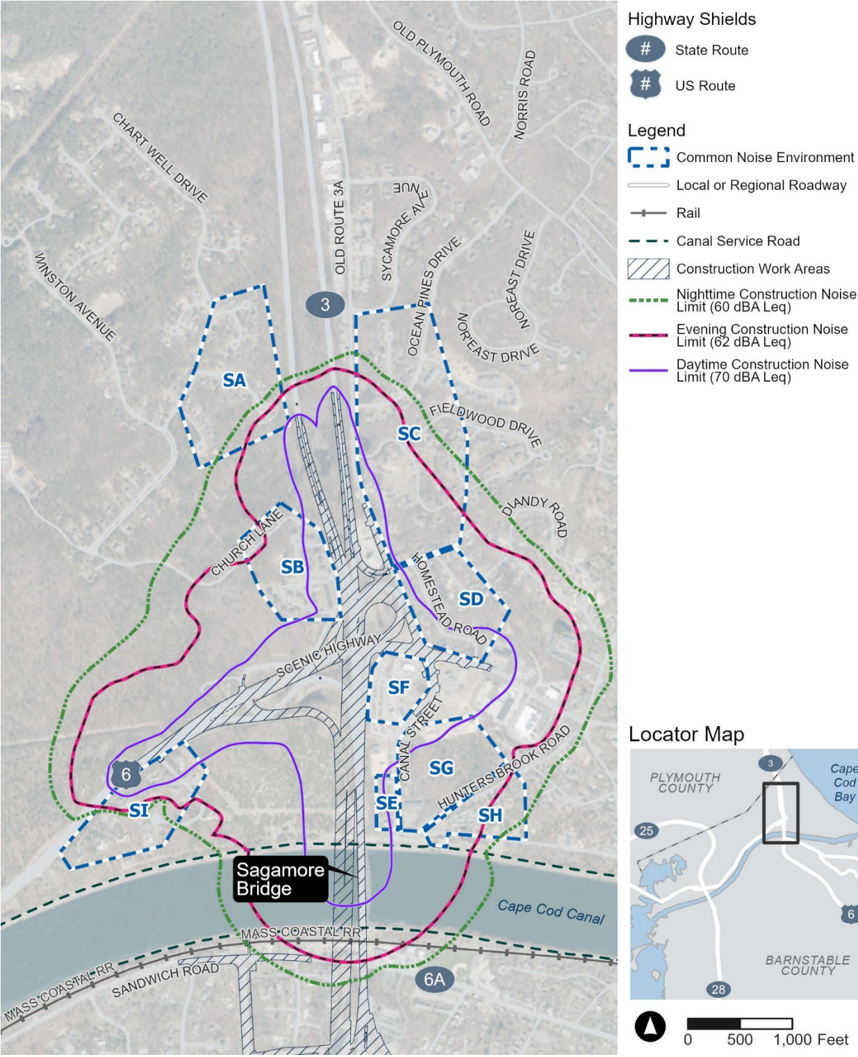
Figure 6-5. Construction Work Areas and Predicted Construction Noise Limit Contours (Sagamore North Quadrant)
