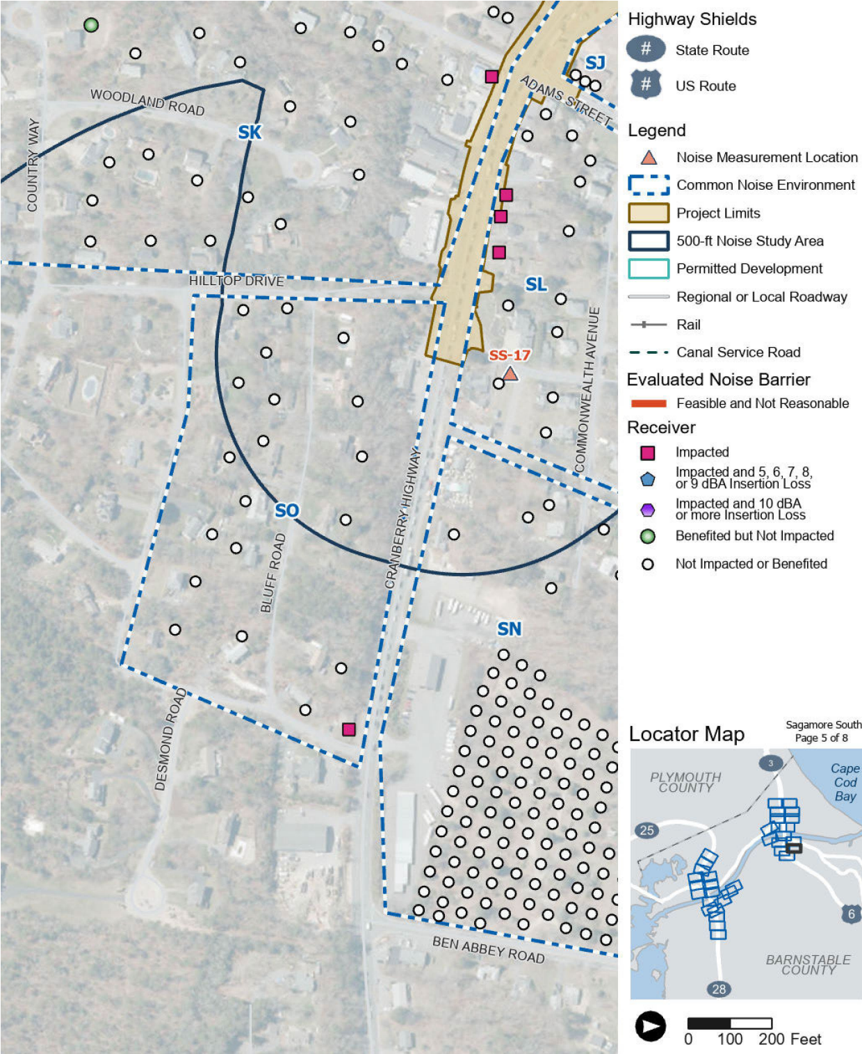
Figure 6-2. Build Alternative Location Map for Barriers, Common Noise Environments, and Receptors (Sagamore South) (5 of 8)
