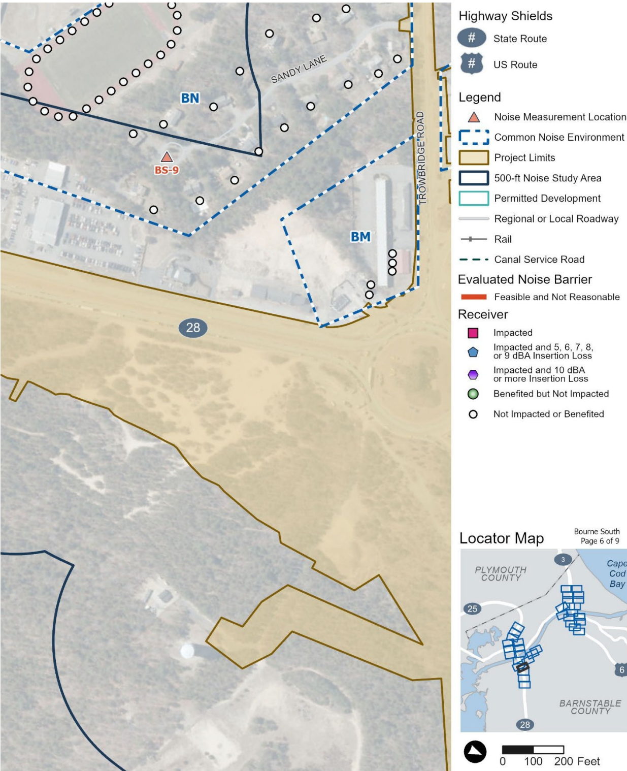
Figure 6-4. Build Alternative: Location Map for Barriers, Common Noise Environments, and Receptors (Bourne South Quadrant) (6 of 9)
