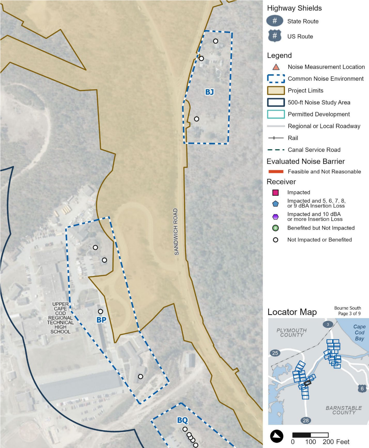
Figure 6-4. Build Alternative: Location Map for Barriers, Common Noise Environments, and Receptors (Bourne South Quadrant) (3 of 9)
