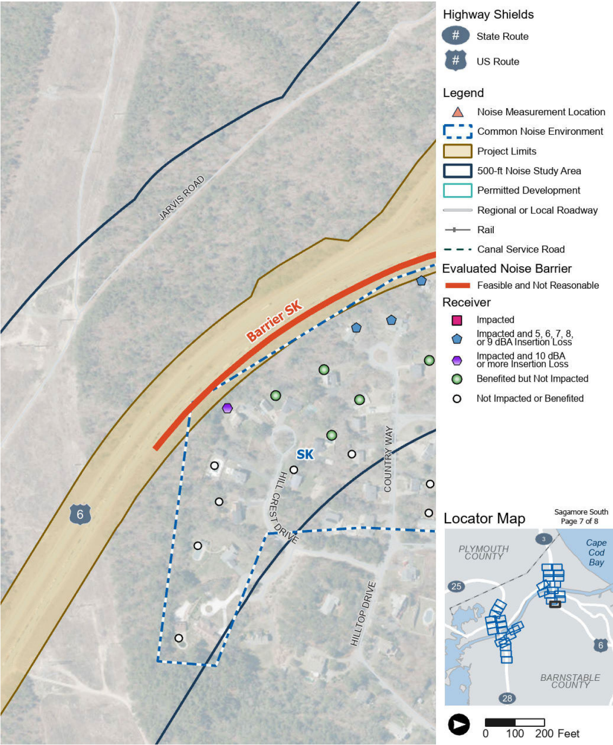
Figure 6-2. Build Alternative Location Map for Barriers, Common Noise Environments, and Receptors (Sagamore South) (7 of 8)
