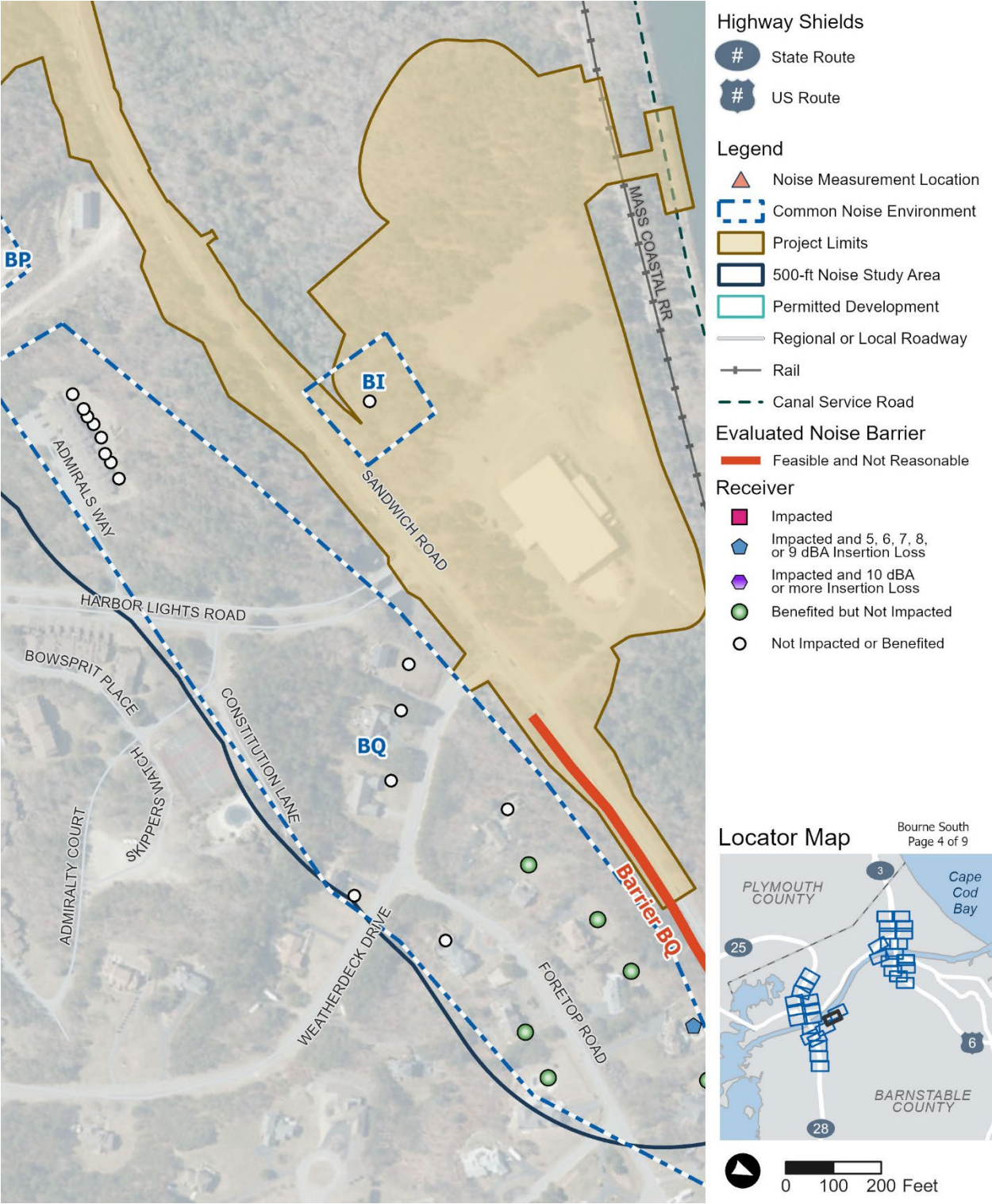
Figure 6-4. Build Alternative: Location Map for Barriers, Common Noise Environments, and Receptors (Bourne South Quadrant) (4 of 9)
