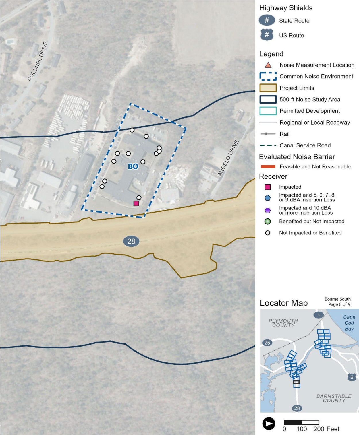
Figure 6-4. Build Alternative: Location Map for Barriers, Common Noise Environments, and Receptors (Bourne South Quadrant) (8 of 9)
