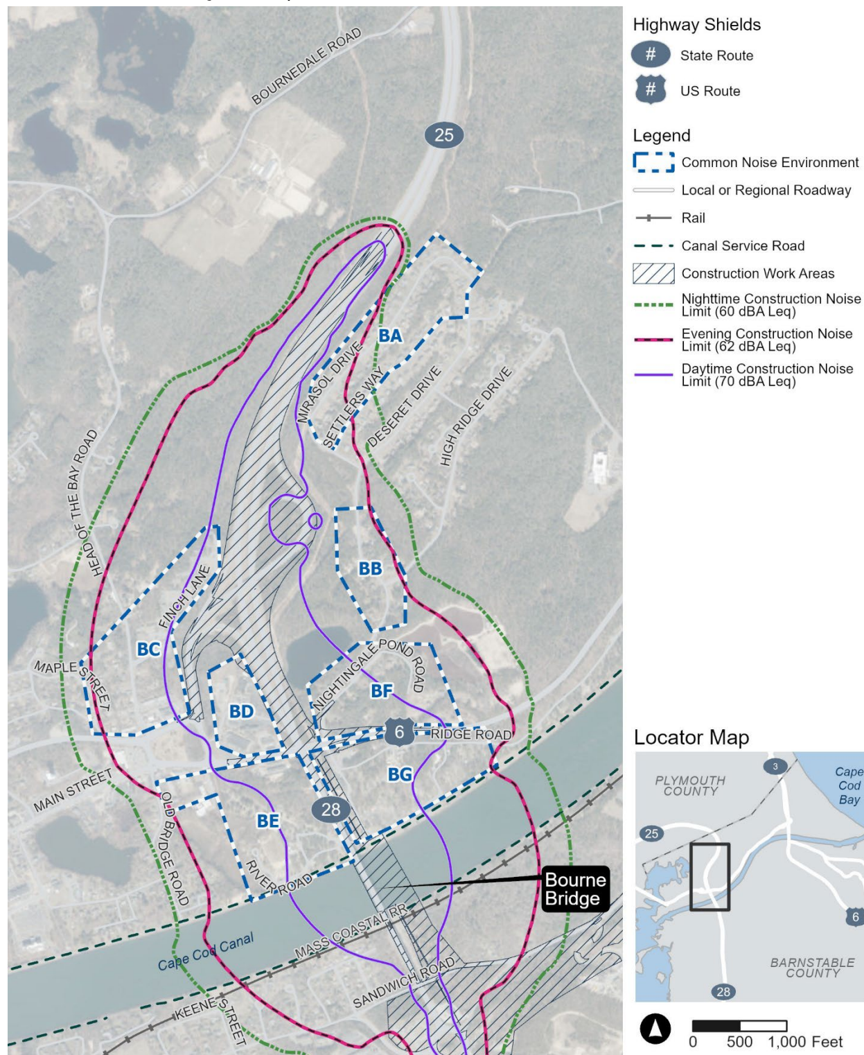
Figure 6-7. Construction Work Areas and Predicted Construction Noise Limit Contours (Bourne North Quadrant)
