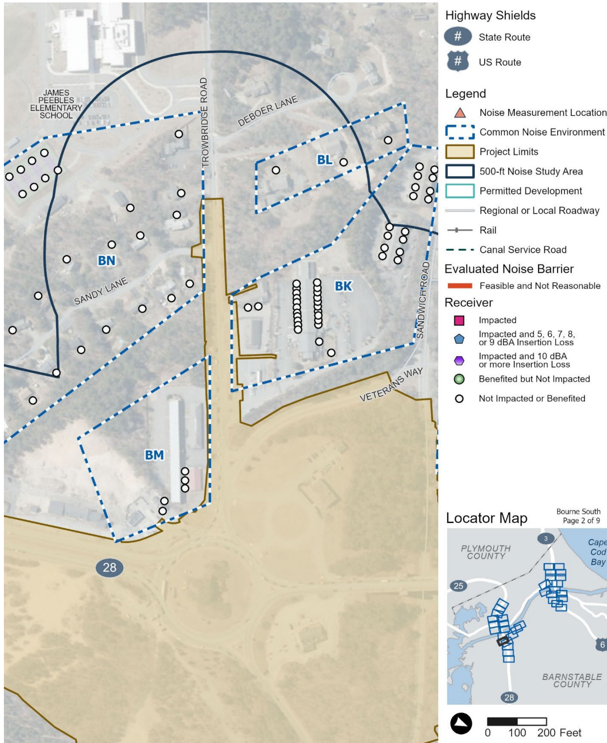
Figure 6-4. Build Alternative: Location Map for Barriers, Common Noise Environments, and Receptors (Bourne South Quadrant) (2 of 9)
