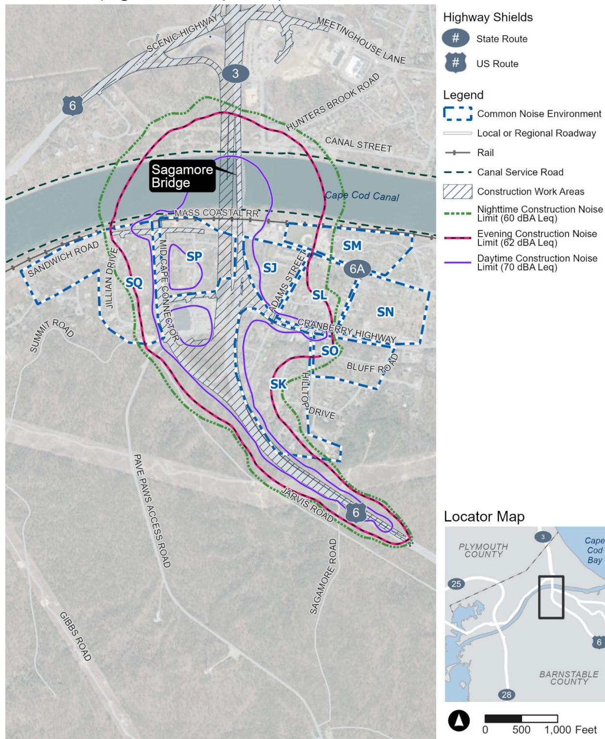
Figure 6-6. Construction Work Areas and Predicted Construction Noise Limit Contours (Sagamore South Quadrant)
