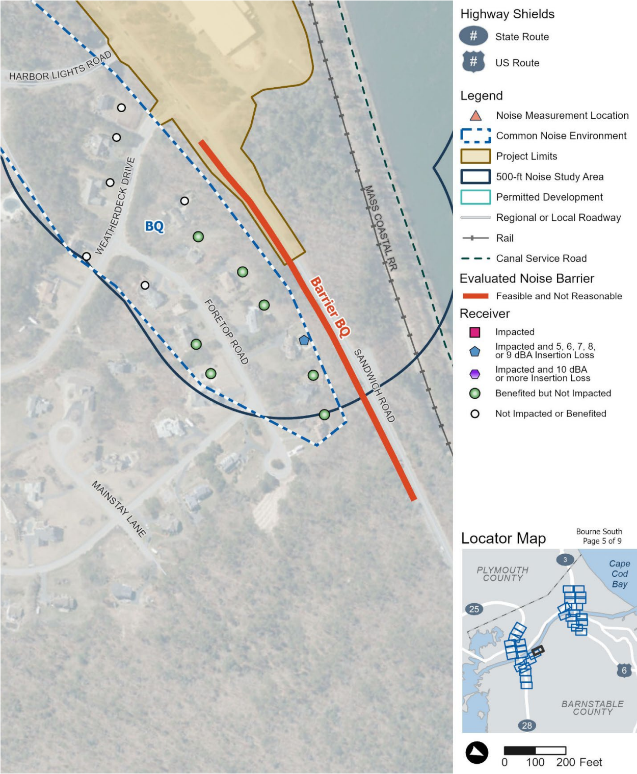
Figure 6-4. Build Alternative: Location Map for Barriers, Common Noise Environments, and Receptors (Bourne South Quadrant) (5 of 9)
