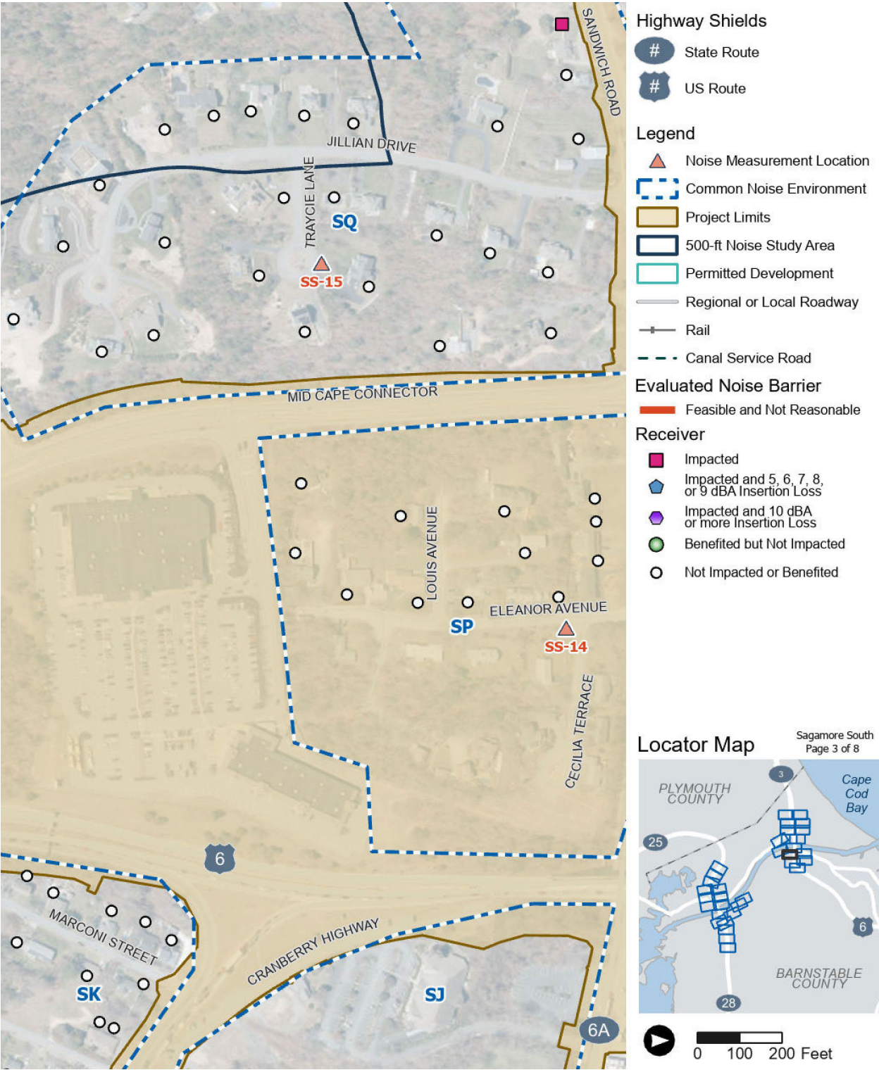
Figure 6-2. Build Alternative Location Map for Barriers, Common Noise Environments, and Receptors (Sagamore South) (3 of 8)
