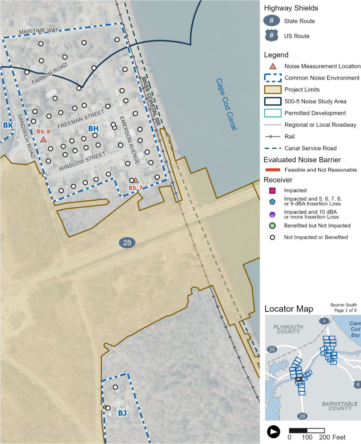
Figure 6-4. Build Alternative: Location Map for Barriers, Common Noise Environments, and Receptors (Bourne South Quadrant) (1 of 9)
