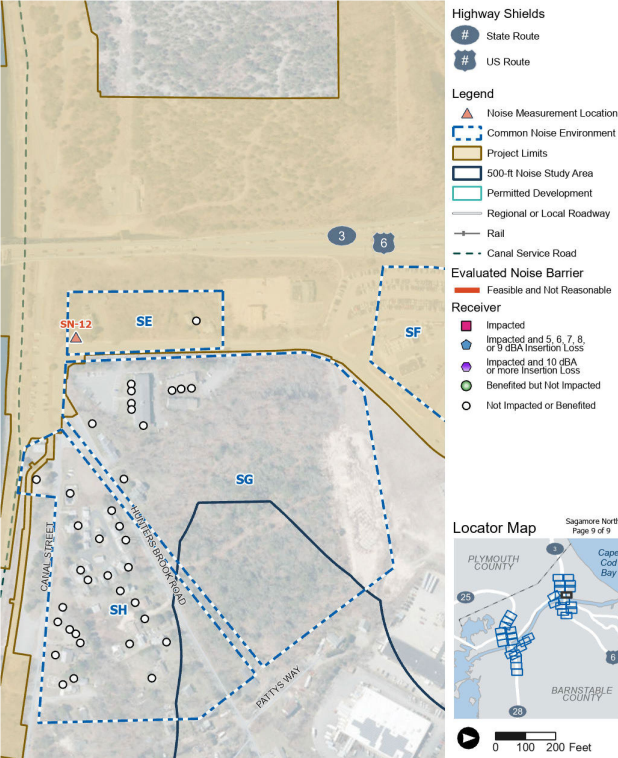
Figure 6-1. Build Alternative: Location Map for Barriers, Common Noise Environments, and Receptors (Sagamore North Quadrant) (9 of 9)
