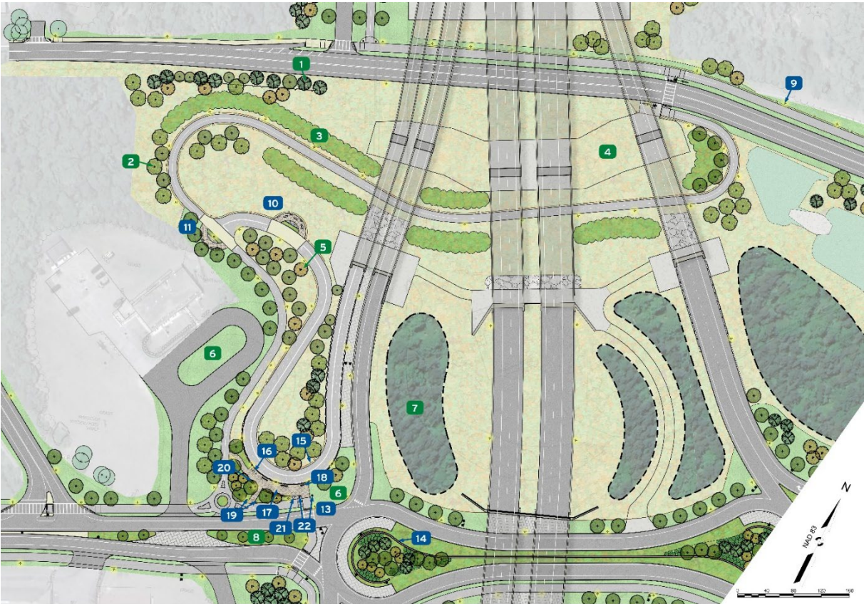
Figure 8-4. Landscape Plan and Amenities: Shared-Use Path at State Route 28 and Diamond Interchange Roundabouts, Bourne South Quadrant
