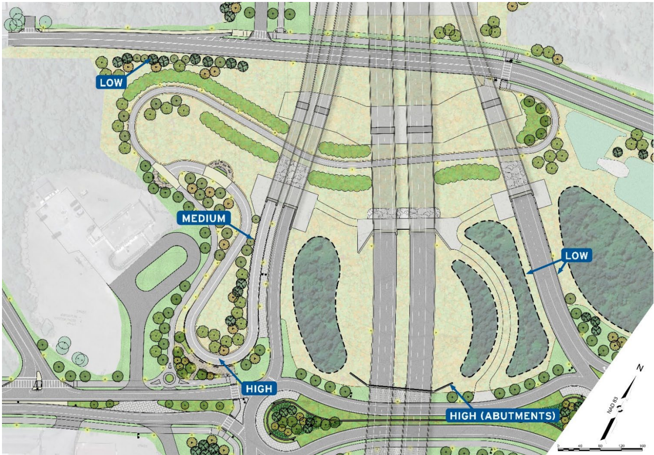
Figure 8-6. .... Example of Retaining Wall Potential Exposure Assessment, Bourne South
