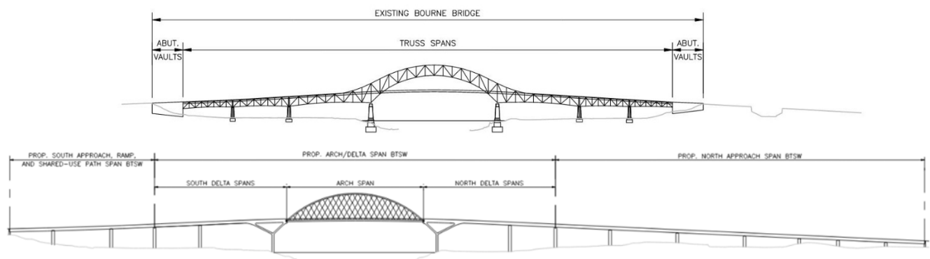
Figure 7-2. Comparison of Existing and Proposed Bourne Bridge
