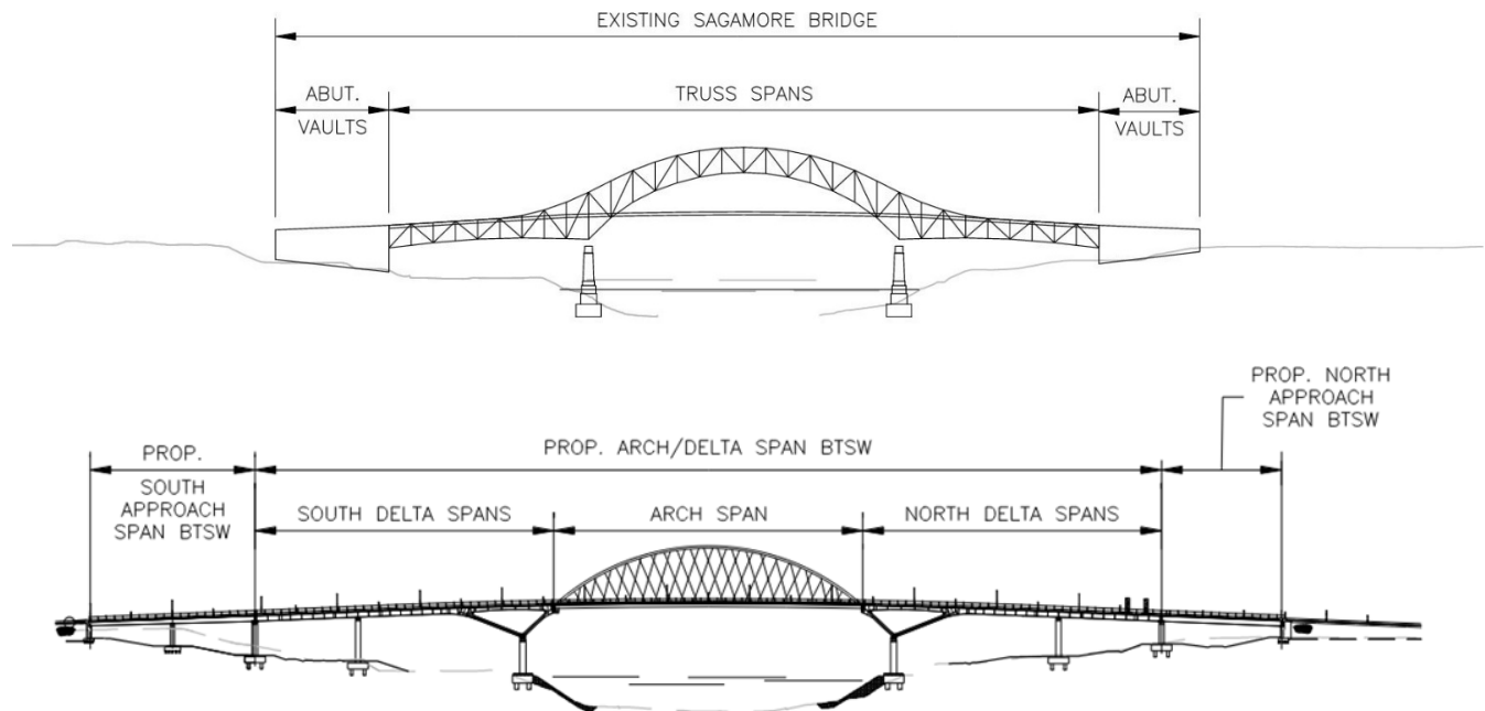
Figure 7-1. Comparison of Existing and Proposed Sagamore Bridge
