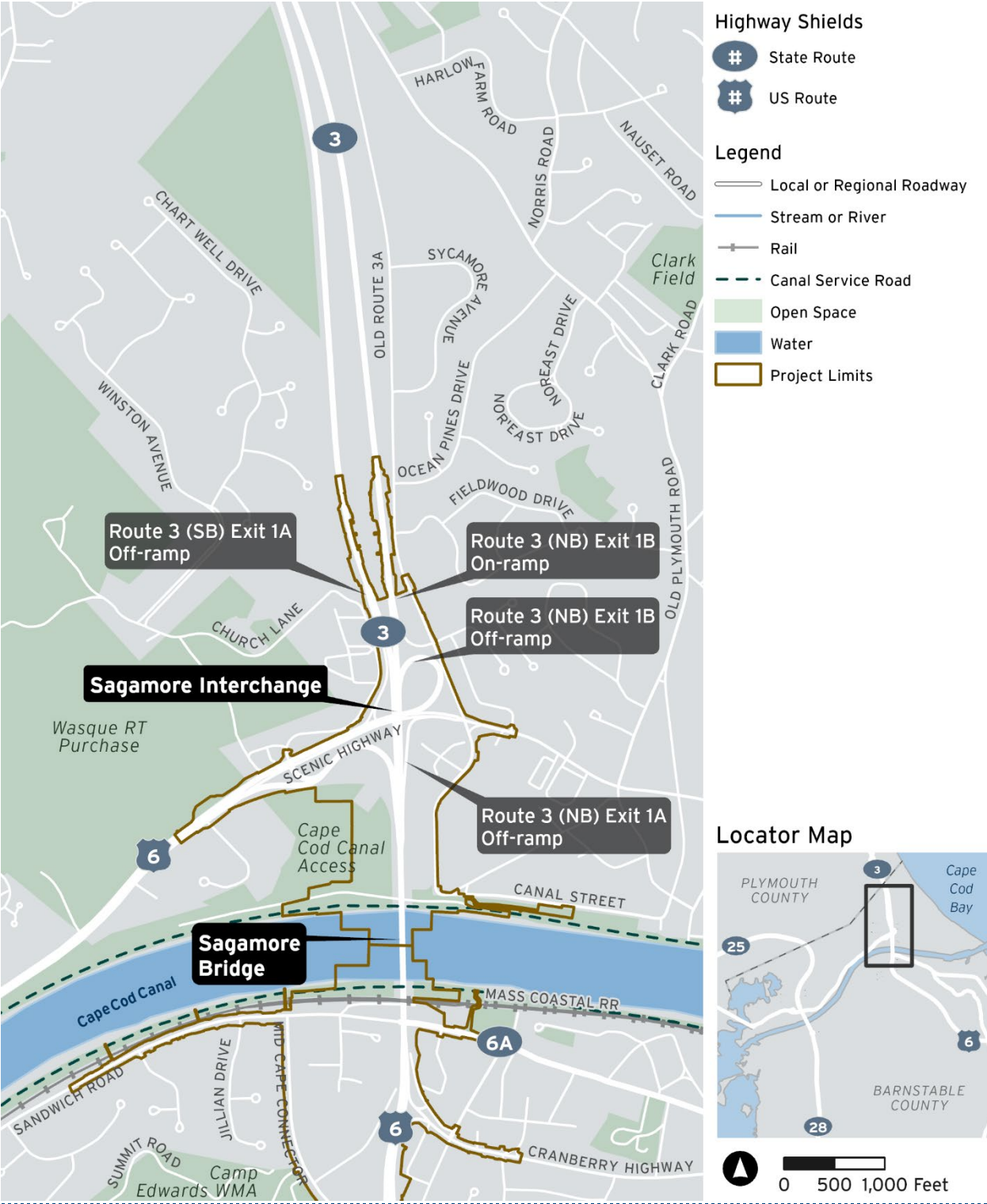
Figure 1-5. Sagamore Interchange
