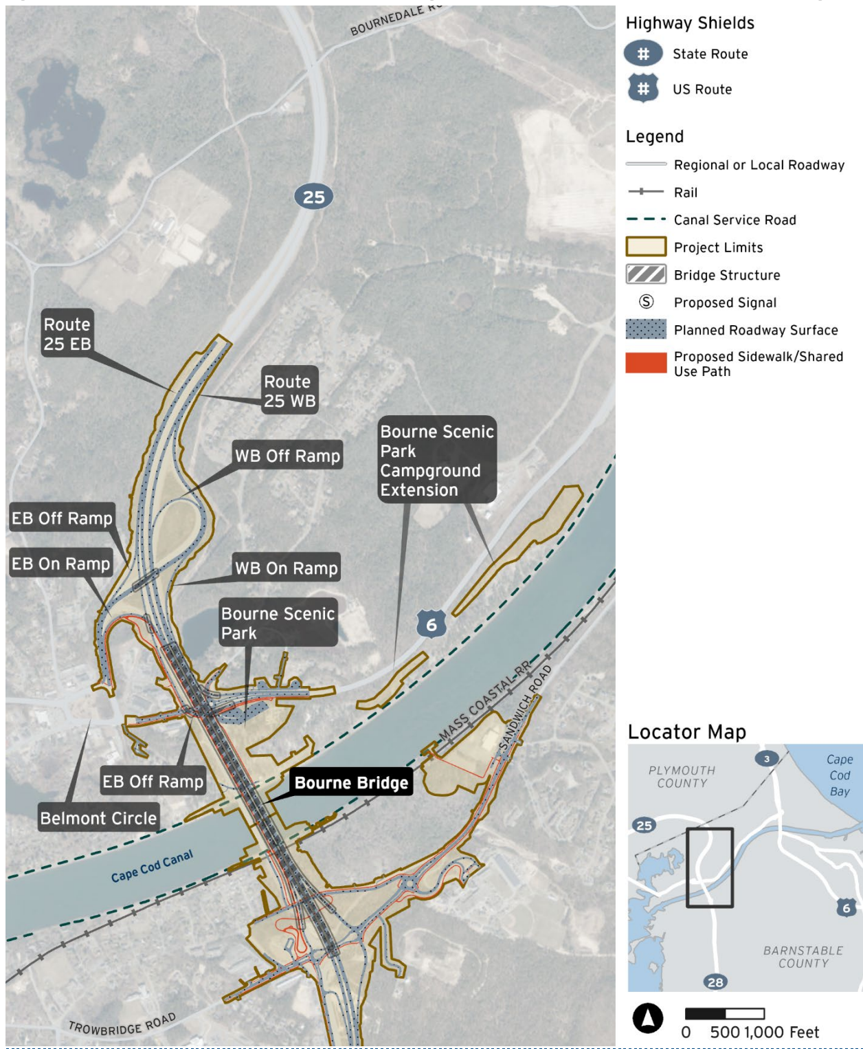
Figure 3-13. Bourne North Quadrant Crossing: Option BN-14.4b, Directional Interchange
