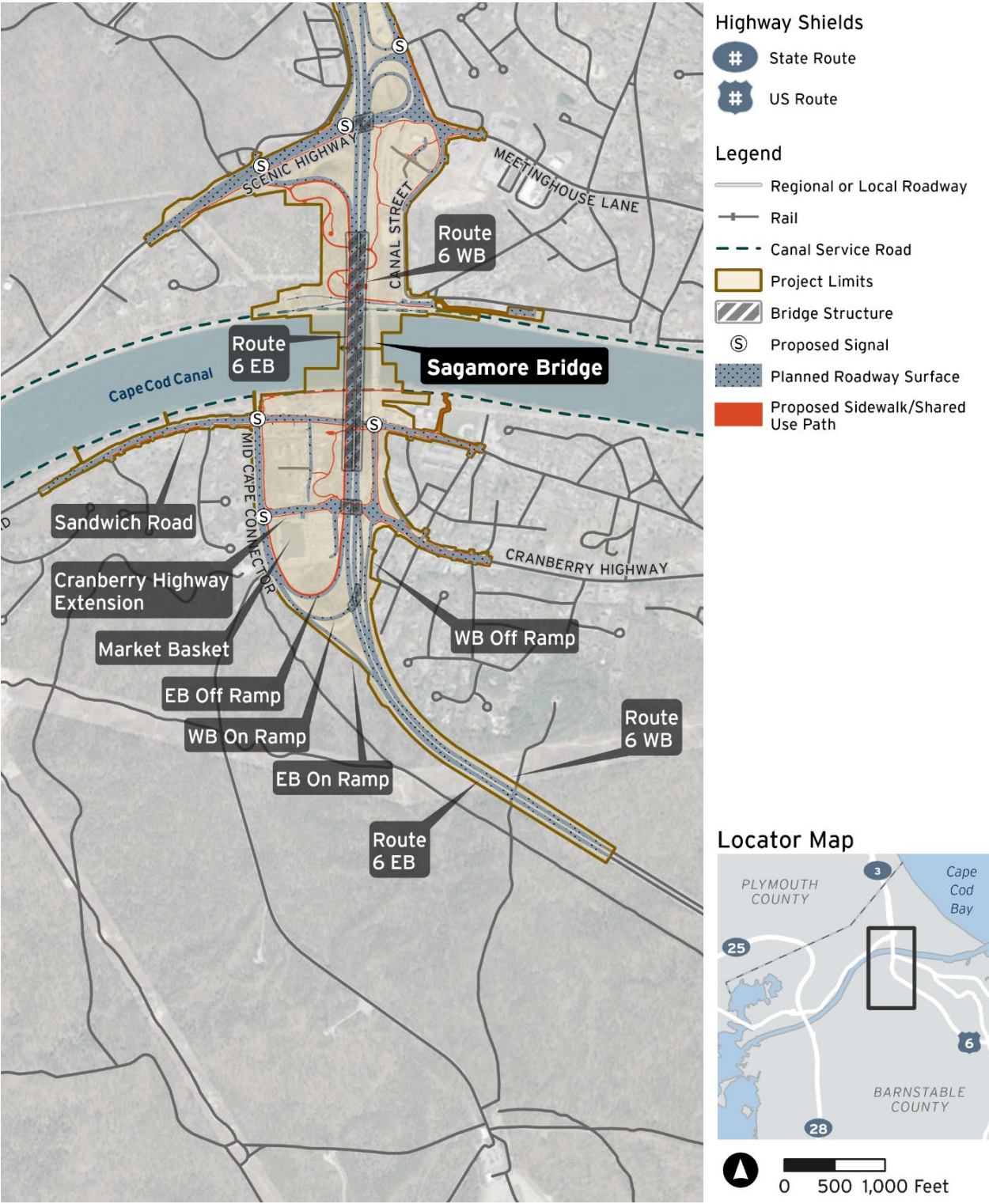
Figure 3-12. Sagamore South Quadrant Crossing: Option SS-3.1A, Westbound On-Ramp Under U.S. Route 6 with Sandwich Road Extension
