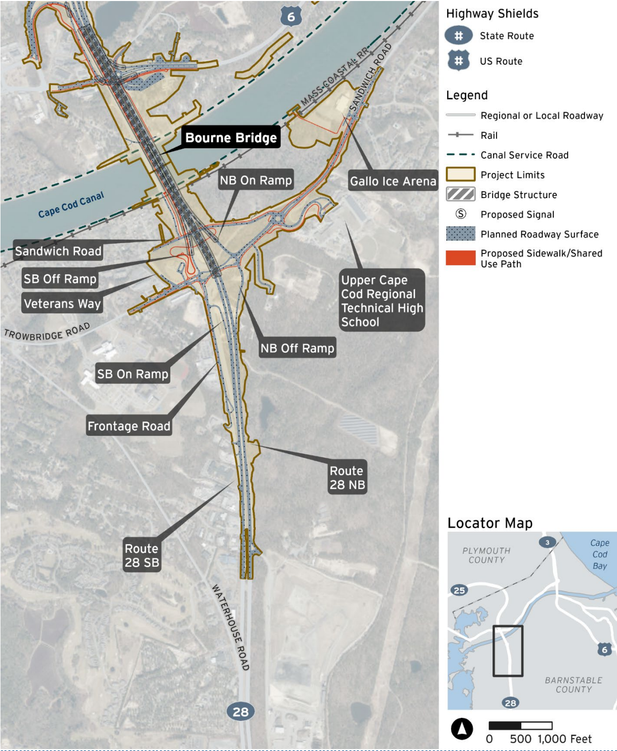
Figure 3-14. Bourne South Quadrant Crossing: Option BS-2, Diamond Interchange
