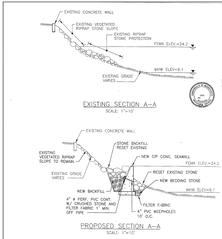
Figure 4.3. Cross sections of existing slope and proposed armoring with concrete seawall.
