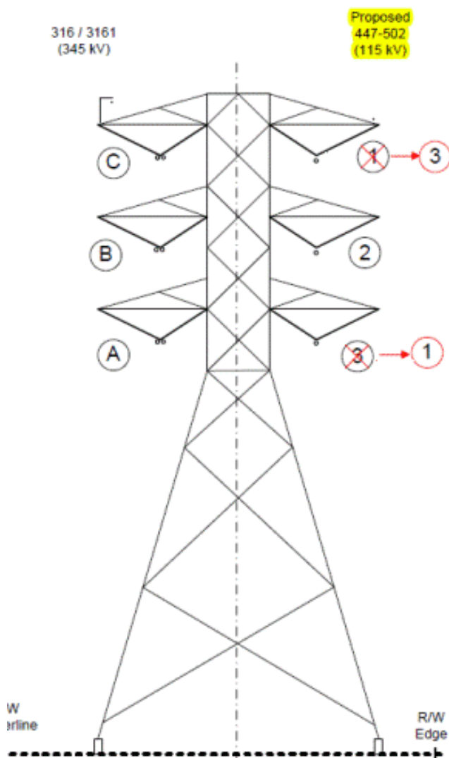
Fig. 2. Reverse Phasing, Line 447-502/510
