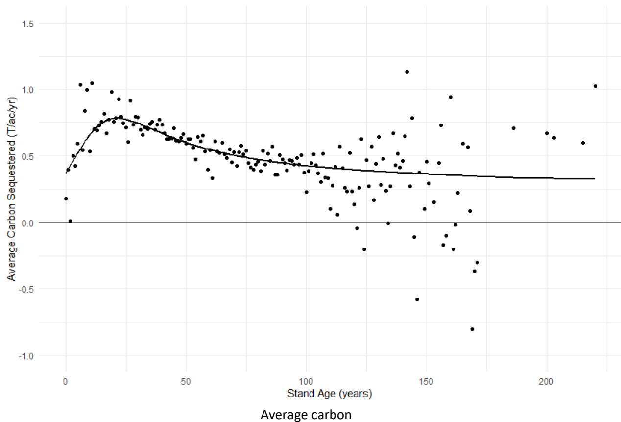
Figure 2. Live-tree carbon sequestration rate changes with stand age. Points represent the average net carbon sequestered for each stand age (one year increments) from FIA data for northeastern U.S. states, while the line represents the best fit model to the point data.
