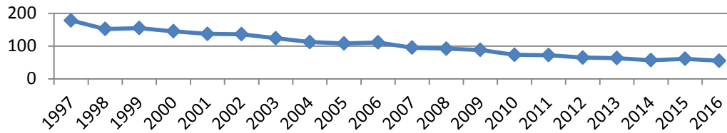
Average Reported Gallons of Perc Use by Year
