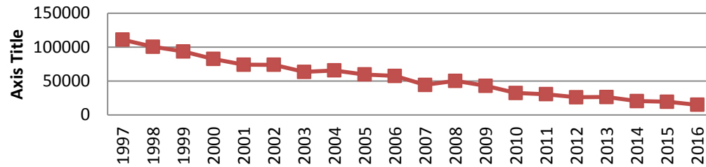
Average Reported Gallons of Perc Use by Year
