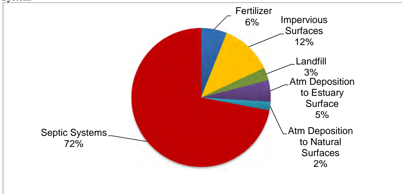
Figure 4: Percent Contribution of Nitrogen Sources to the Swan Pond River Estuarine System
