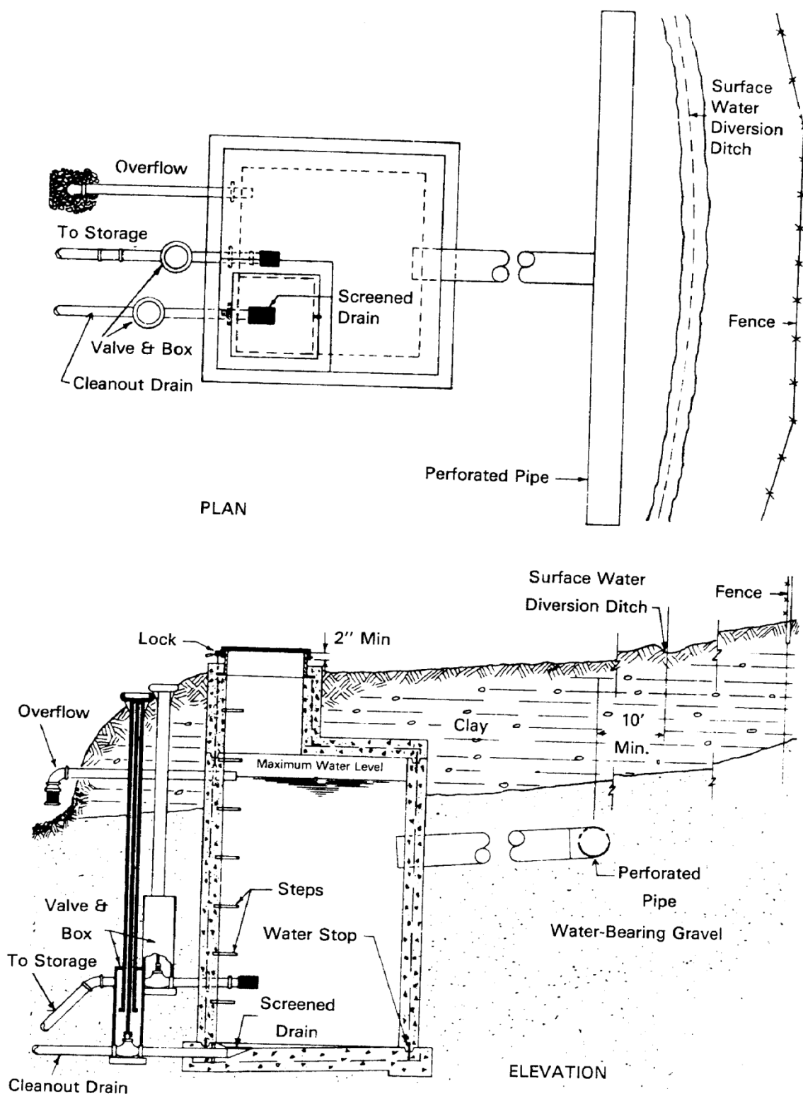
Figure 17. Spring Protection
