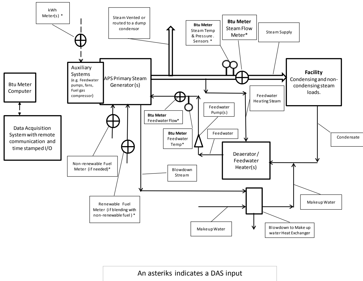
Figure 14. Simplified Schematic Diagram of a Generic RTGU Generating Steam Figure 14. Simplified Schematic Diagram of a Generic Large RTGU Generating Steam
