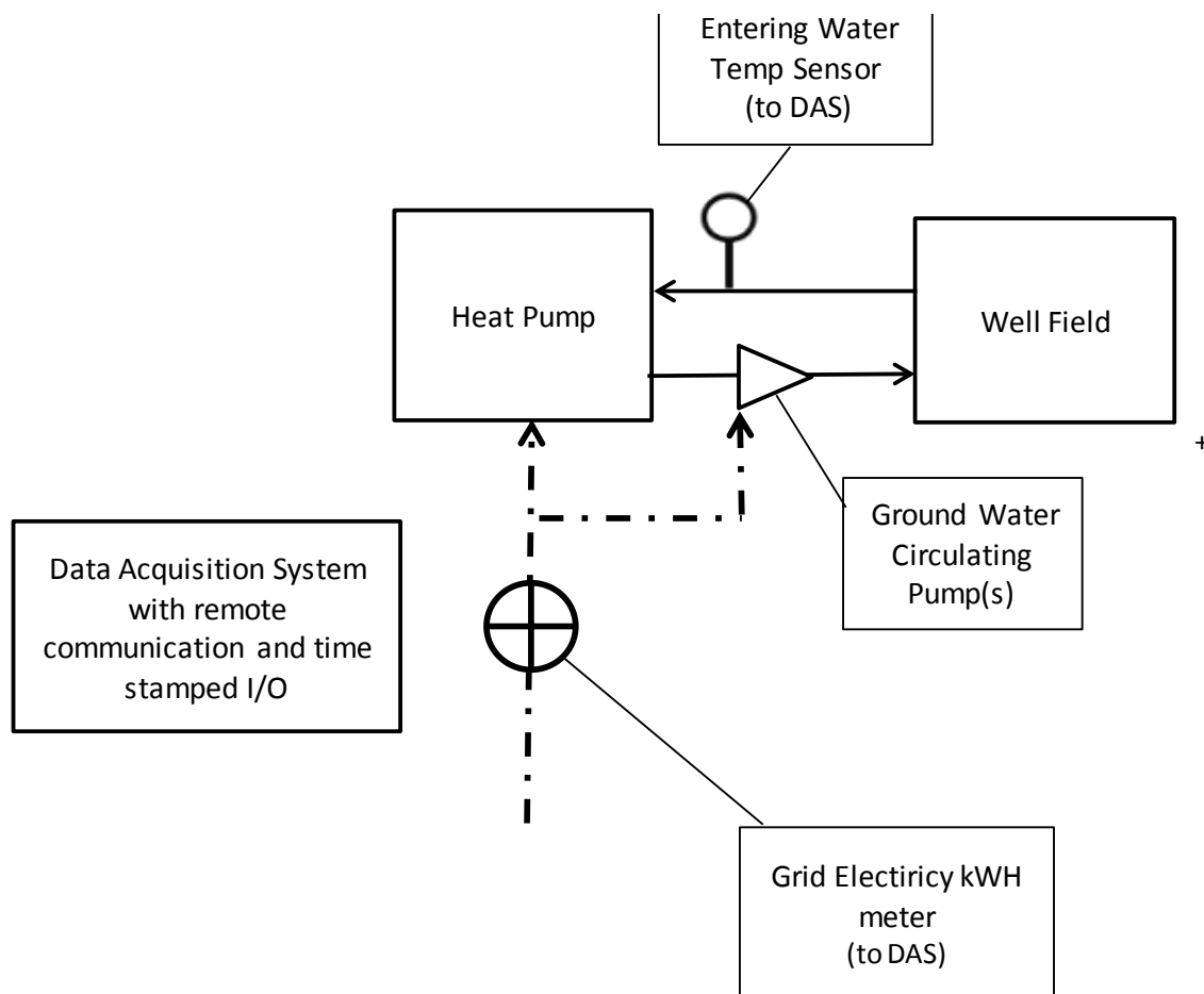
Figure 12. Metering Diagram for an Intermediate GSHP Figure 10. Metering Diagram for an Intermediate GSHP
