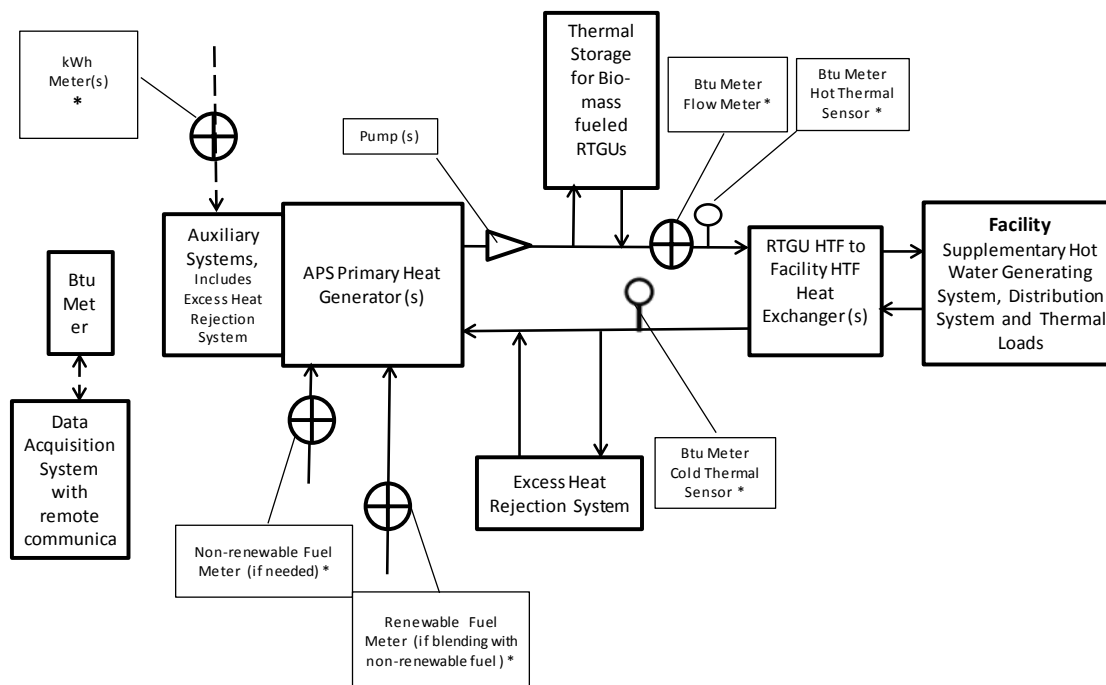
Figure 15. Metering Diagram for a Large Fired RTUG which Generates a Hot Heat Transfer Fluid
