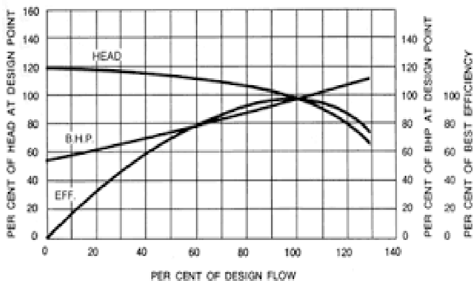
5) Figure 4. Example of a Typical Pump Curve with Showing the Design Operating Point
