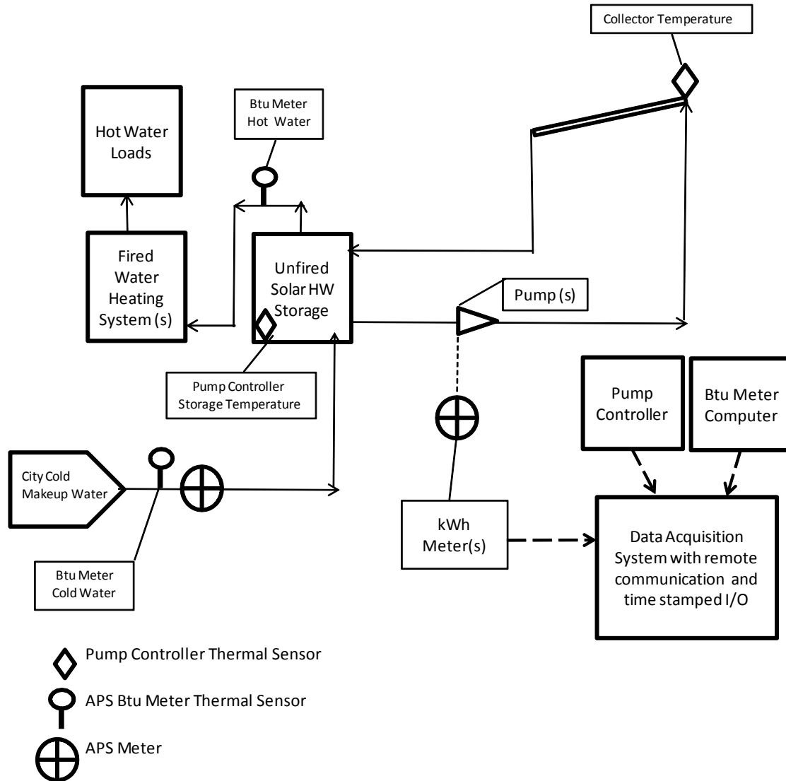
Figure 5. Simplified Schematic of a Typical Generic Large, Evacuated Tube , Solar Thermal RTGU
