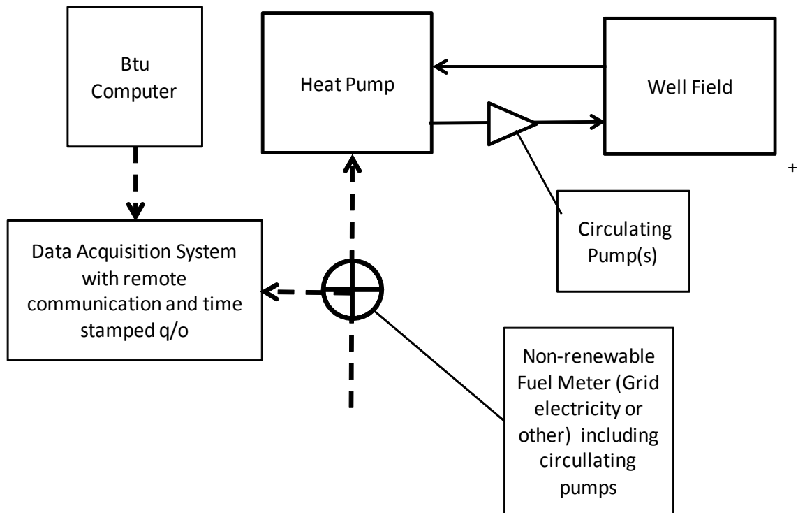
Figure 12. Metering Diagram for an Intermediate GSHP
