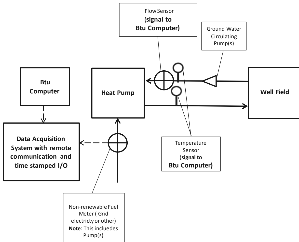
Figure 13. Metering Diagram for a Large GSHP
