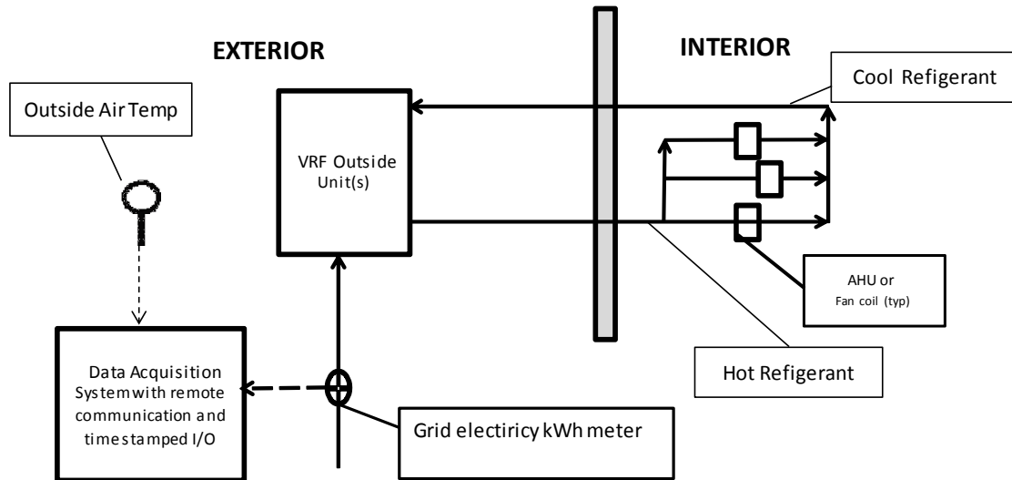
Figure 10. Metering Diagram for an Intermediate, VRF ASHP
