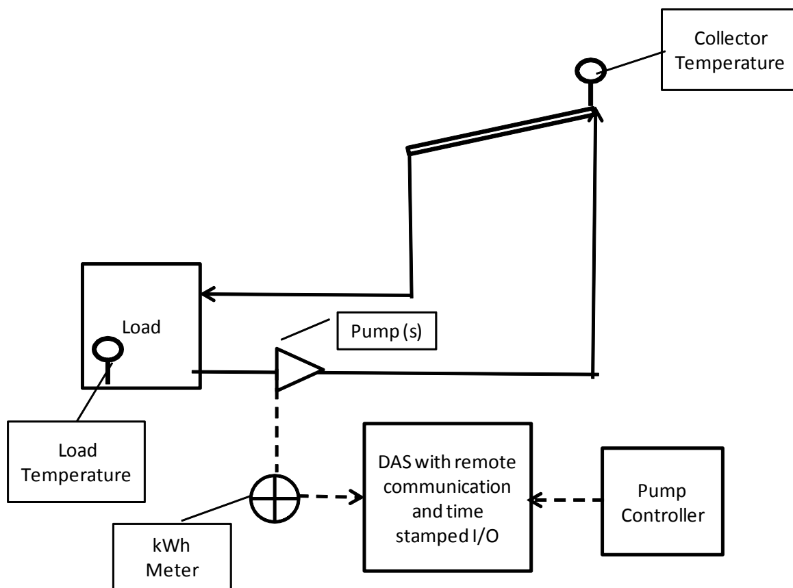
Figure 2. Simplified Schematic of a Typical Generic Intermediate Size, Evacuated Tube , Solar Thermal RTGU
