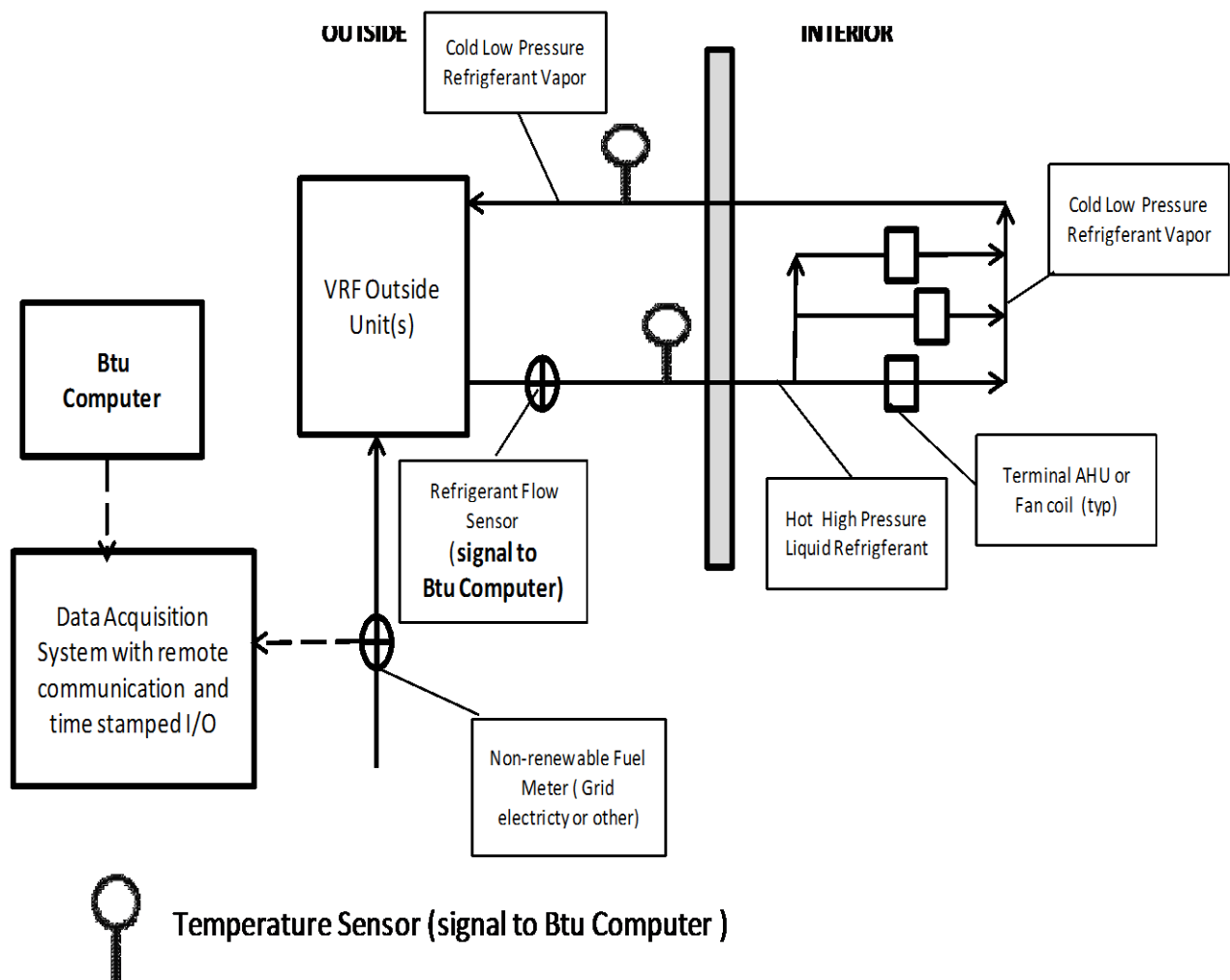
Figure 11. Metering Diagram for a Large, VRF ASHP
