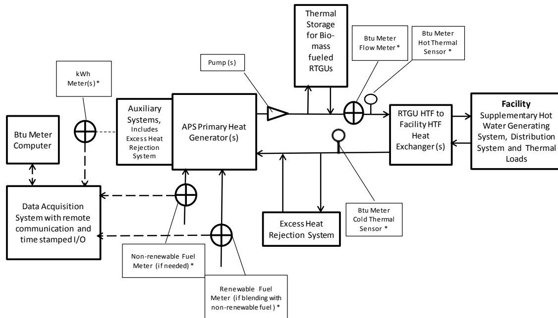
Figure 15-15. Metering Diagram for a Large Fired RTUG which Generates a Hot Heat Transfer Fluid
