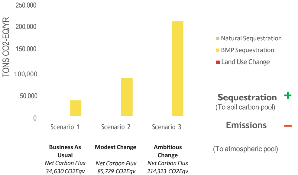
Figure 3.3 - Turf SOC Fluxes in Tons CO2-eq/yr. in 2050
