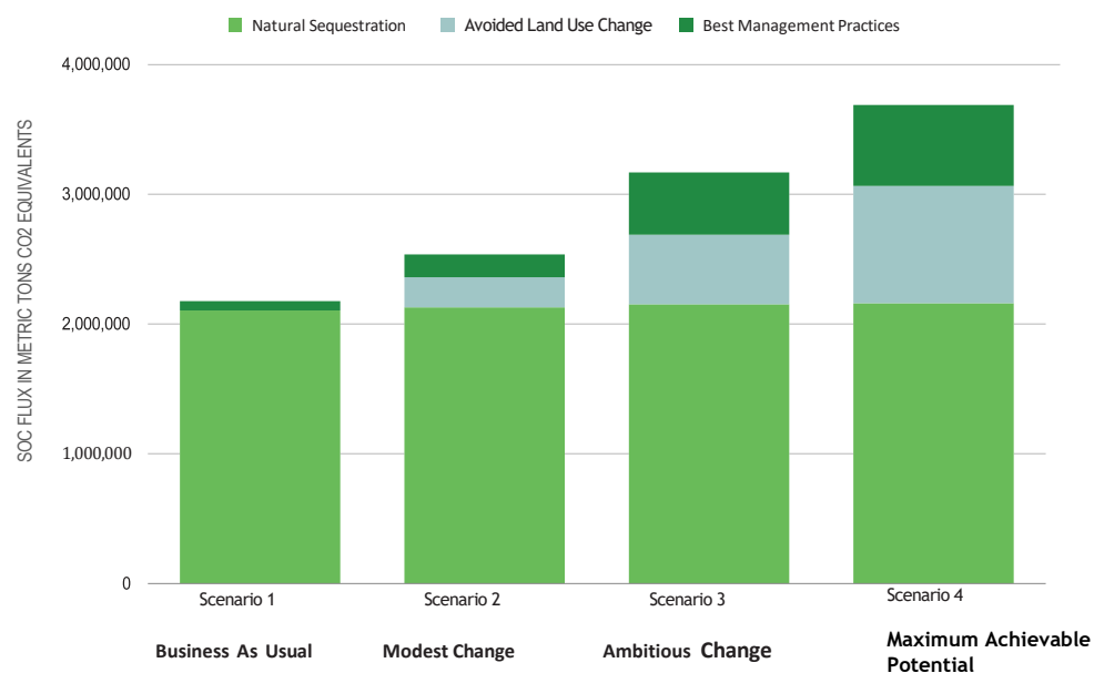
Figure 1.8 - Net SOC Flux Comparison in 2050: Technical Potential
