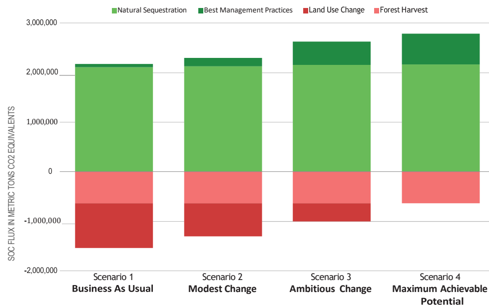
Figure 1.7 - Gain in Net SOC Flux in 2050: Technical Potential
