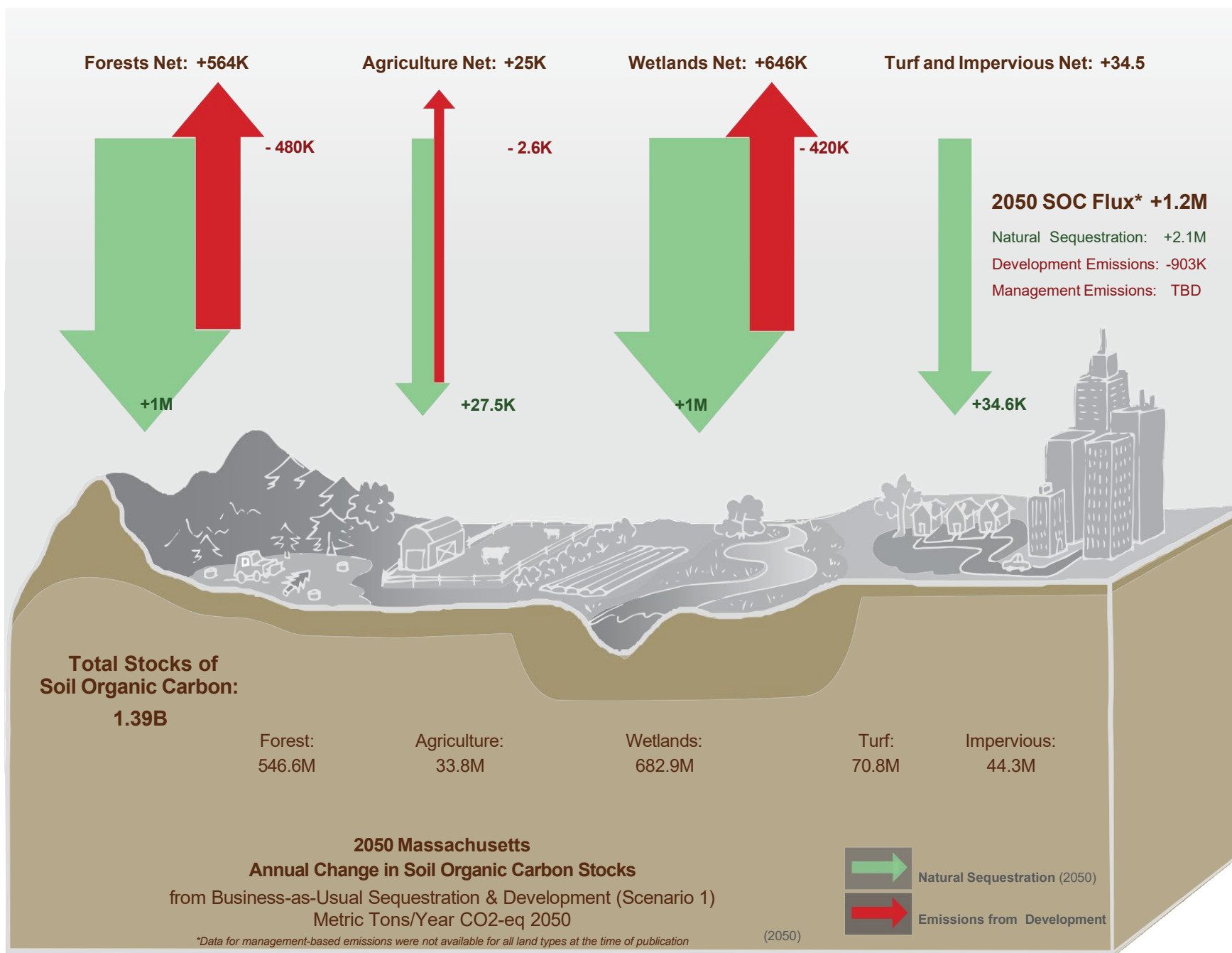
Figure 1.1 – 2050 Massachusetts Annual Change in Soil Carbon Stocks
