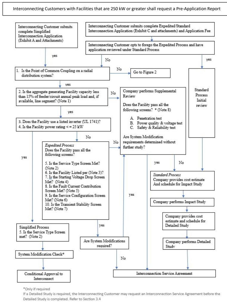
Figure 1. Schematic of Massachusetts DG Interconnection Process
