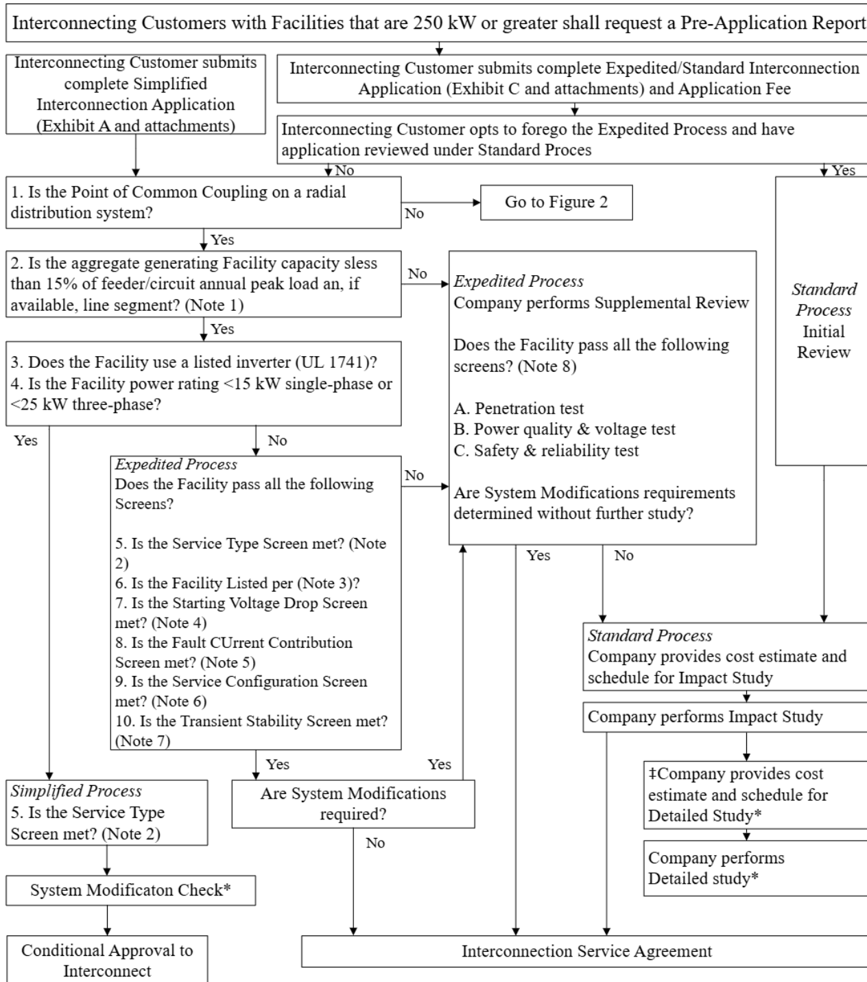
Figure 1 - Schematic of Massachusetts DG Interconnection Process
