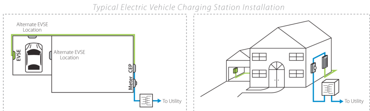
Figure 3-6. TYPICAL ELECTRIC VEHICLE SERVICE EQUIPMENT INSTALLATION.
