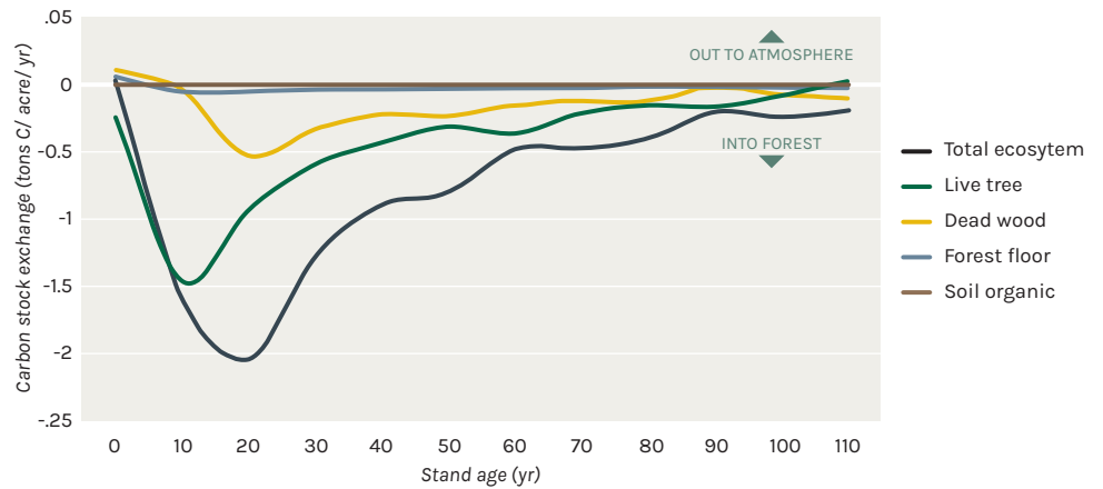
Figure 1. Carbon stock change by pool over 110 years following clear-cut harvest in Northeast Oak-hickory stands. 4
