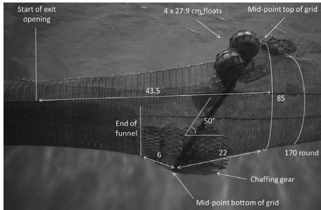
FIGURE 2 Structure and dimensions of the experimental trawl extension, including grid and escape window, during flume tank testing. Measurements are in number of meshes, unless otherwise specified (modified from Bayse, He, Pol, & Chosid, 2014)
