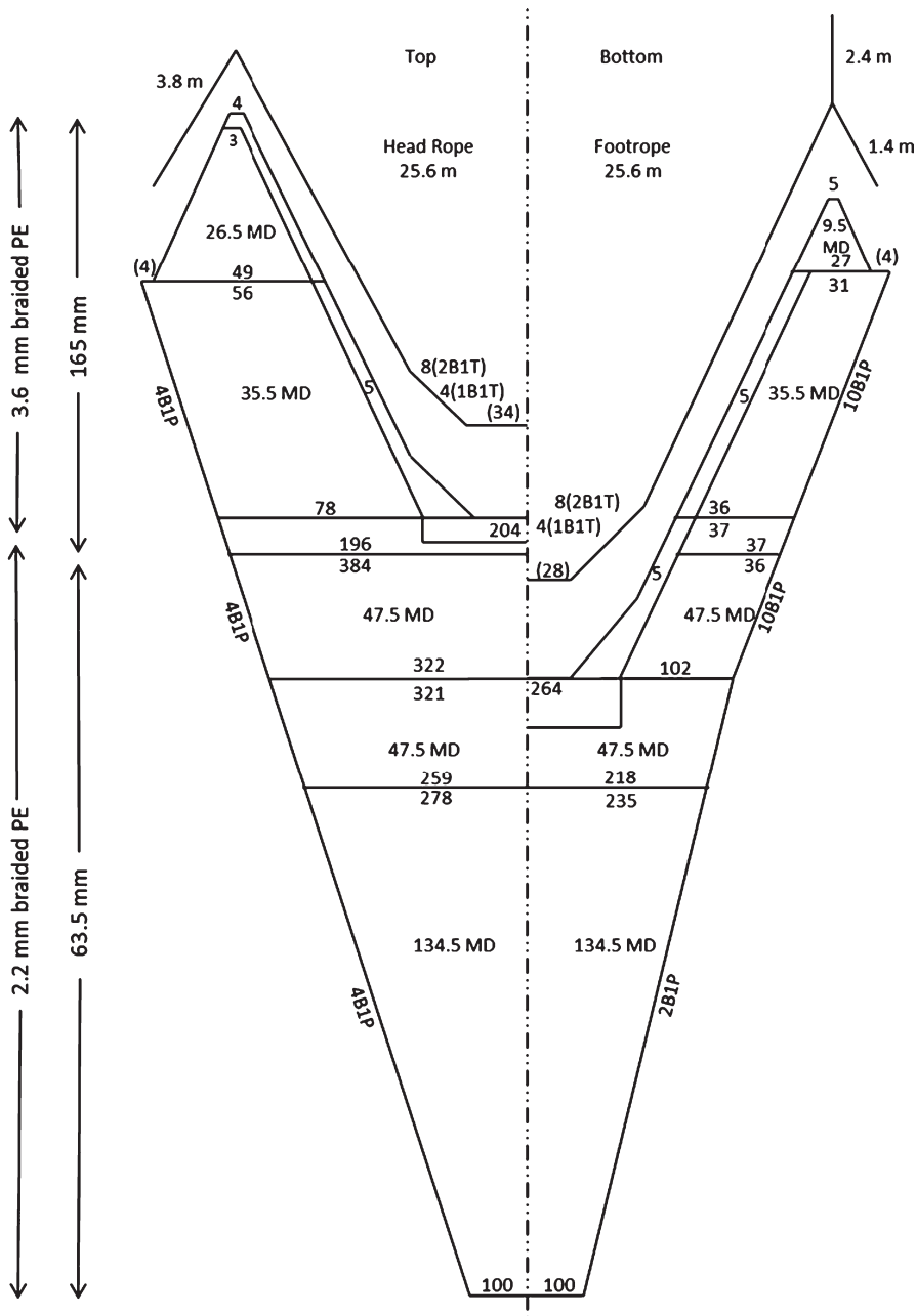
FIGURE 1 Net plan of trawl used. Measurements are in number of meshes unless otherwise noted (modified from Bayse, Pol, & He, 2016)
