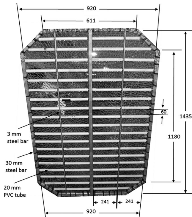
FIGURE 3 Structure and dimension of grid. Measurements are in mm (modified from Bayse, He, Pol, & Chosid, 2014)
