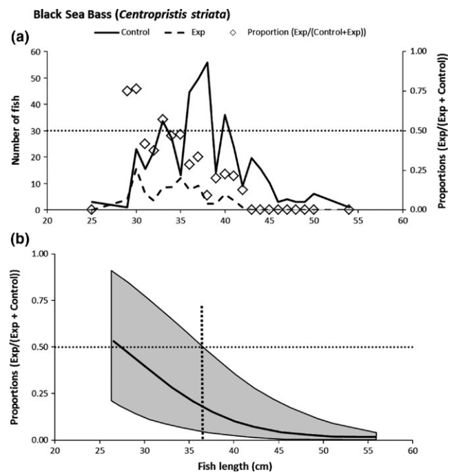
FIGURE 7 (a) Pooled length frequencies of black sea bass and observed proportions exp/(exp + control). (b) Generalized linear mixed model (GLMM) of modeled proportions of black sea bass catch at length caught in the trawl with a species-separator grid (experimental). The vertical dotted line displays the length where a significant difference occurs
