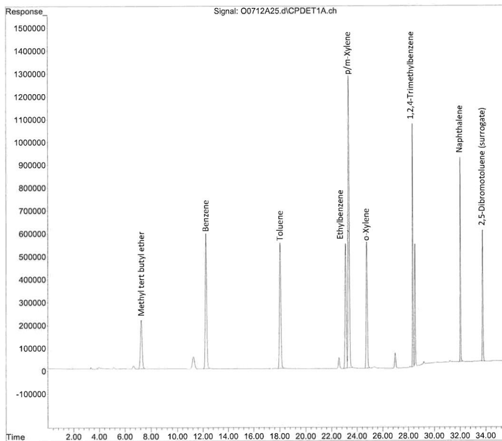
Figure 2. PID Chromatogram
