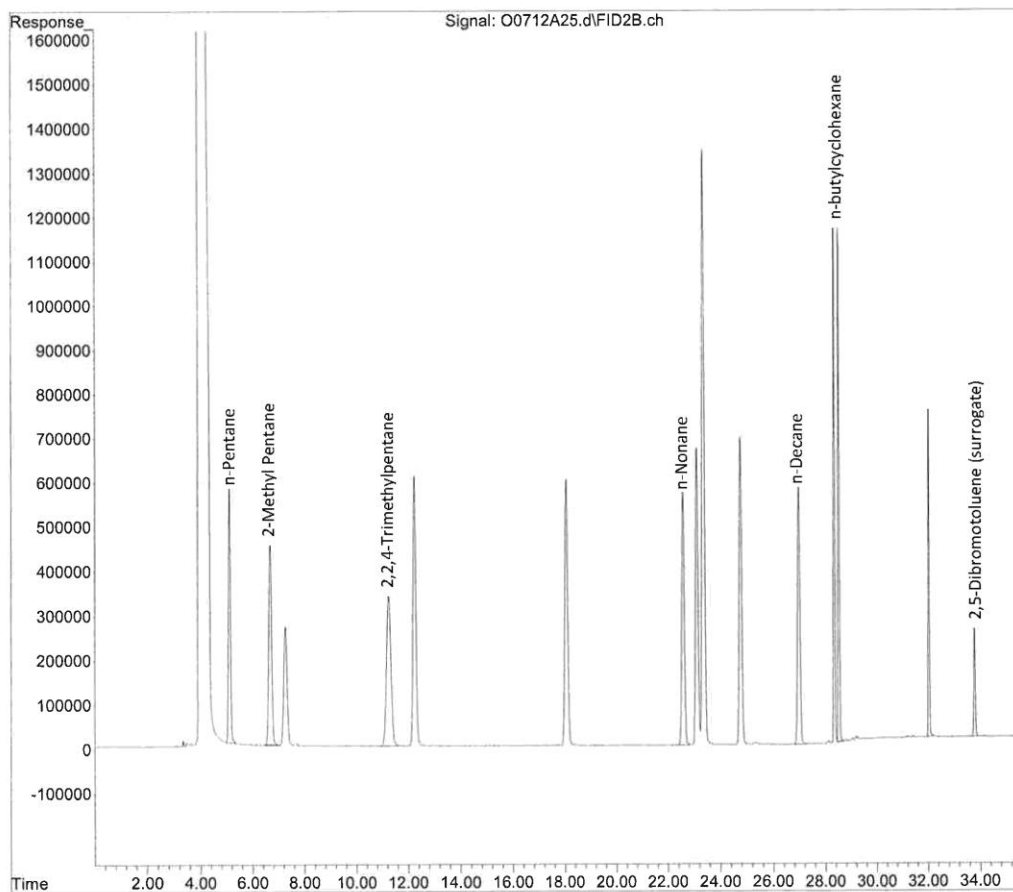
Figure 1. FID Chromatogram
