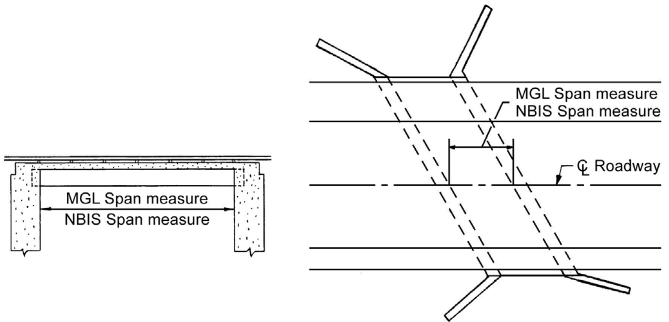
Figure 2c: Bridges without Defined Centerlines of Bearings
