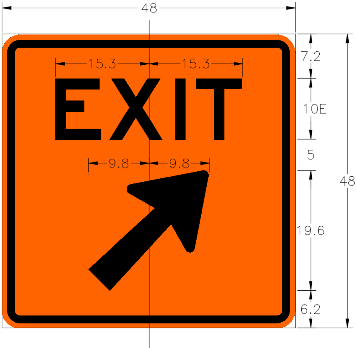
MA-E5-1wz EXIT GORE (WORK ZONE)
