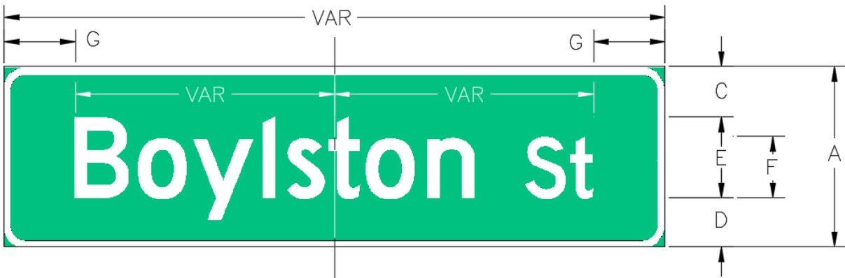
MA-D3-1 WITH DESCENDING STROKES
