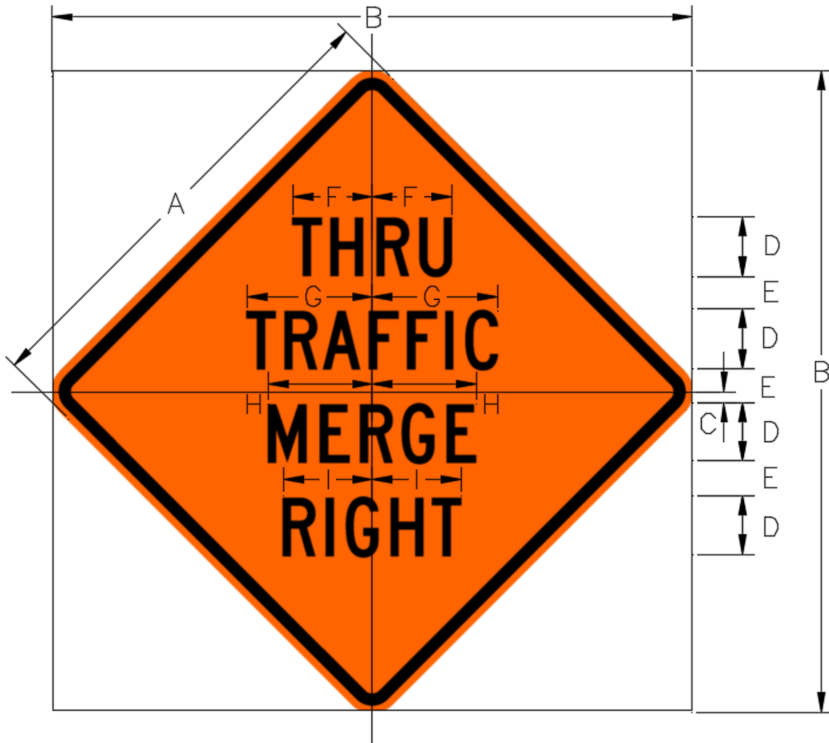
MA-W4-7R THRU TRAFFIC MERGE RIGHT
