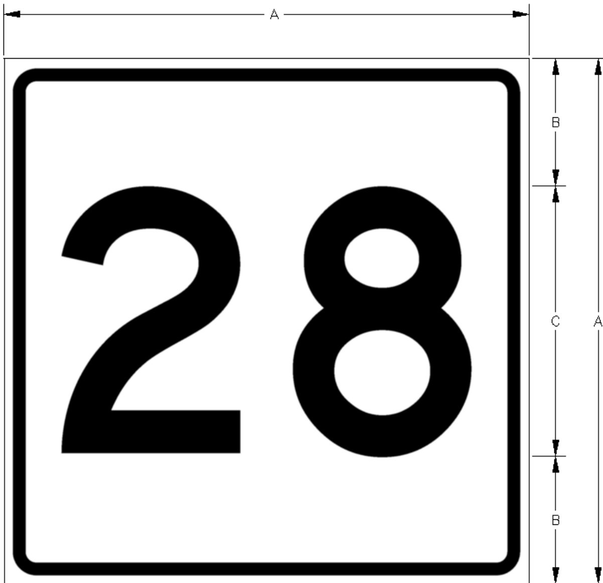
MA-M1-5 (1 OR 2 DIGIT) STATE ROUTE SIGN
