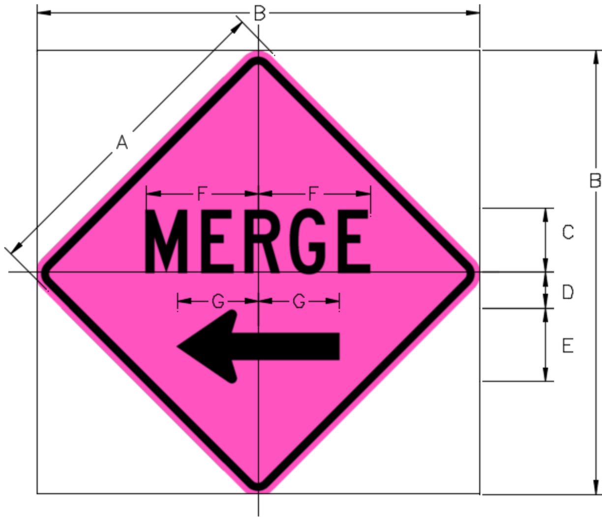
MA-W4-2aL/R MERGE LEFT/RIGHT
