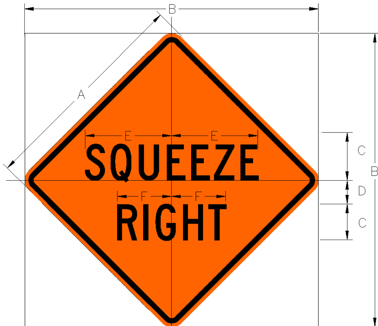
MA-W30-8R SQUEEZE RIGHT
