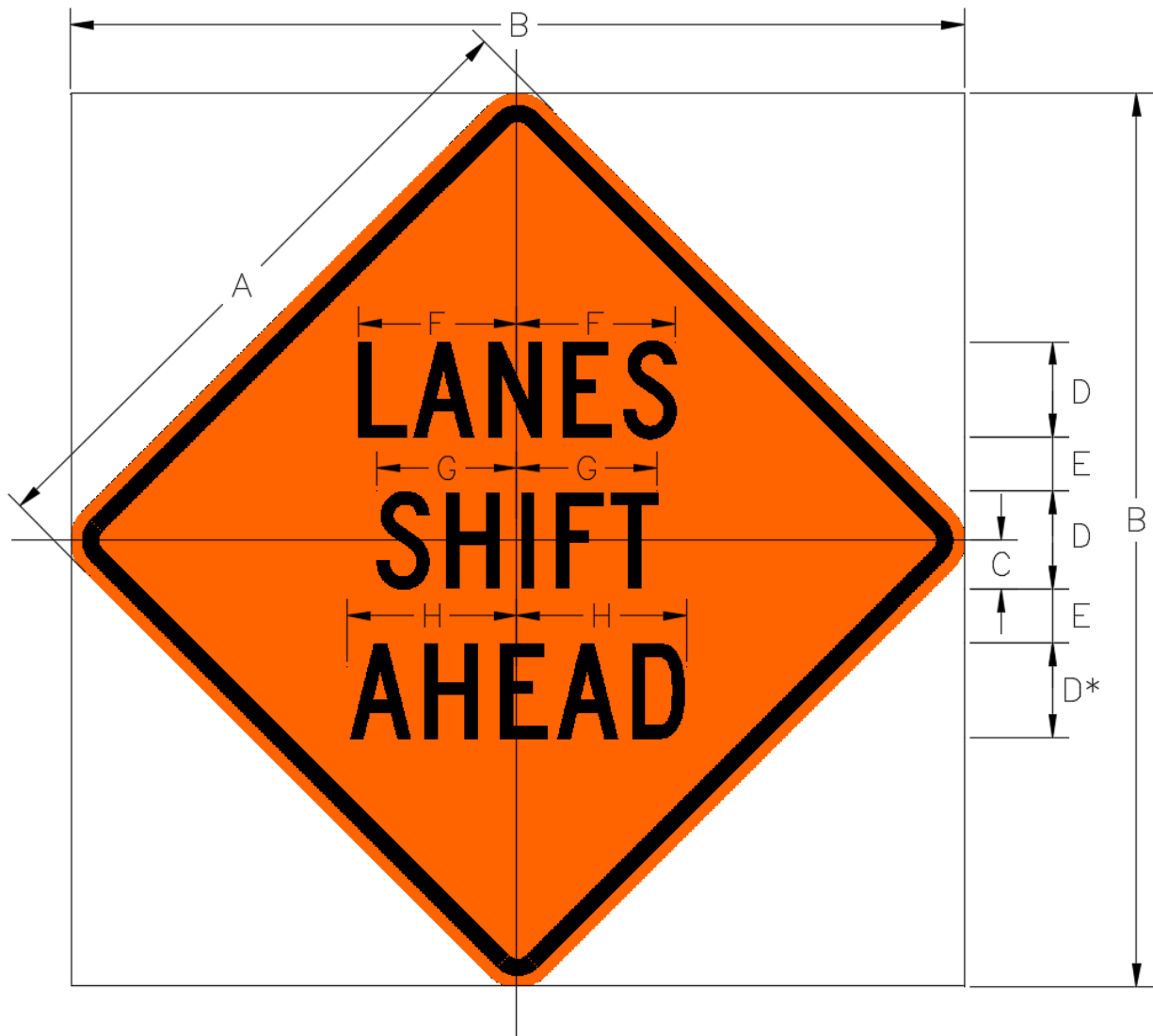
MA-W24-2 LANES SHIFT AHEAD
