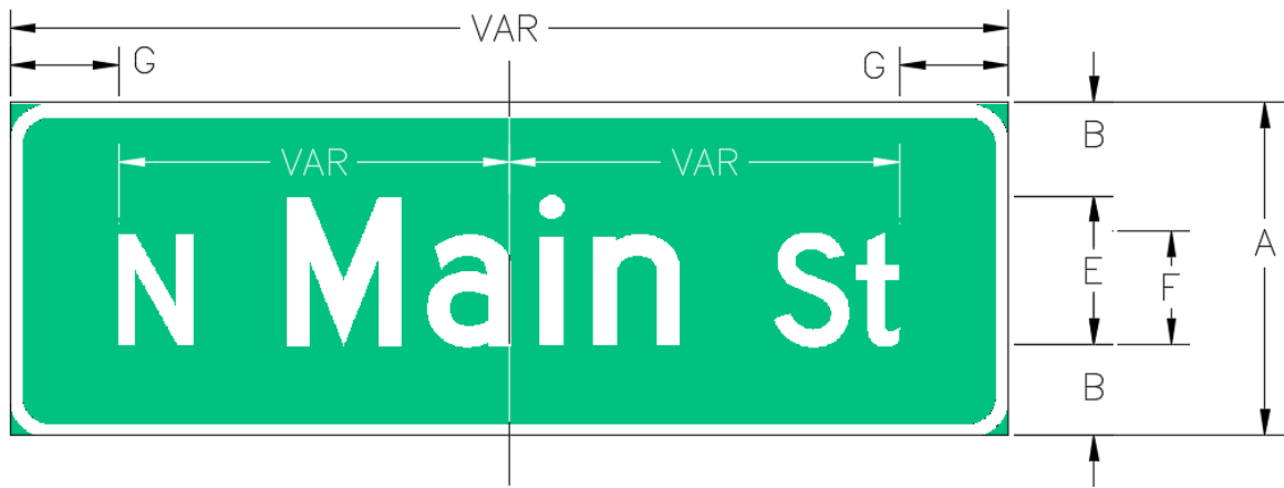
MA-D3-1 WITHOUT DESCENDING STROKES
