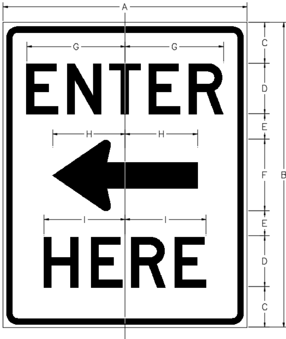
MA-R4-25 ENTER HERE
