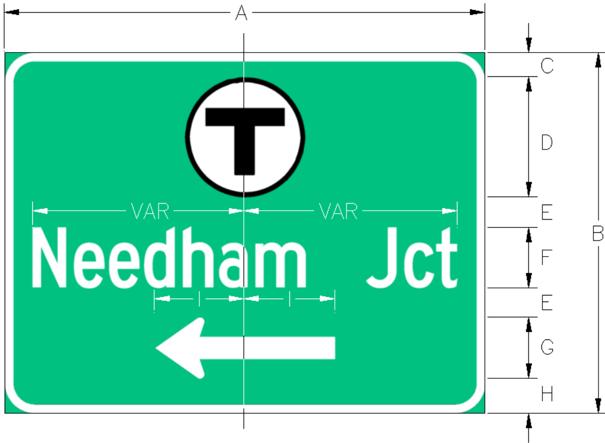
MA-D1-5 (T) DIRECTIONAL, MBTA STATION
