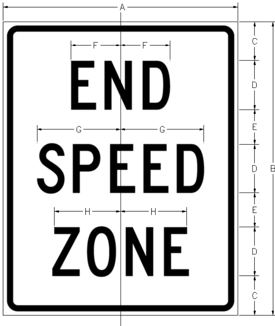
MA-R2-7 END SPEED ZONE
