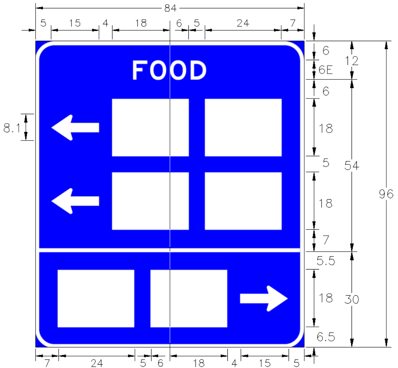
MA-D9-20a**, Sheet 1 of 2 EXIT RAMP, SPECIFIC SERVICES (TWO COLUMNS)
