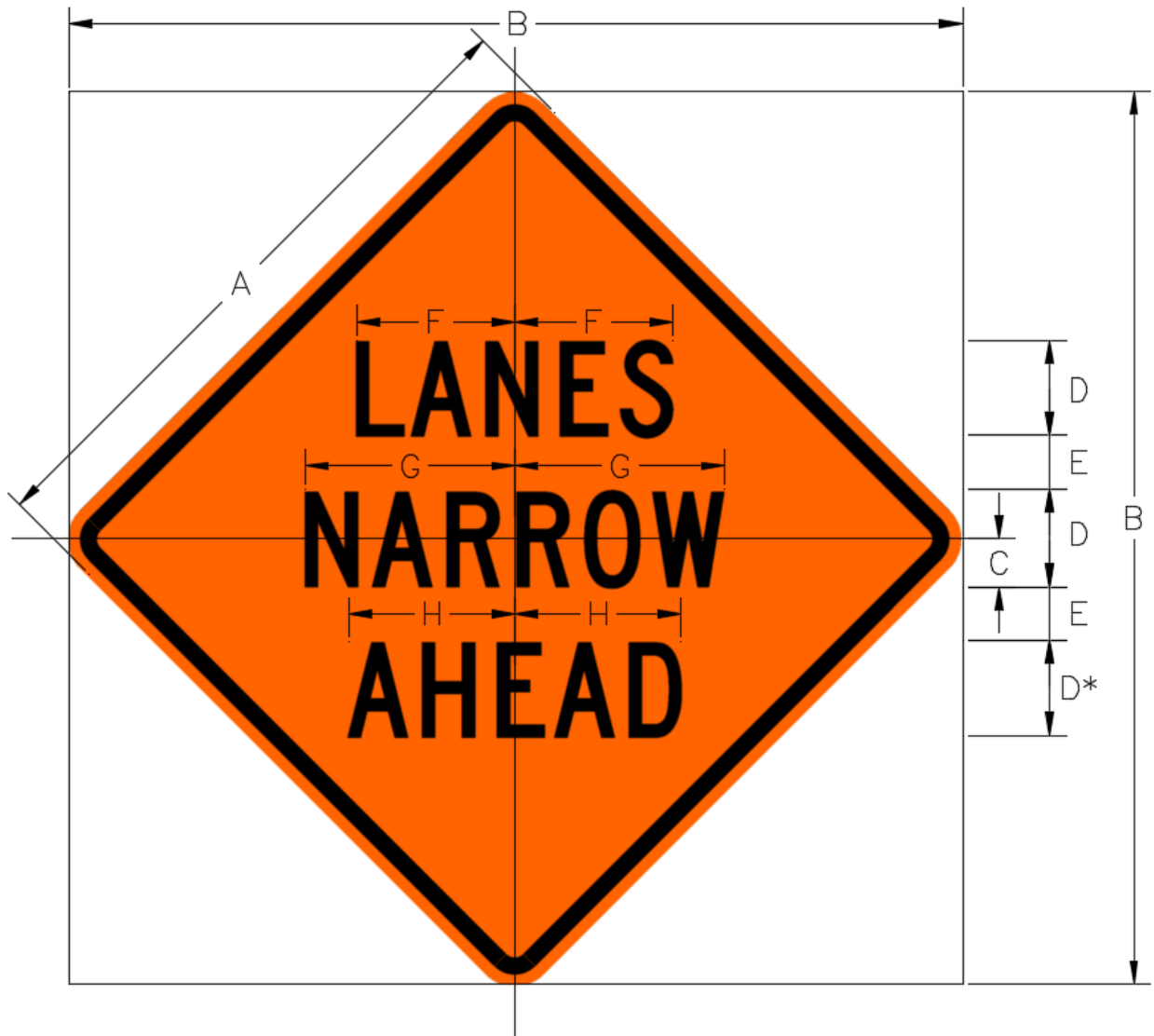
MA-W5-5 LANES NARROW AHEAD
