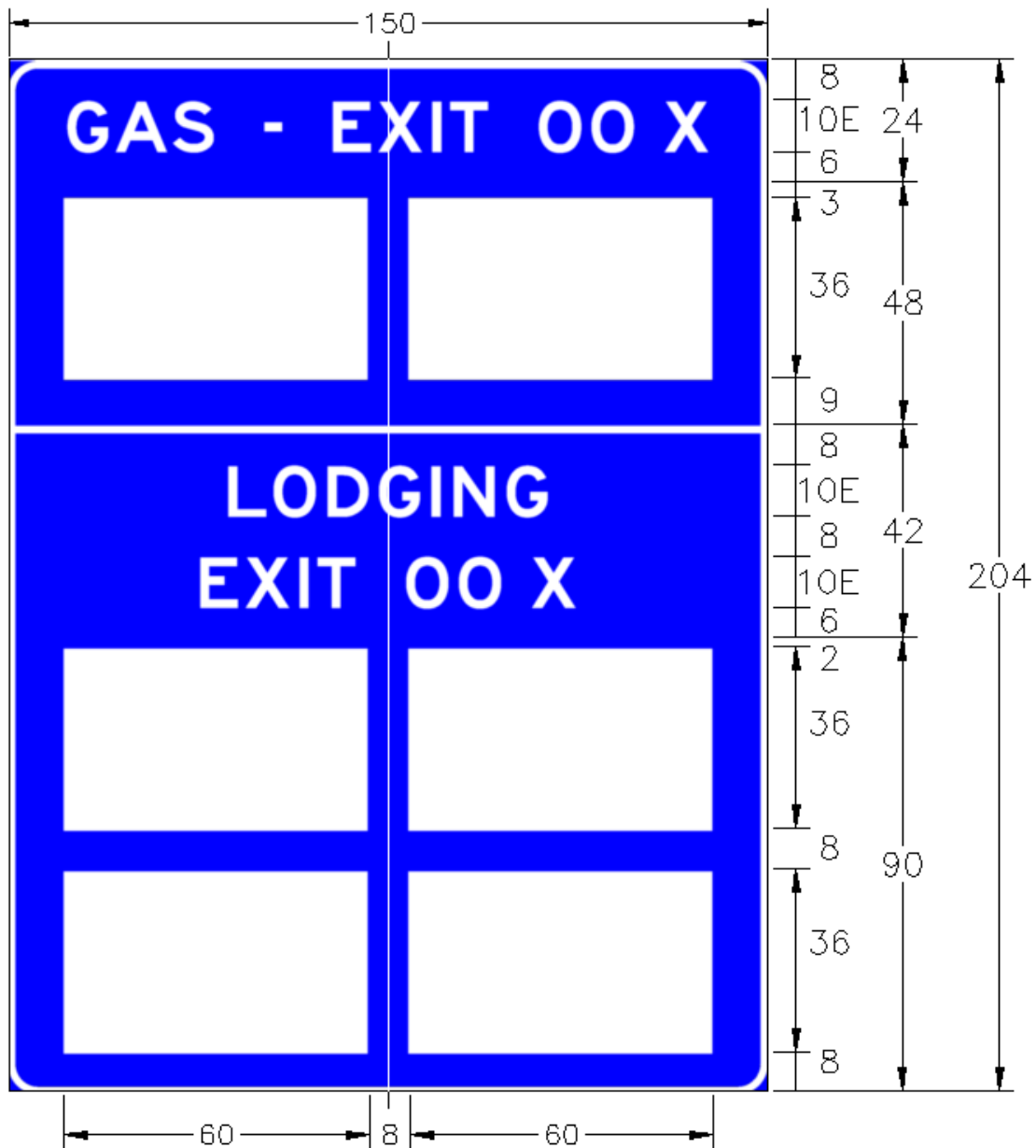
MA-D9-19c**, Sheet 1 of 2 MULTI-EXIT INTERCHANGE, SPECIFIC SERVICES
