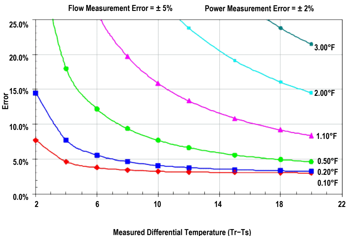
Figure 5-2. Example Influence of Sensor Accuracy on Calculations. 23
