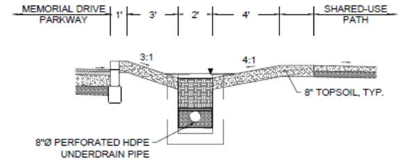
TYPICAL BIOSWALE DETAIL
