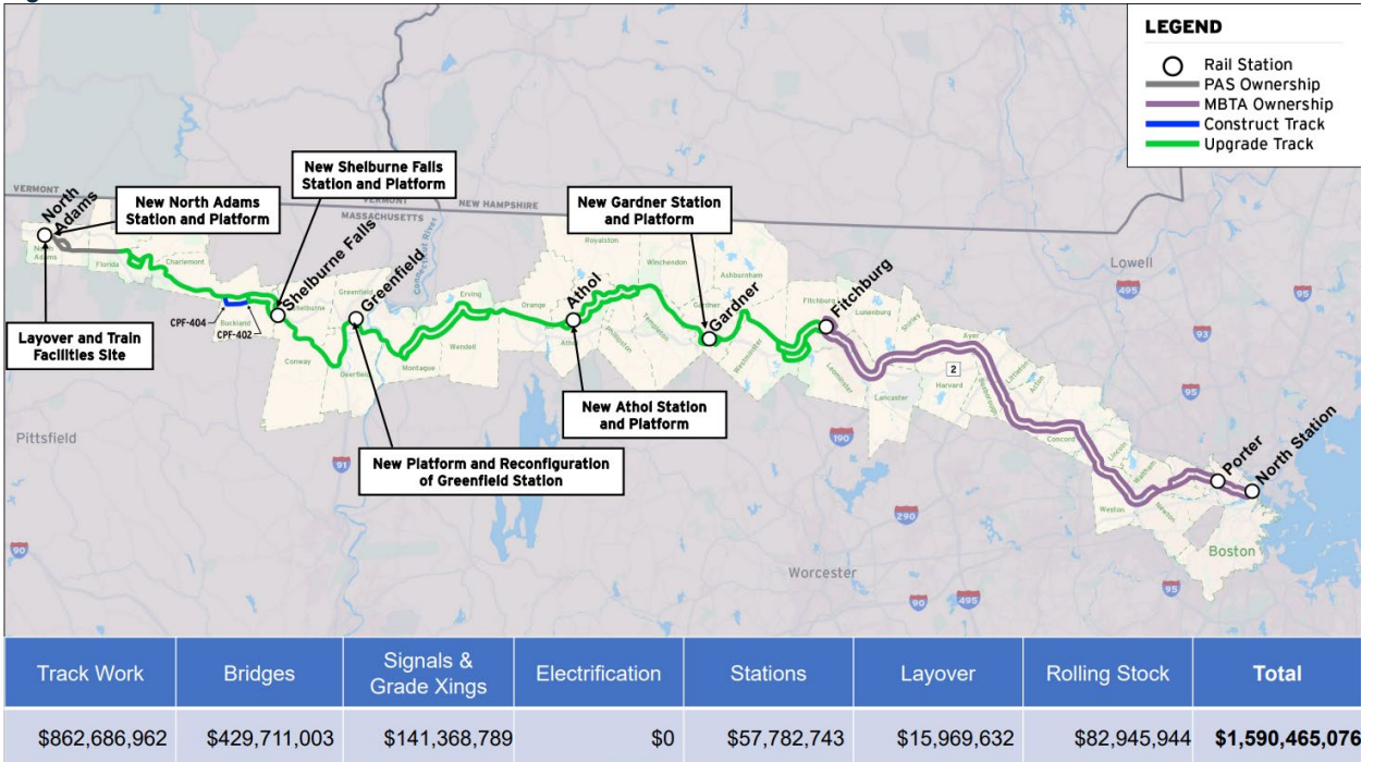
Figure 4.25: Alternative 4 – Full Local Service
