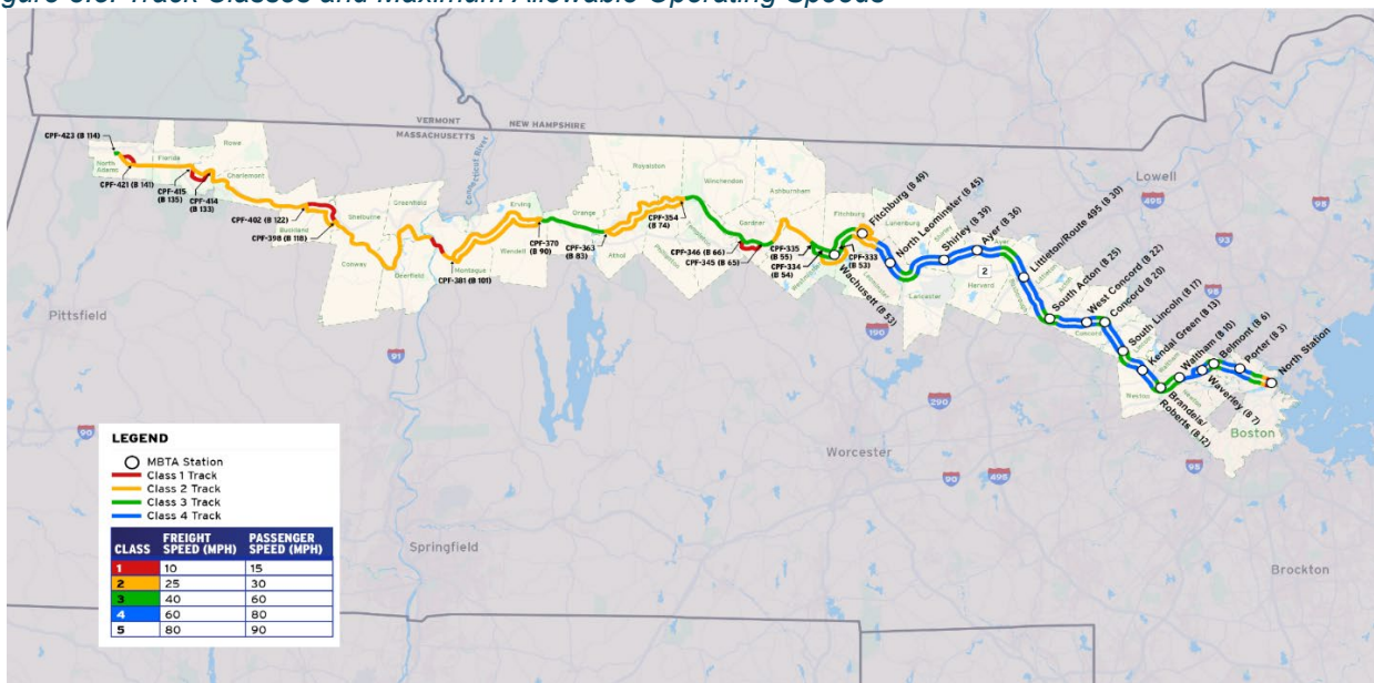
Figure 3.5: Track Classes and Maximum Allowable Operating Speeds
