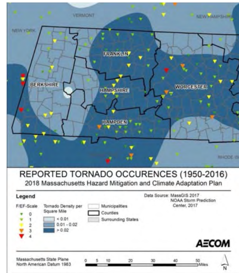
Figure 3.36: Density of Reported Tornadoes per Square Mile
