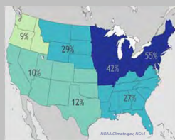
Observed Increase in Heavy Precip. 1958-2016
