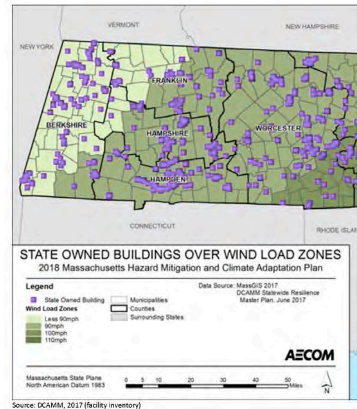
Fig. 3.25. Wind Load Zones for Massachusetts According to MA State Building Code
