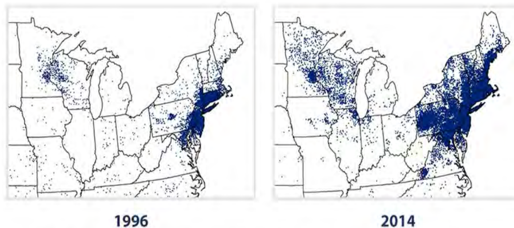
Fig. 3.32. Reported Lyme Disease Cases in 1996 and 2014
