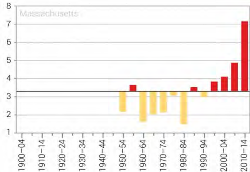
Fig. 3.18. Number of Nights When Temperatures Remain 70°F or Higher
