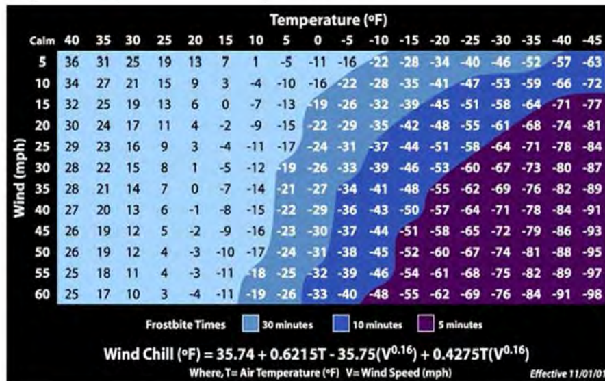
Fig. 3.19. Wind Chill Temperature Index and Frostbite Risk
