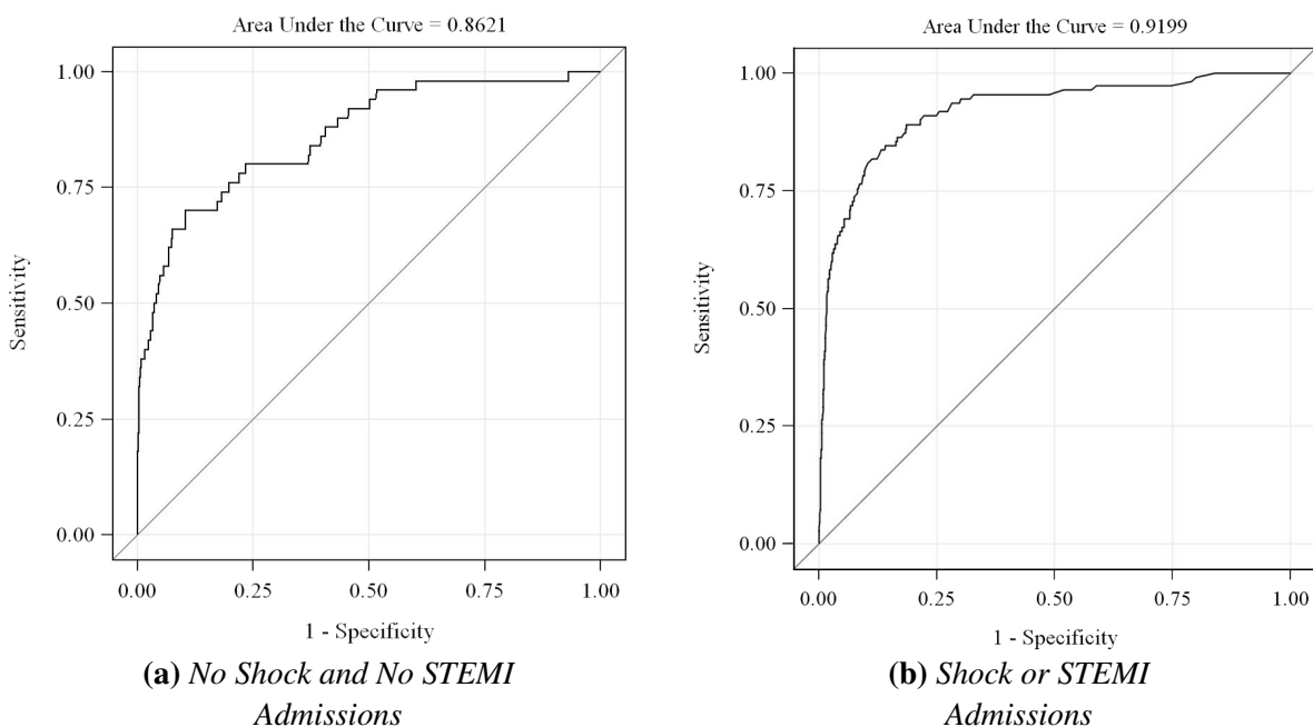
Figure 7.1: ROC Curve-Hierarchical
