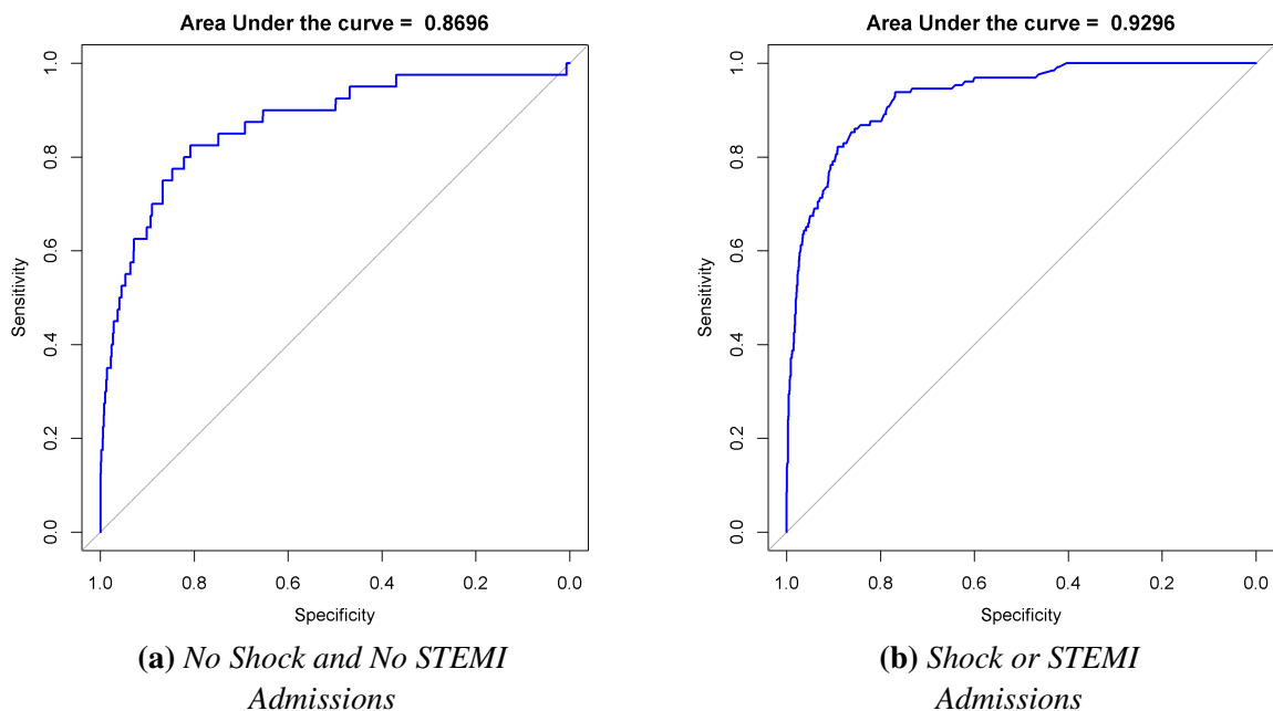
Figure 7.1: ROC Curve-Hierarchical
