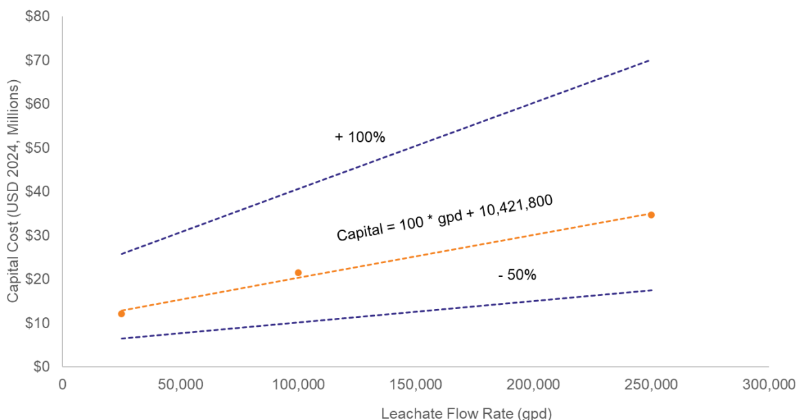
Figure 3-29. Project Capital Cost Curve with Estimating Range (-50% to +100%) for Installation of Reverse Osmosis
