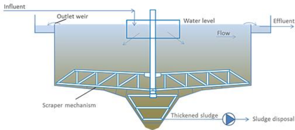
Figure D- 1. Gravity thickener
