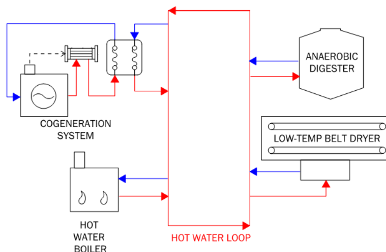
Figure D- 18. Representative Low Temperature, Indirect-Fired Belt Dryer Tied into a Plantwide Heat Loop
