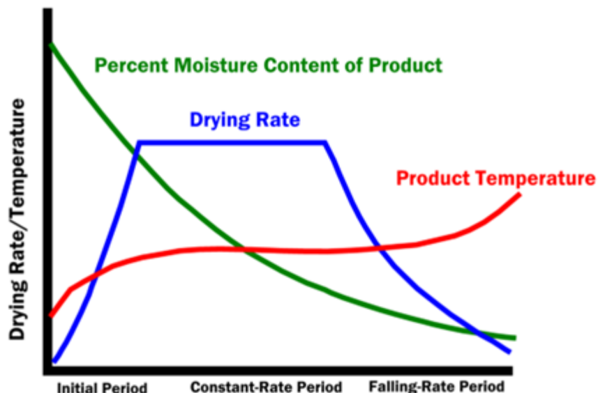
Figure D- 11. Thermal Drying Process Curve Over Time.
