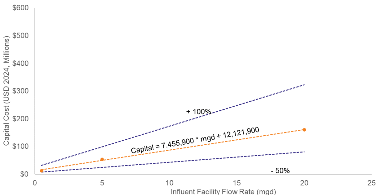
Figure 3-1. Project Capital Cost Curve with Estimating Range (-50% to +100%) for Installation of GAC
