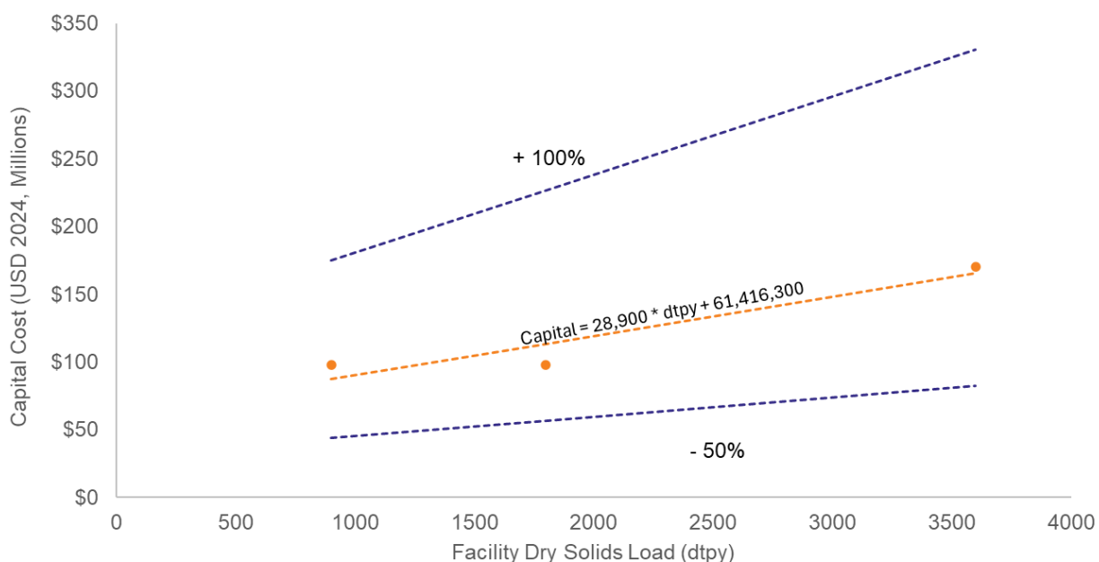
Figure 3-18. Project Capital Cost Curve with Estimating Range (-50% to +100%) for Installation of Gasification Systems
