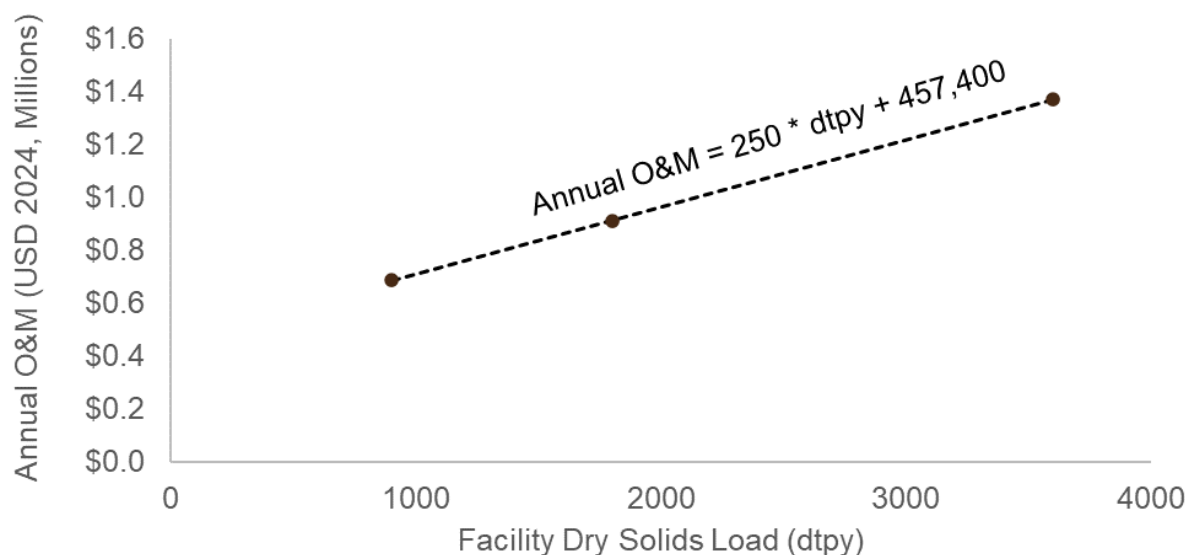
Figure 3-21. Annual Estimated O&M Cost Curve of Pyrolysis Systems
