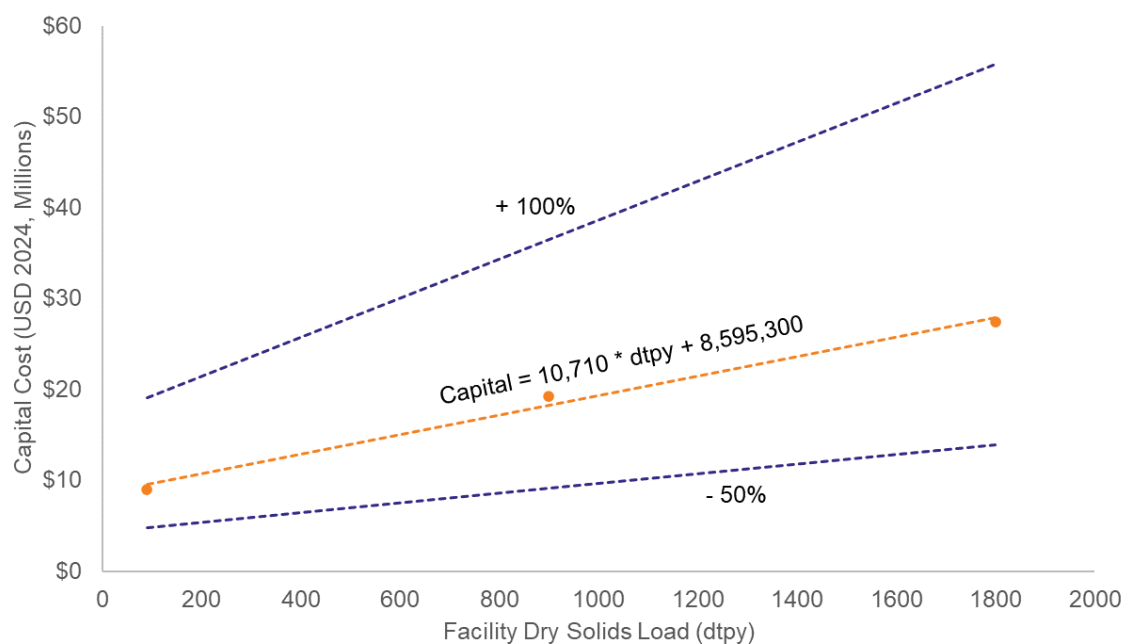
Figure 3-8. Project Capital Cost Curve with Estimating Range (-50% to +100%) for Installation of Screw Presses
