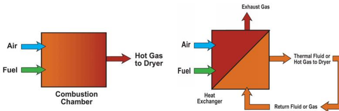
Figure D- 13. Direct And Indirect-Fired Process Heating System Illustrations, Show Respectively Direct-fired Belt Dryers
