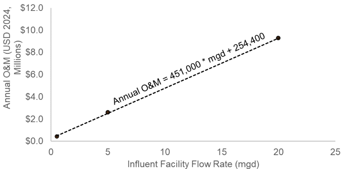
Figure 3-2. Annual Estimated O&M Cost Curve for GAC
