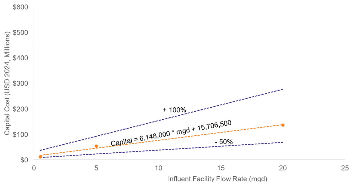
Figure 3-3. Project Capital Cost Curve with Estimating Range (-50% to +100%) for Installation of IX
