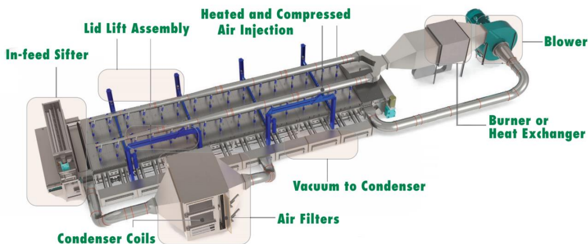
Figure D- 15. Representative Direct Dryer Model
