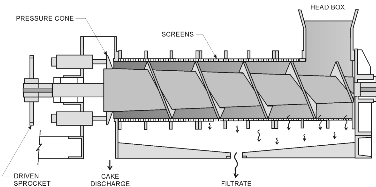
Figure D- 7. Configuration and Operation of a Typical Screw Press
