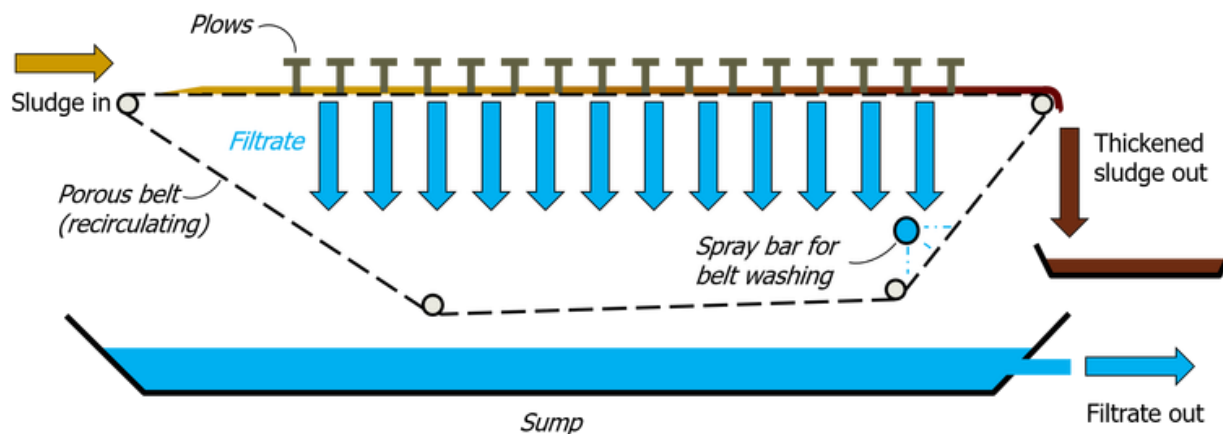
Figure D- 3. Gravity Belt Thickening (Courtesy of Judd Water & Wastewater Consultants)
