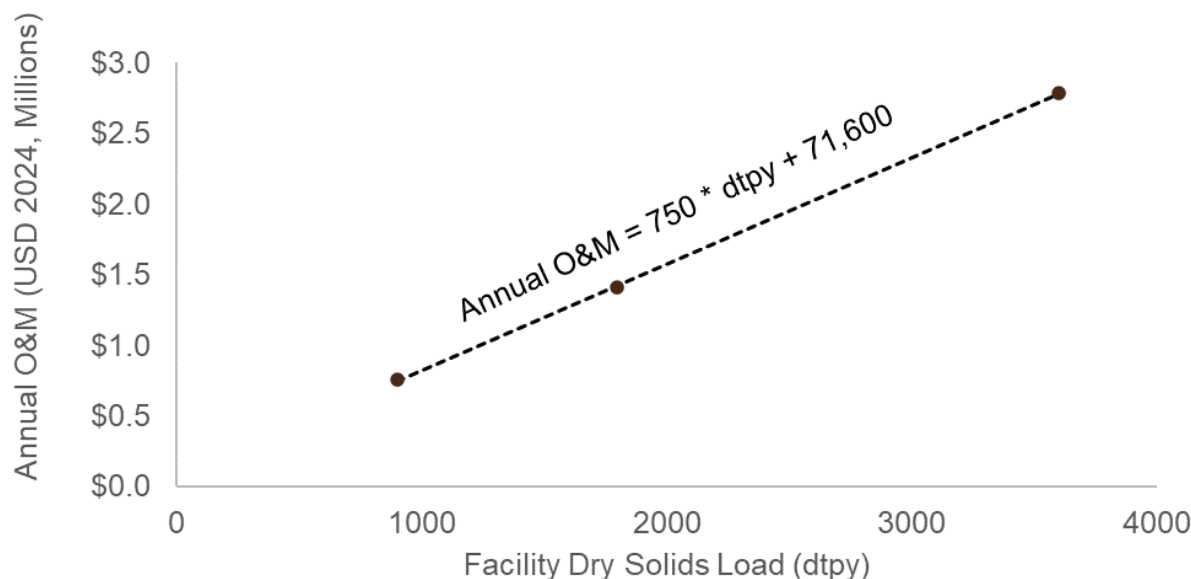
Figure 3-23. Annual Estimated O&M Cost Curve of SCWO Systems
