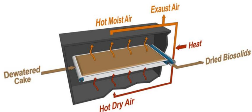
Figure D- 12 Representative Belt Dryer Operation Schematic
