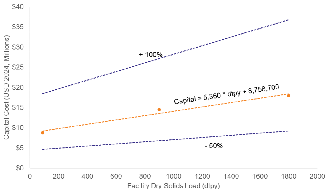
Figure 3-10. Project Capital Cost Curve with Estimating Range (-50% to +100%) for Installation of Centrifuges
