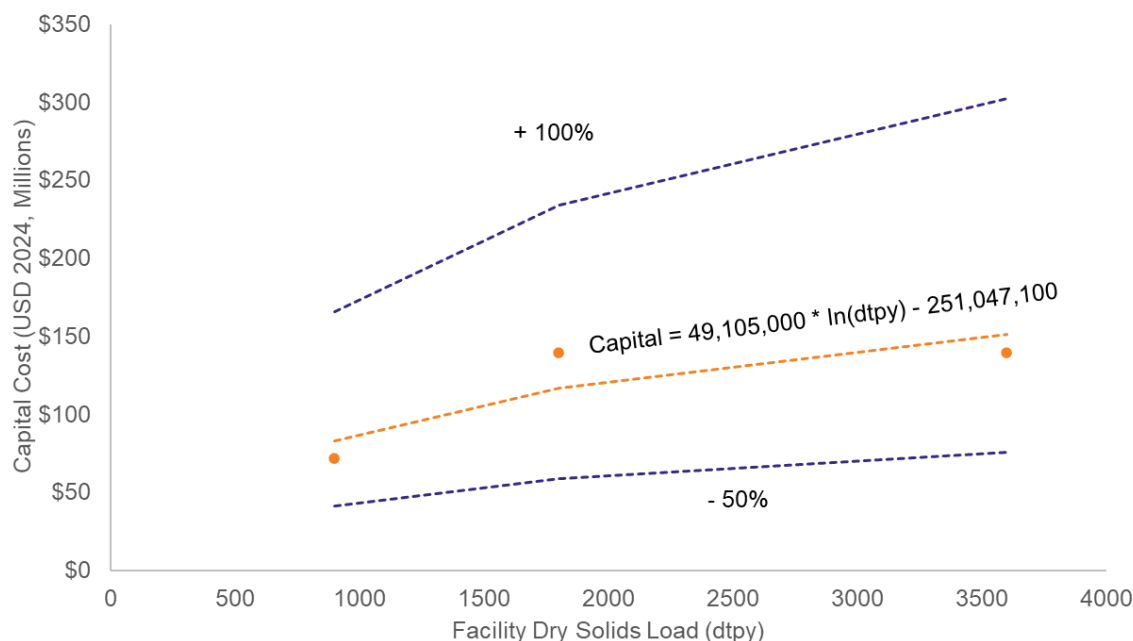
Figure 3-16. Project Capital Cost Curve with Estimating Range (-50% to +100%) for Installation of Rotary Drum Dryers
