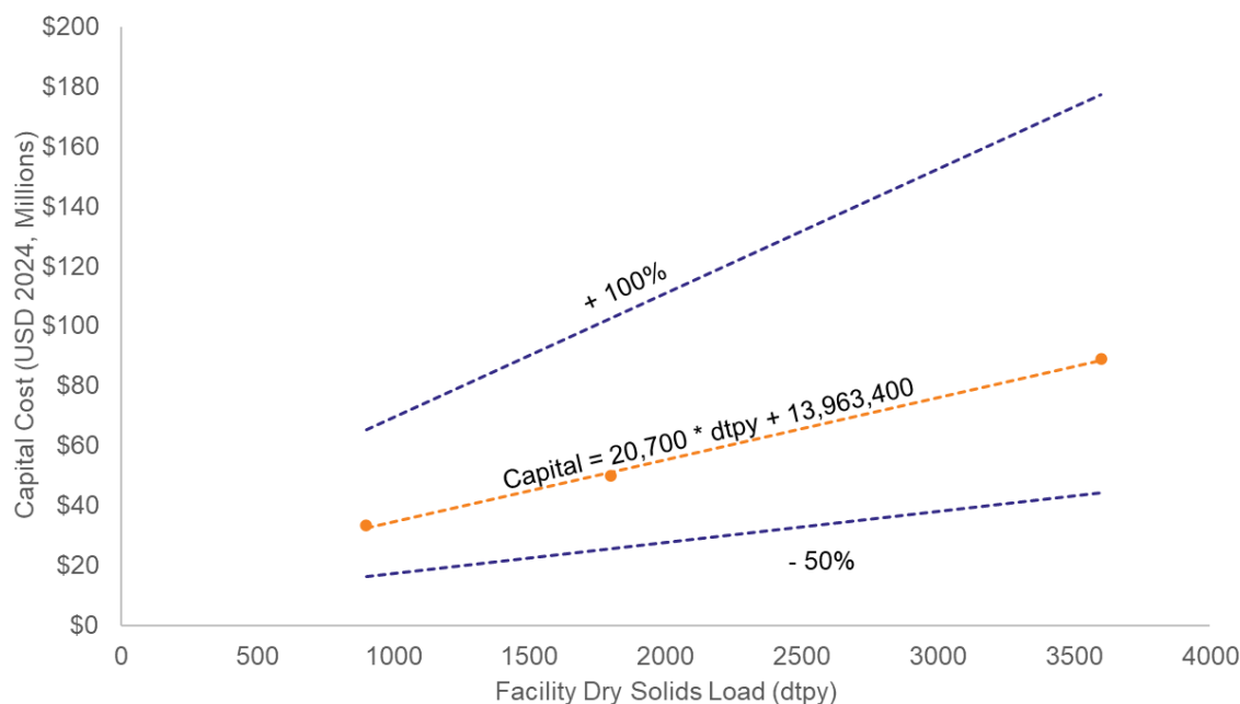
Figure 3-12. Project Capital Cost Curve with Estimating Range (-50% to +100%) for Installation of Mesophilic Anaerobic Digestion
