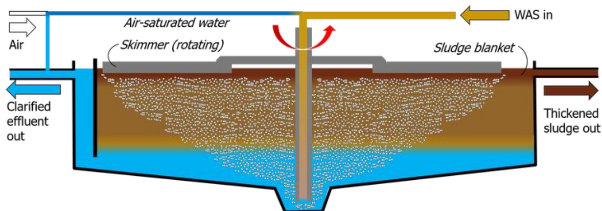
Figure D- 2.- Dissolved Air Flotation (Courtesy of Judd Water & Wastewater Consultants)
