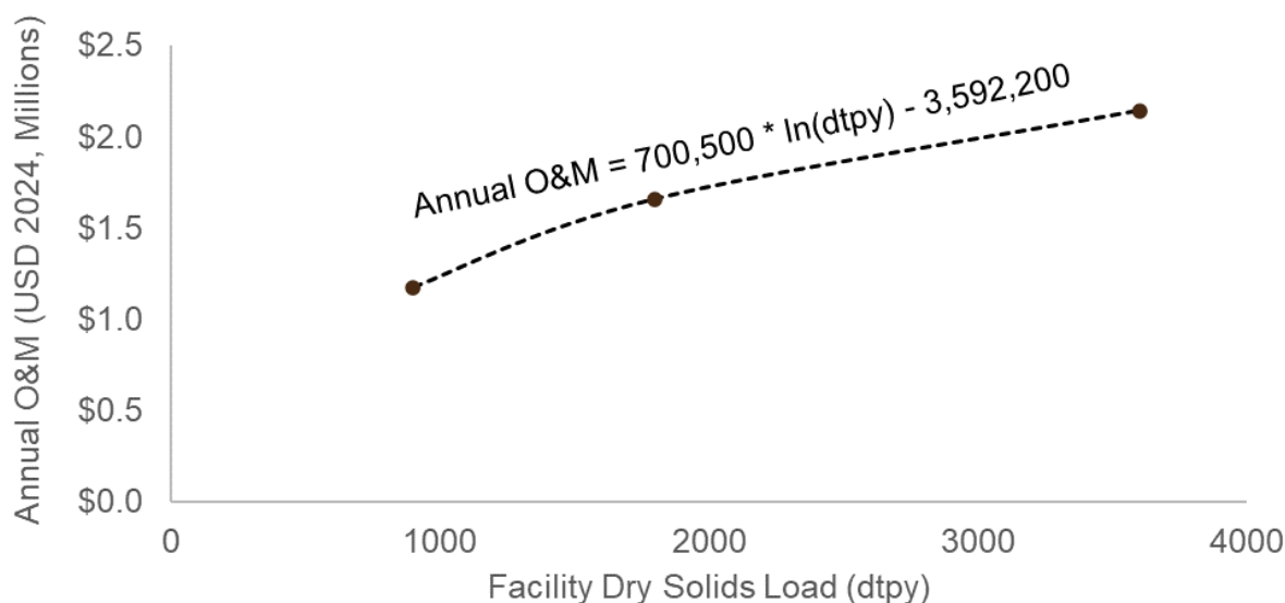
Figure 3-19. Annual Estimated O&M Cost Curve of Gasification Systems
