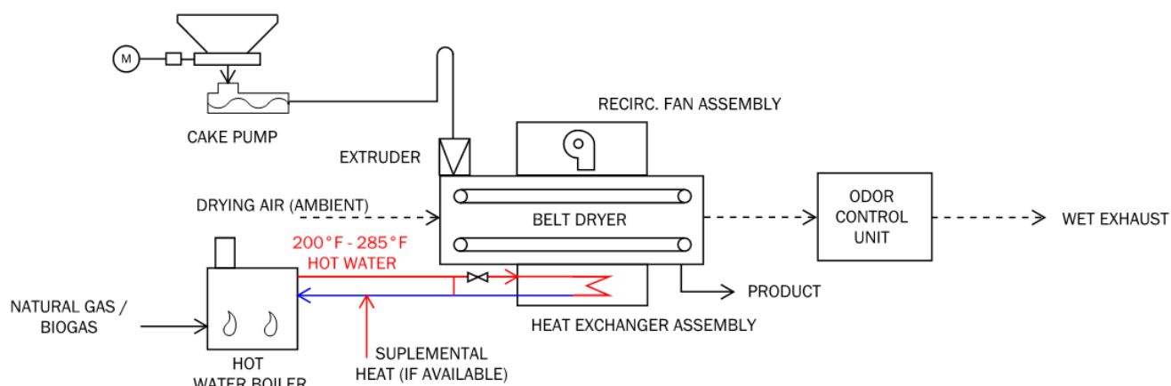
Figure D- 16. Representative Indirect-Fired Belt Dryer Operation Schematic
