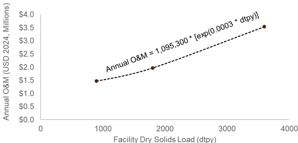
Figure 3-17. Annual Estimated O&M Cost Curve of Rotary Drum Dryers
