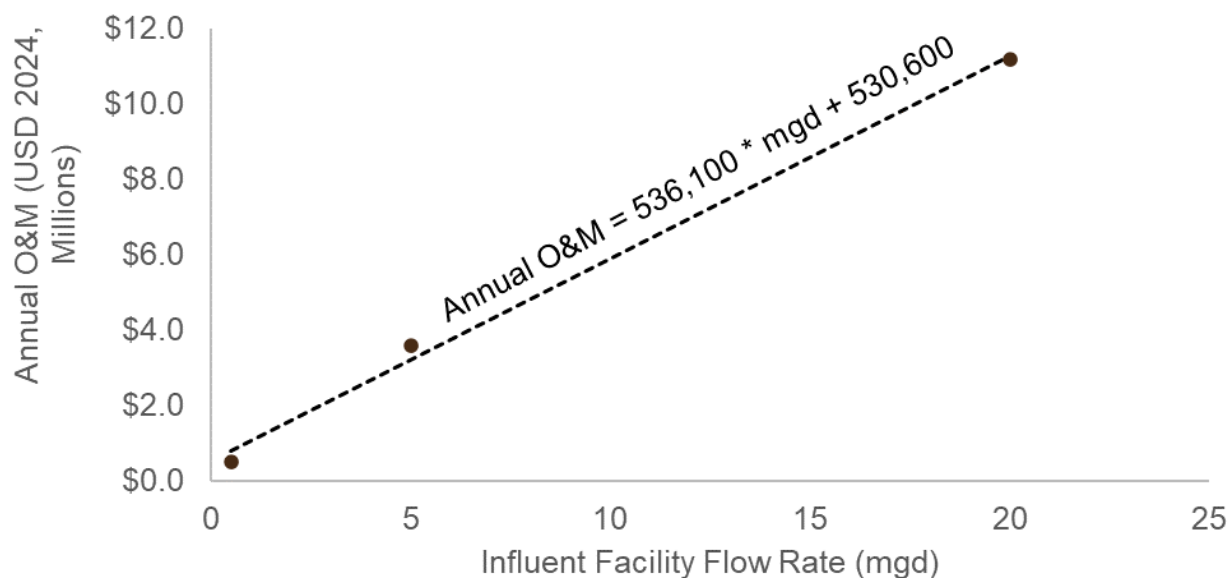
Figure 3-6. Annual Estimated O&M Cost Curve of GAC+IX
