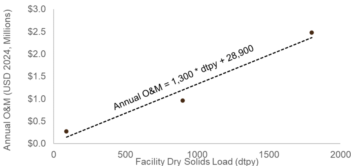
Figure 3-11. Annual Estimated O&M Cost Curve of Centrifuges
