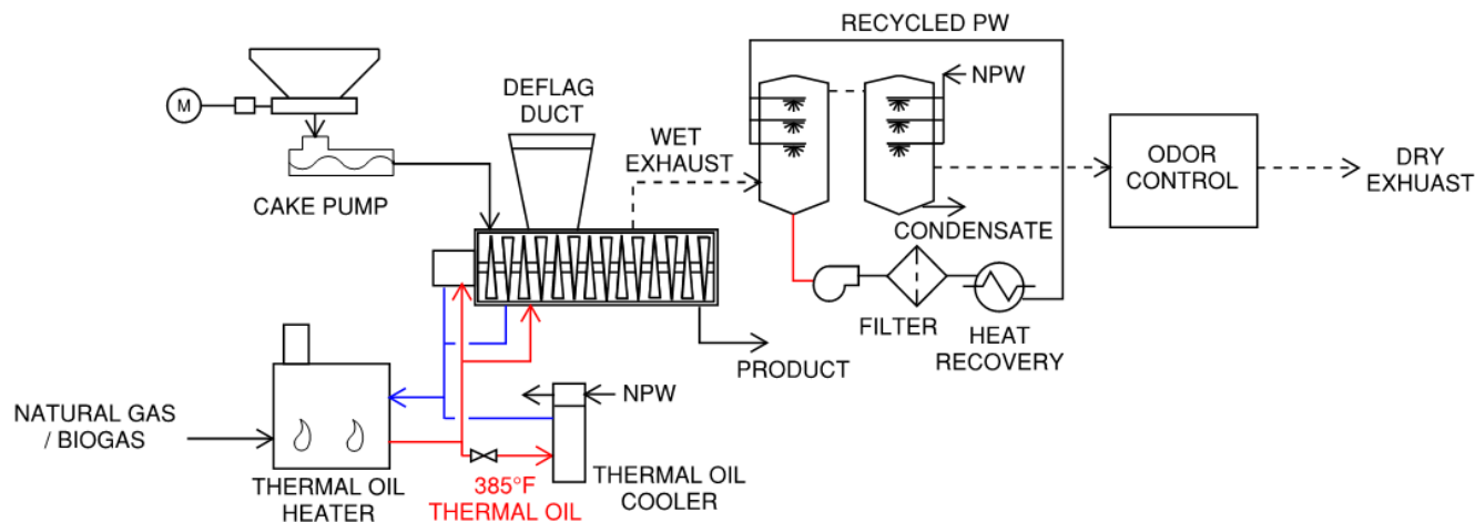
Figure D- 22. Representative Indirect, Paddle Dryer Operation Schematic
