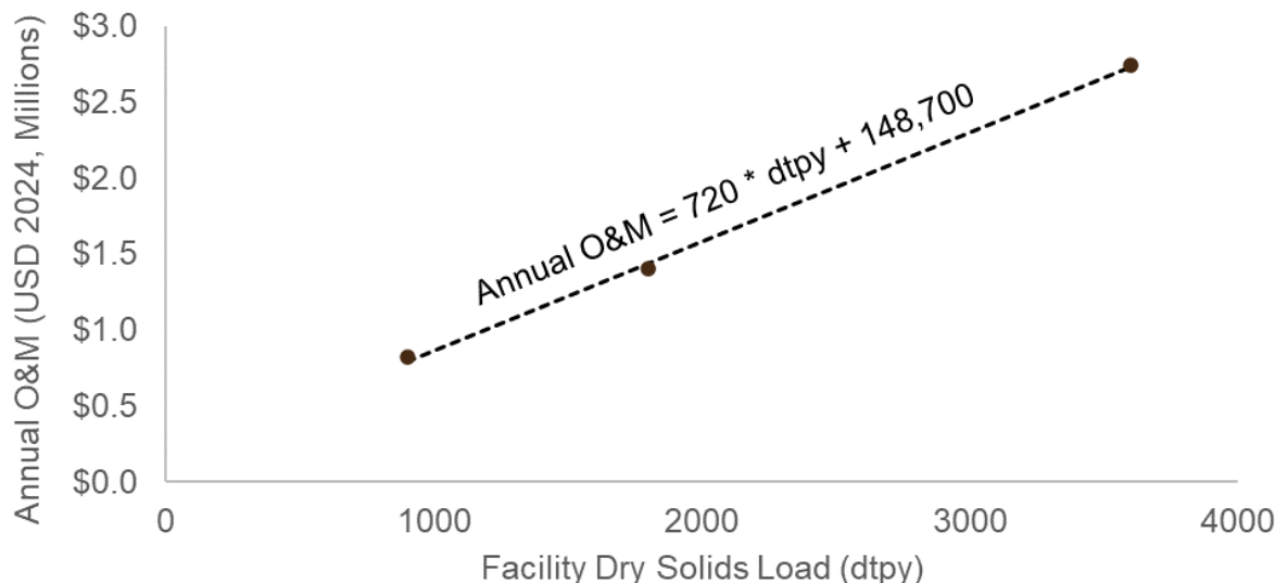
Figure 3-13. Annual Estimated O&M Cost Curve of Mesophilic Anaerobic Digestion
