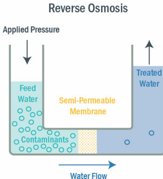
Figure B- 3. RO and NF are separation processes that retain contaminants like PFAS and allow water to permeate through the membrane
