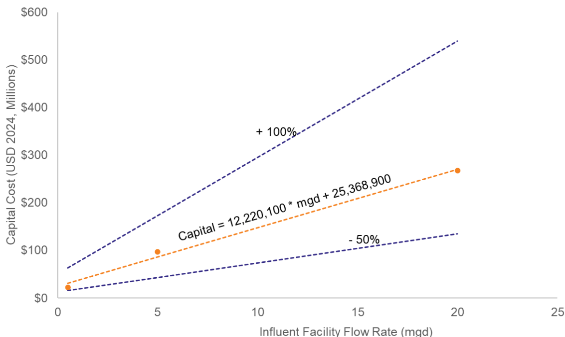
Figure 3-5. Project Capital Cost Curve with Estimating Range (-50% to +100%) for Installation of GAC+IX
