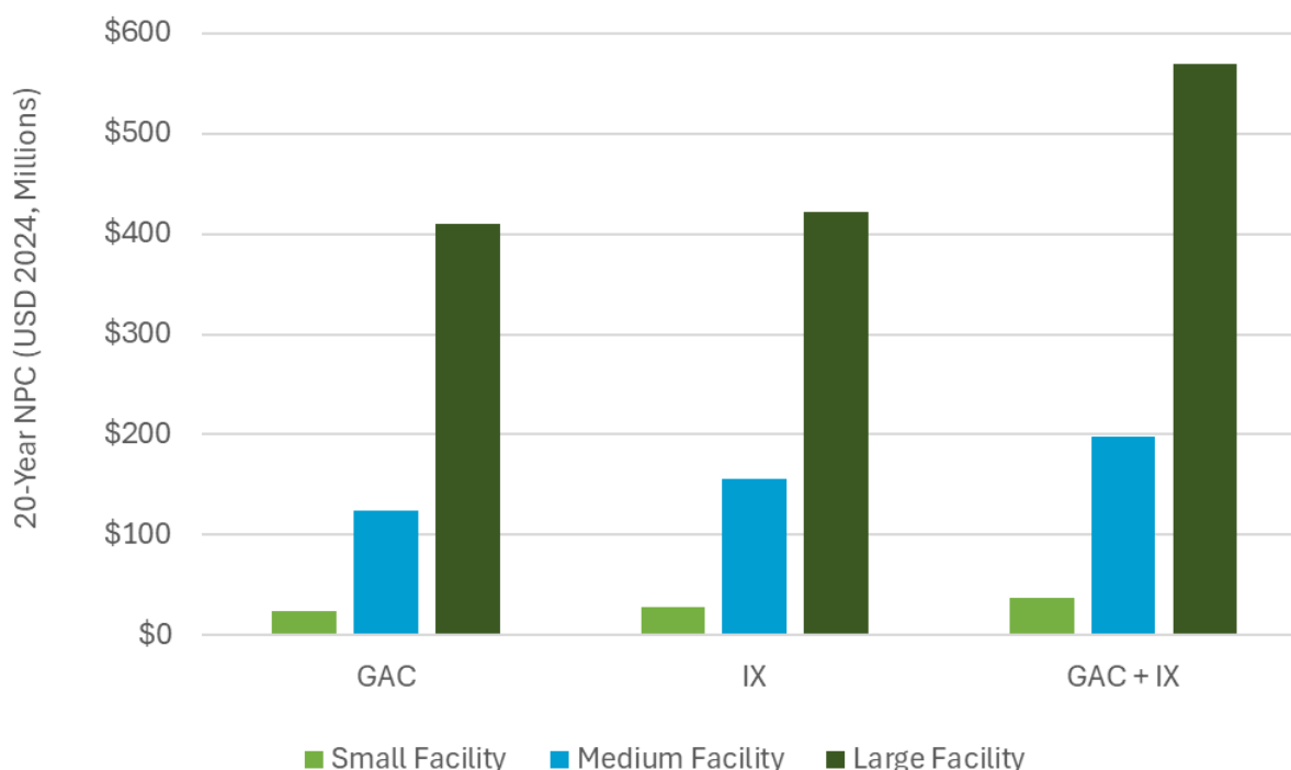
Figure 3-7. A Summary of the 20-Year NPC for Liquid Fraction of Wastewater PFAS Mitigation Technologies
