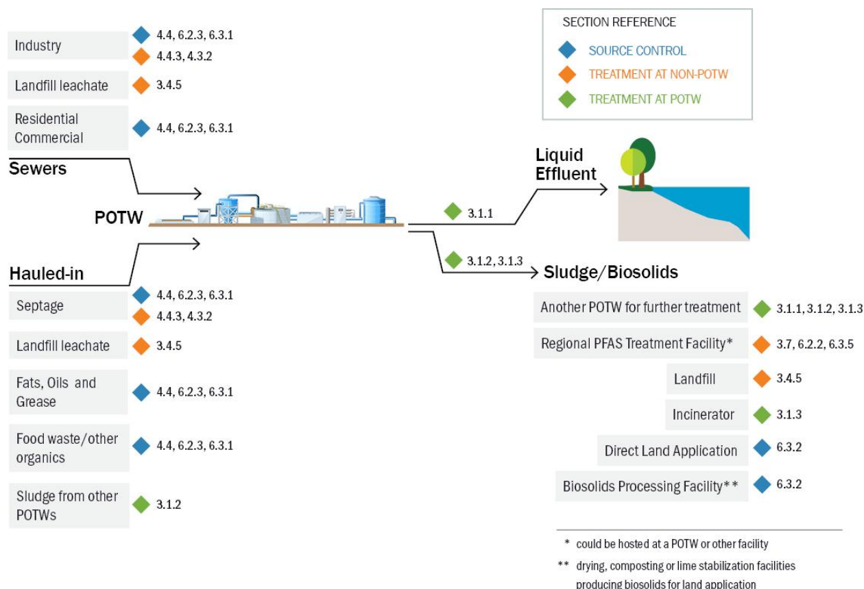
Figure ES-1. PFAS flows into and out of a POTW with control points (and report section numbers)
