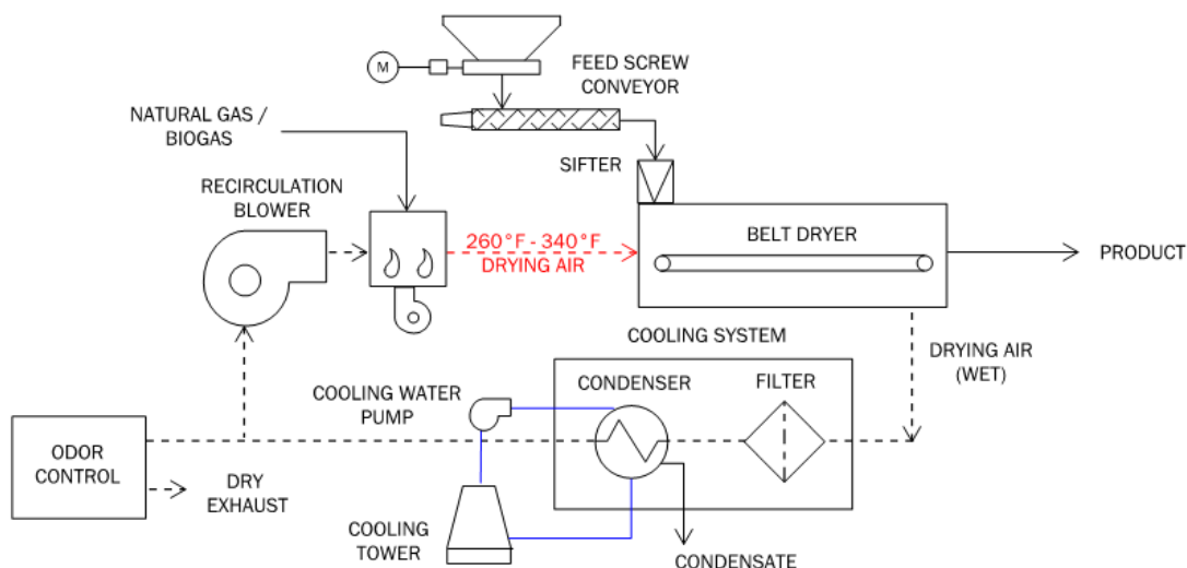
Figure D- 14. Representative direct-fired belt dryer operation schematic
