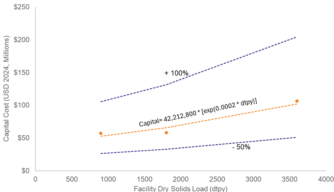
Figure 3-22. Project Capital Cost Curve with Estimating Range (-50% to +100%) for Installation of SCWO Systems
