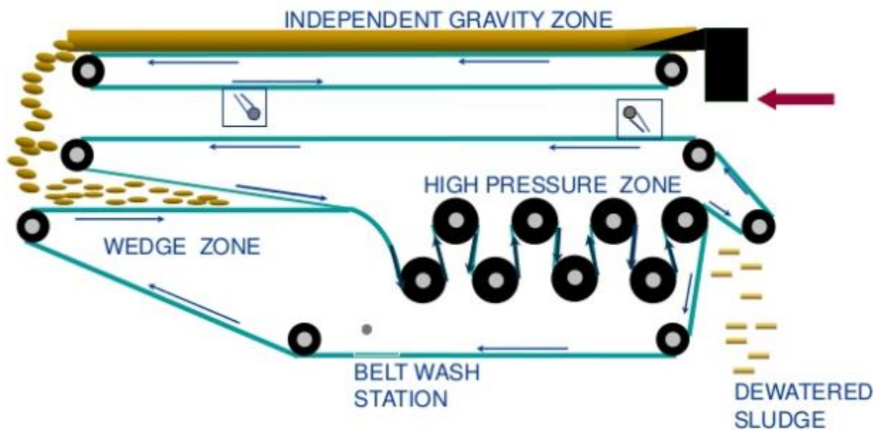
Figure D- 10. Belt Filter Press Cross-Section
