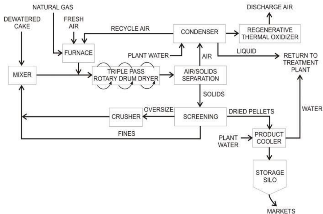
Figure D- 23. Representative Rotary Drum Dryer Operation Schematic
