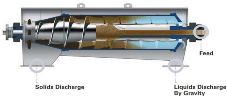
Figure D- 5. Centrifuge Cross-Section
