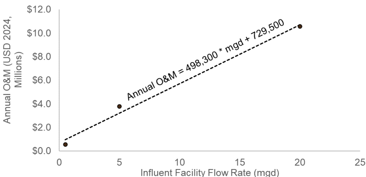
Figure 3-4. Annual Estimated O&M Cost Curve For IX
