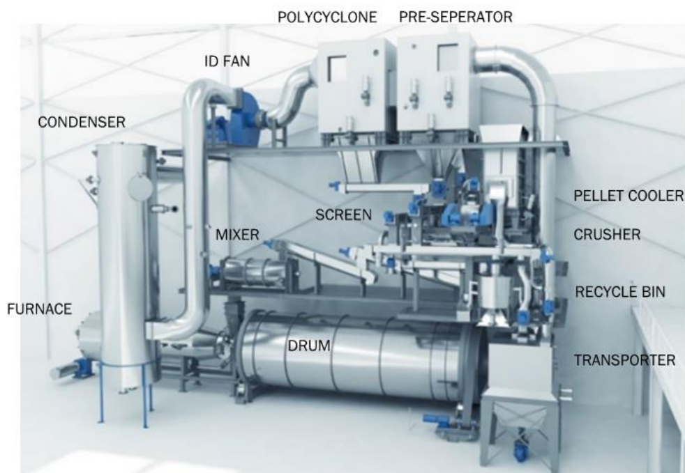
Figure D- 24. Representative Rotary Drum Dryer Model
