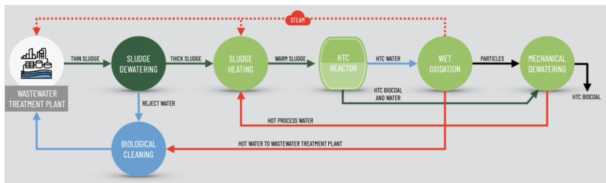
Figure C- 2. Process flow for OxyPower HTC
