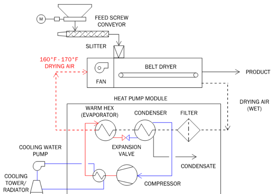
Figure D- 19. Representative Heat Pump Belt Dryer Operation Schematic
