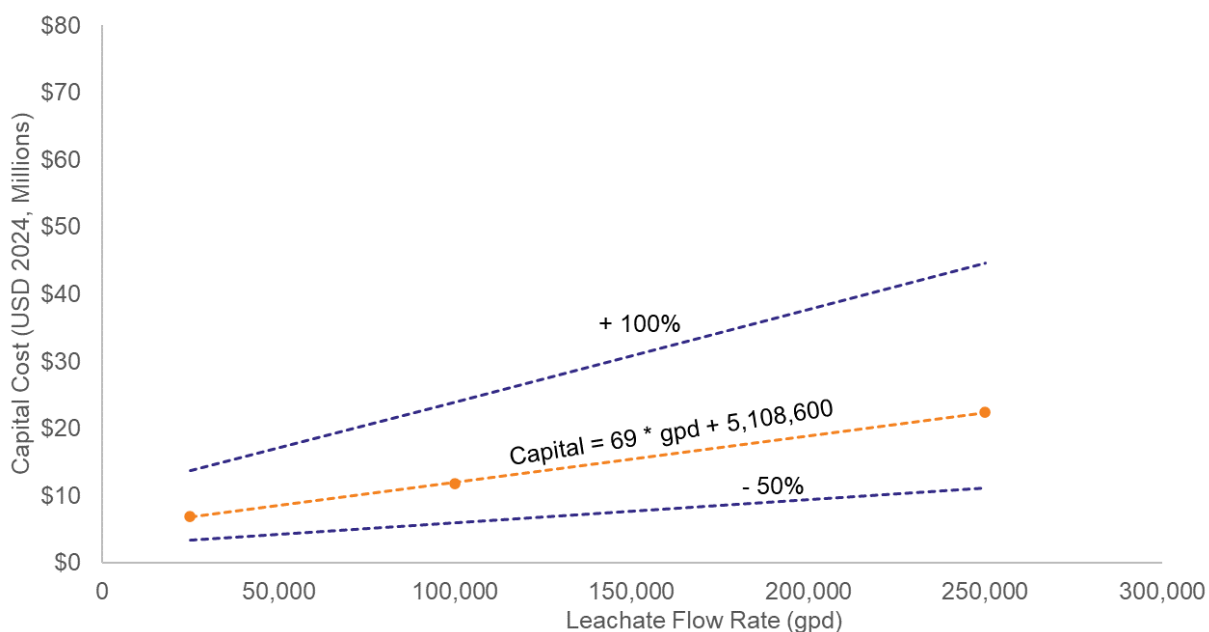
Figure 3-27. Project Capital Cost Curve with Estimating Range (-50% to +100%) for Installation of Foam Fractionation
