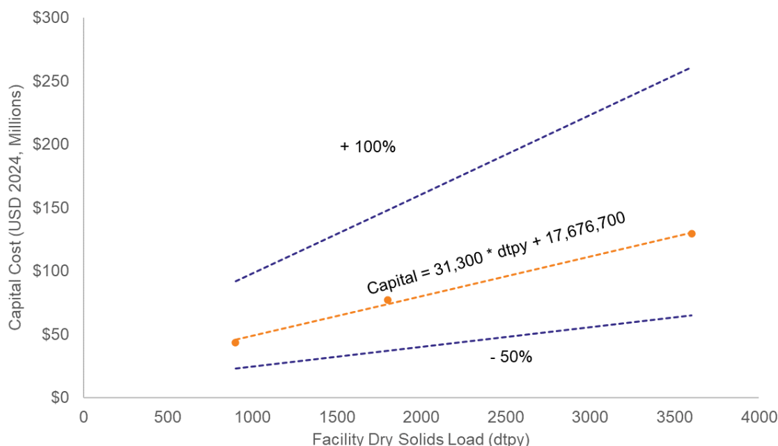
Figure 3-20. Project Capital Cost Curve with Estimating Range (-50% to +100%) for Installation of Pyrolysis Systems
