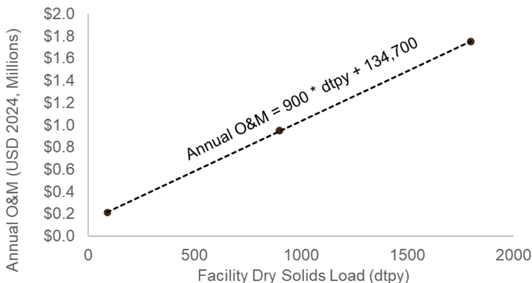
Figure 3-9. Annual Estimated O&M Cost Curve of Screw Presses
