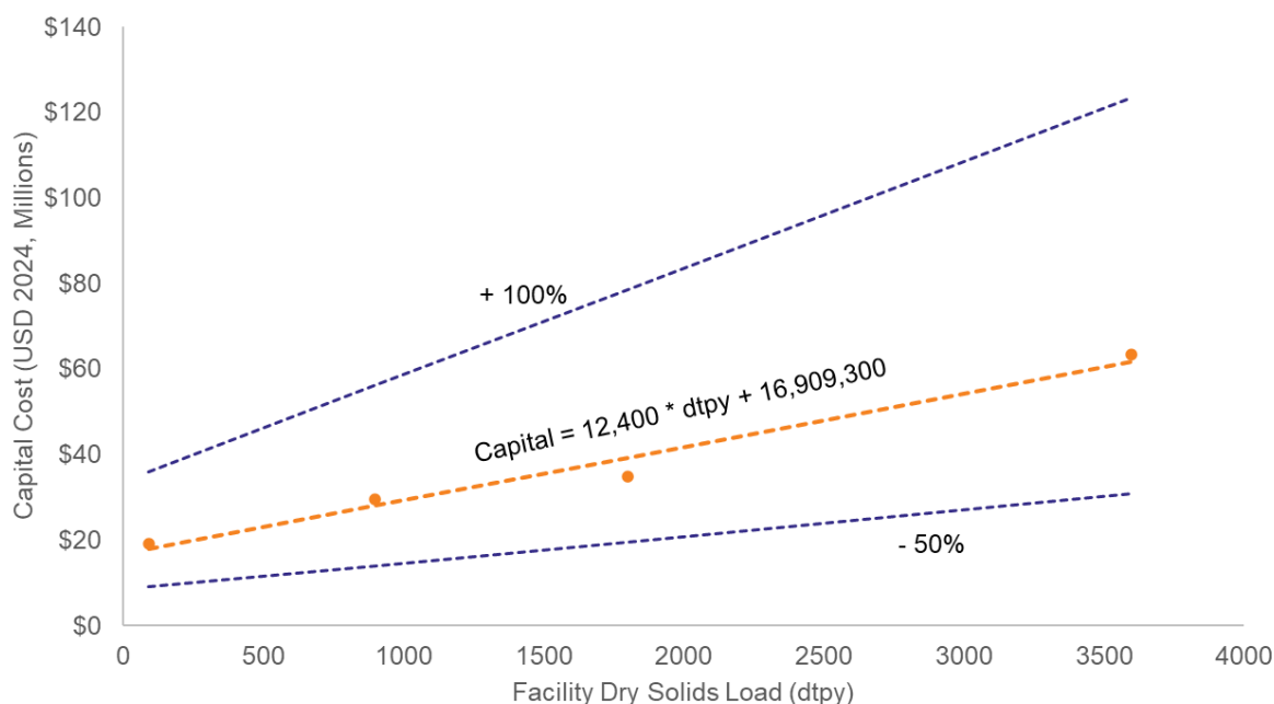
Figure 3-14. Project Capital Cost Curve with Estimating Range (-50% to +100%) for Installation of Belt Dryers
