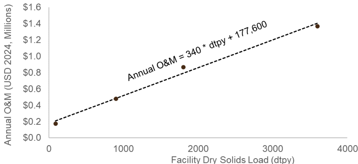
Figure 3-15. Annual Estimated O&M Cost Curve of Belt Dryers
