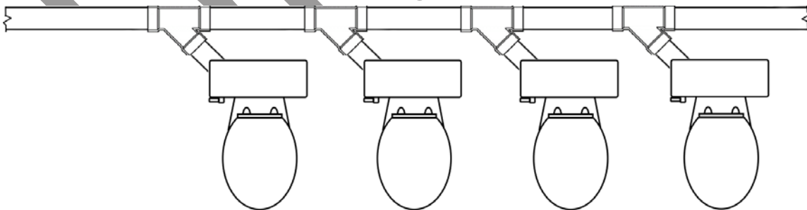
10.03: Example 1 - Battery of Fixtures
