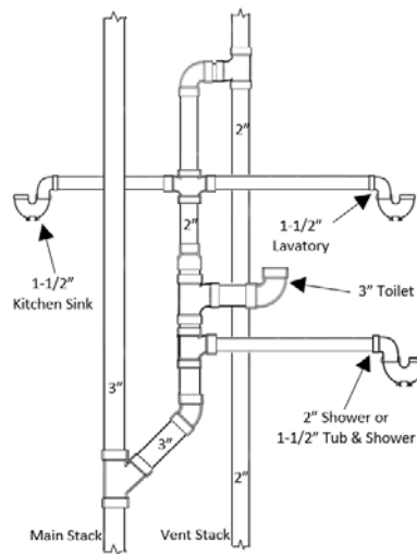
Stack Venting Lower Floors
