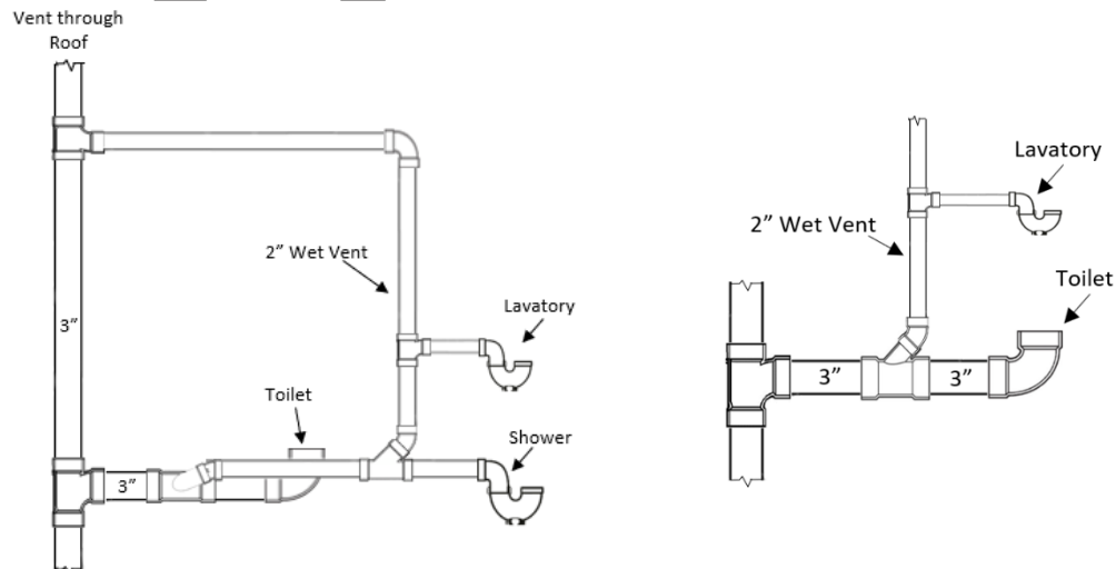
Example 10 - Miscellaneous Wet Venting
