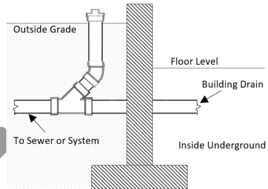
10.08: Example 9 Building Drain Cleanout Installed Outside
