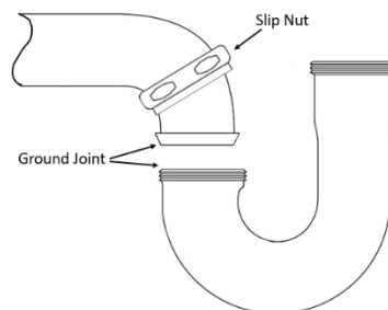
10.07: Example 2 - Ground Joint
