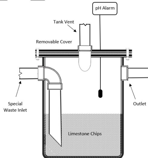
10.13: Example 2 - Chip Tank
