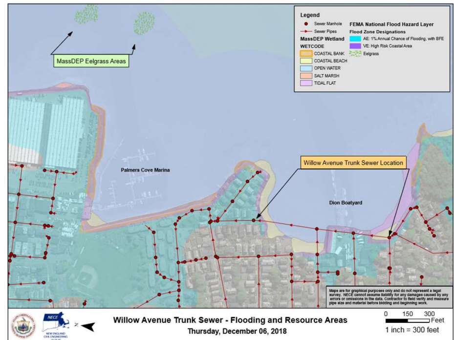
Current conditions map demonstrating the location of the existing trunk sewer
