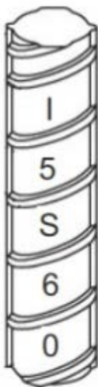
#5 Bar 60 Grade
